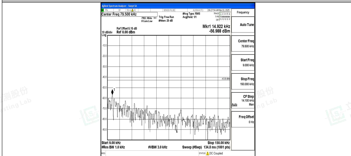
Band66_20MHz_QPSK_132572_1RB#0_0.009~0.15_0.009~0.15
