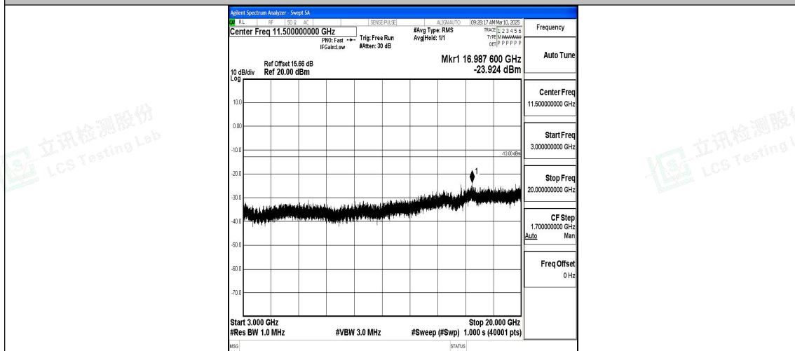
Band66_20MHz_QPSK_132572_1RB#0_3000~20000_3000~20000
