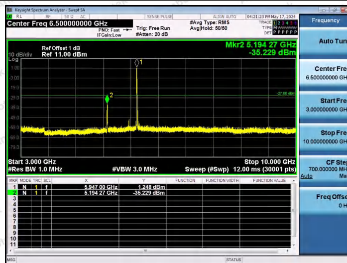
11AX20SISO-Ant1-5955-26Tone-RU0-3000~10000-PASS
