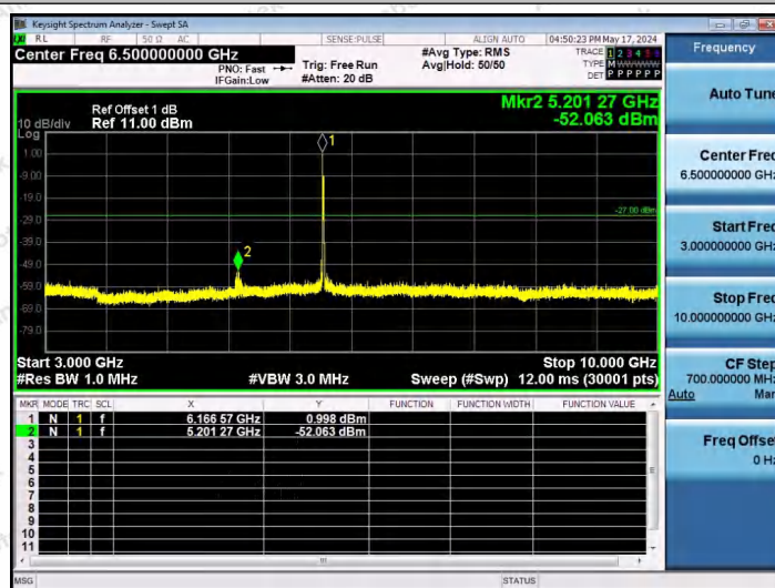
11AX20SISO-Ant1-6175-26Tone-RU0-3000~10000-PASS
