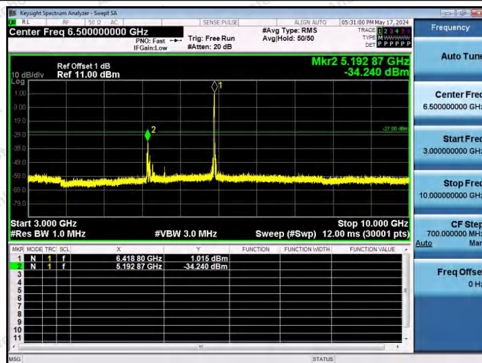
11AX20SISO-Ant1-6415-52Tone-RU39-3000~10000-PASS
