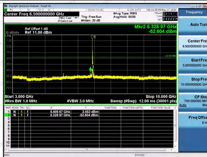
11AX20SISO-Ant1-6415-26Tone-RU0-3000~10000-PASS
