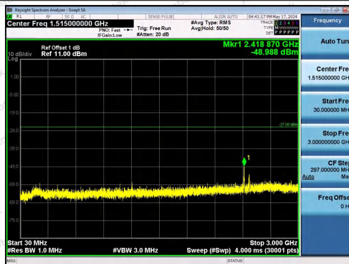
11AX20SISO-Ant1-5955-52Tone-RU40-30~3000-PASS
