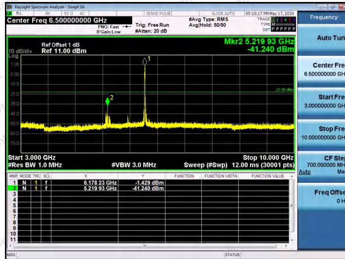
11AX20SISO-Ant1-6175-106Tone-RU54-3000~10000-PASS
