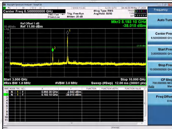
11AX20SISO-Ant1-5955-106Tone-RU54-3000~10000-PASS
