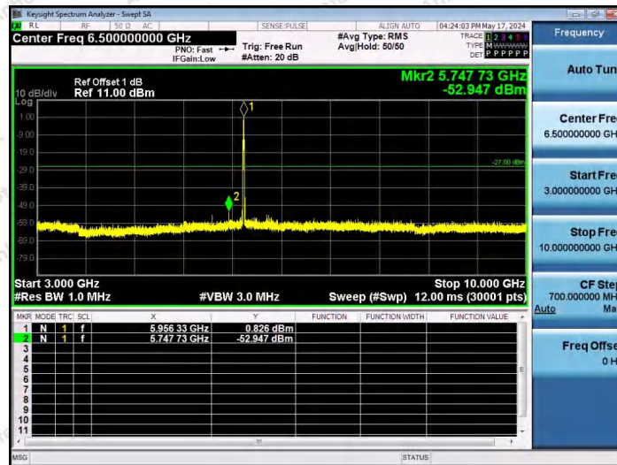
11AX20SISO-Ant1-5955-26Tone-RU4-3000~10000-PASS
