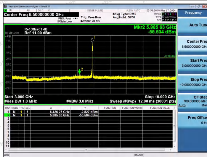
11AX20SISO-Ant1-6435-106Tone-RU53-3000~10000-PASS
