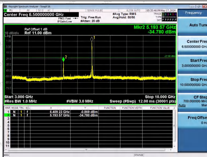
11AX20SISO-Ant1-6415-106Tone-RU53-3000~10000-PASS
