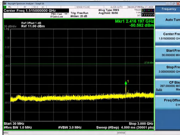
11AX20SISO-Ant1-6475-26Tone-RU0-30~3000-PASS
