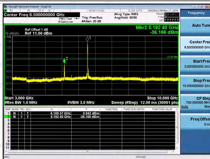
11AX20SISO-Ant1-6175-52Tone-RU37-3000~10000-PASS
