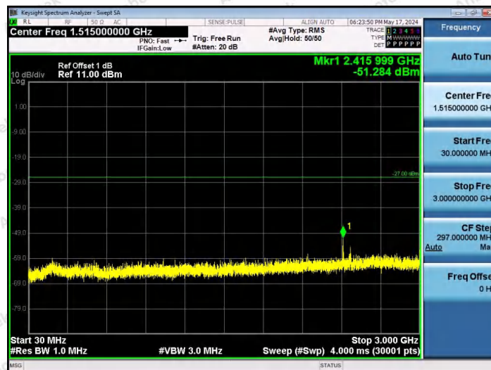
11AX20SISO-Ant1-6475-106Tone-RU54-30~3000-PASS
