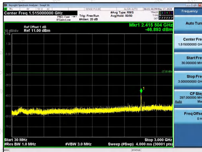
11AX20SISO-Ant1-6435-106Tone-RU54-30~3000-PASS
