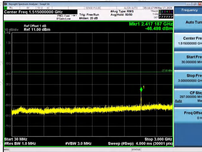
11AX20SISO-Ant1-6415-26Tone-RU0-30~3000-PASS
