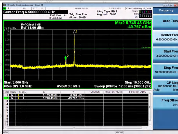
11AX20SISO-Ant1-6175-52Tone-RU40-3000~10000-PASS
