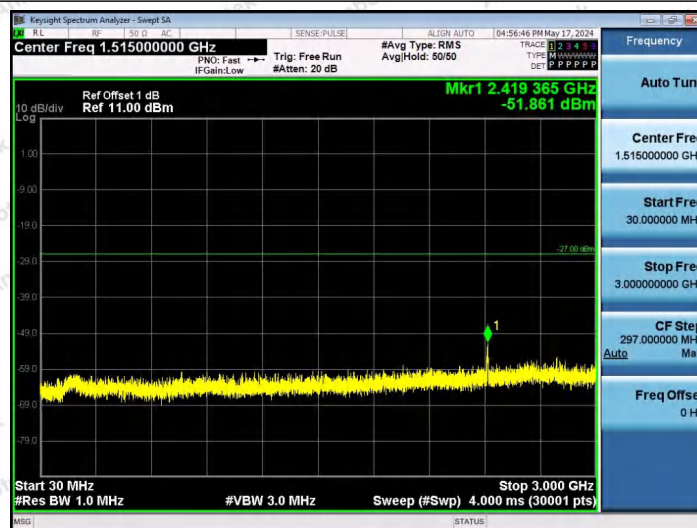
11AX20SISO-Ant1-6175-26Tone-RU8-30~3000-PASS
