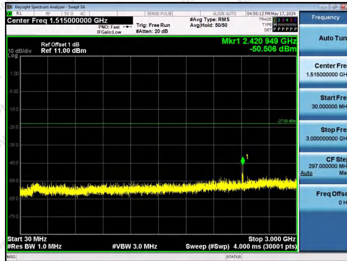
11AX20SISO-Ant1-6175-26Tone-RU0-30~3000-PASS
