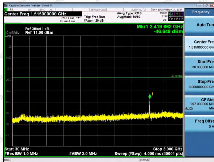
11AX20SISO-Ant1-5955-106Tone-RU54-30~3000-PASS
