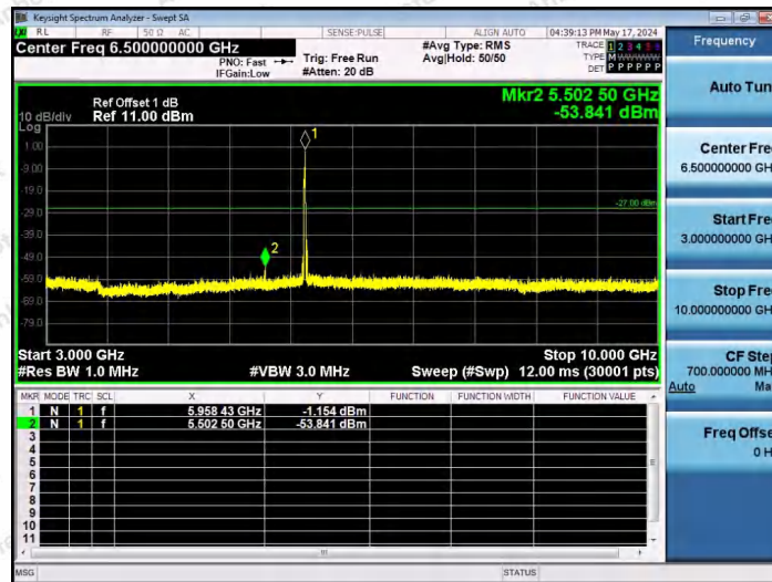
11AX20SISO-Ant1-5955-52Tone-RU39-3000~10000-PASS
