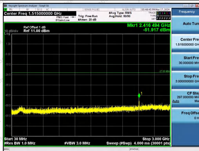
11AX20SISO-Ant1-6435-26Tone-RU8-30~3000-PASS
