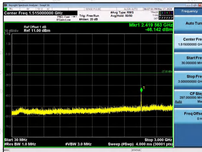
11AX20SISO-Ant1-6475-26Tone-RU4-30~3000-PASS
