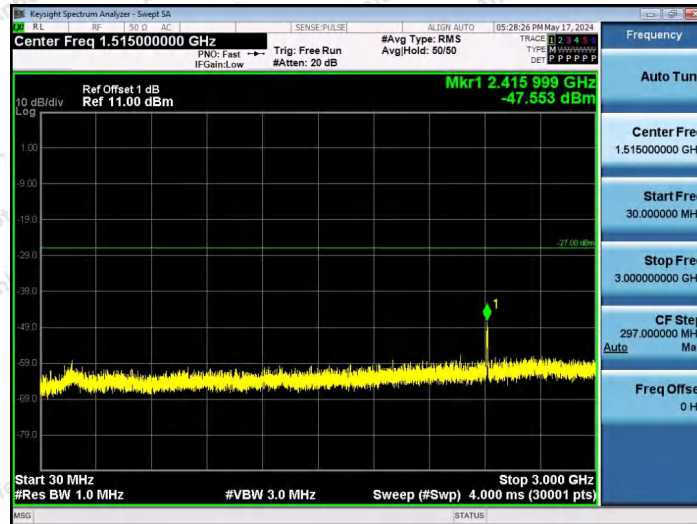
11AX20SISO-Ant1-6415-52Tone-RU37-30~3000-PASS
