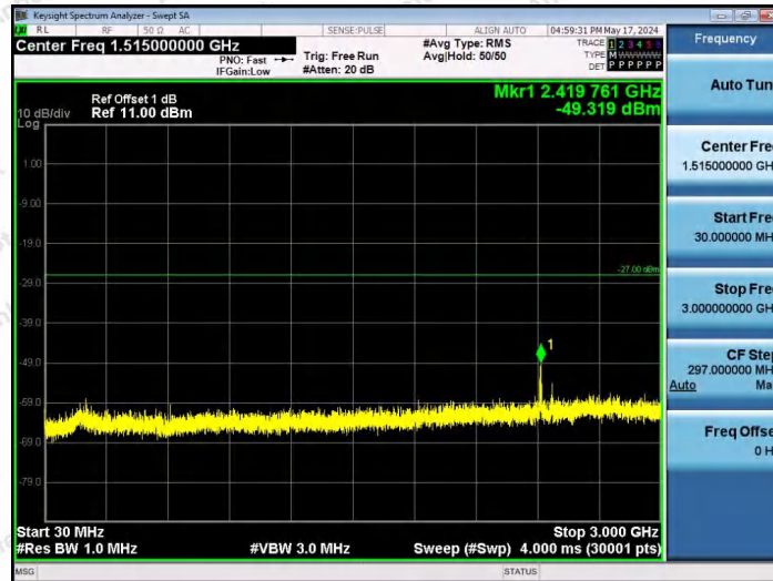
11AX20SISO-Ant1-6175-52Tone-RU37-30~3000-PASS
