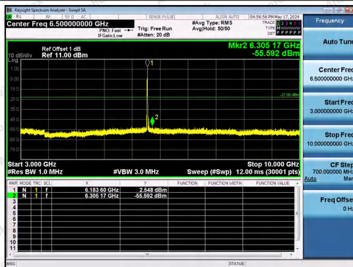
11AX20SISO-Ant1-6175-26Tone-RU8-3000~10000-PASS
