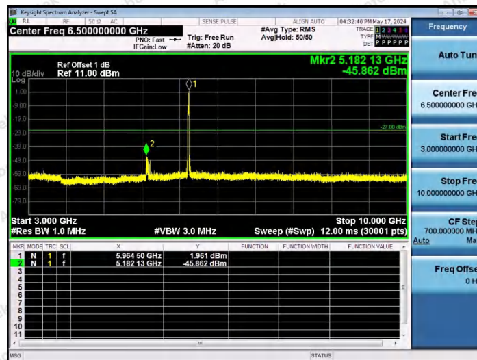
11AX20SISO-Ant1-5955-26Tone-RU8-3000~10000-PASS
