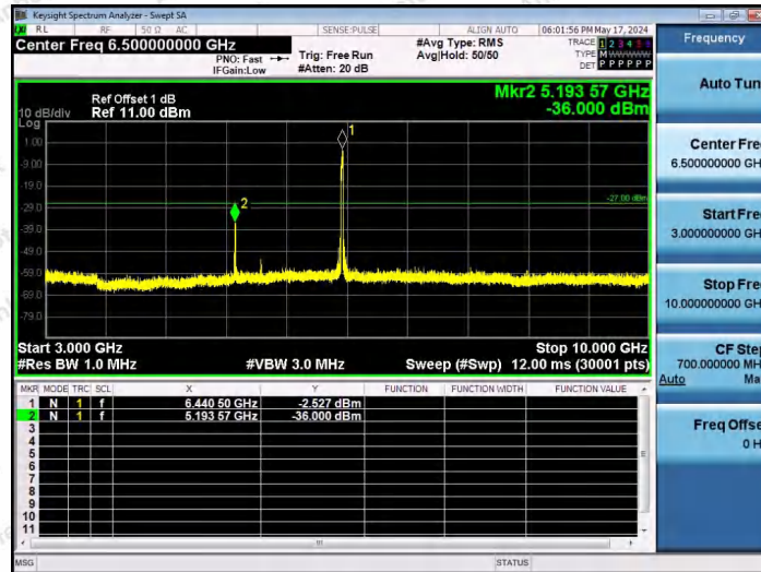
11AX20SISO-Ant1-6435-106Tone-RU54-3000~10000-PASS
