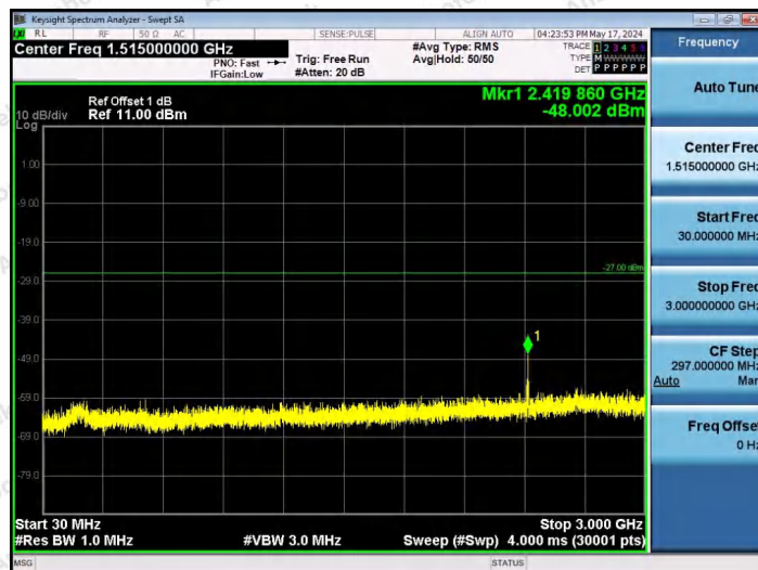
11AX20SISO-Ant1-5955-26Tone-RU4-30~3000-PASS
