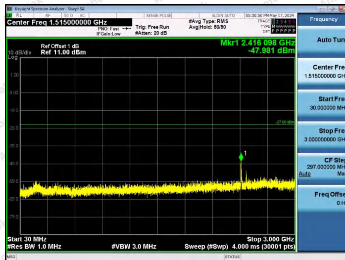
11AX20SISO-Ant1-6415-52Tone-RU39-30~3000-PASS
