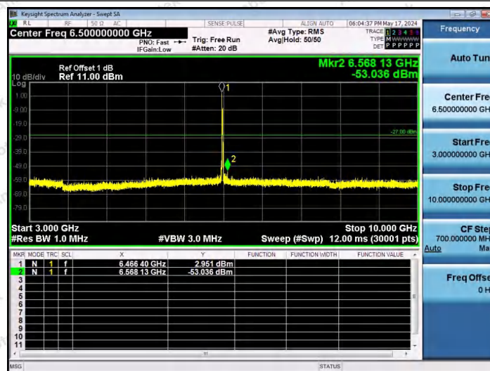
11AX20SISO-Ant1-6475-26Tone-RU0-3000~10000-PASS
