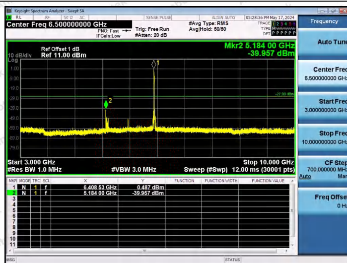
11AX20SISO-Ant1-6415-52Tone-RU37-3000~10000-PASS
