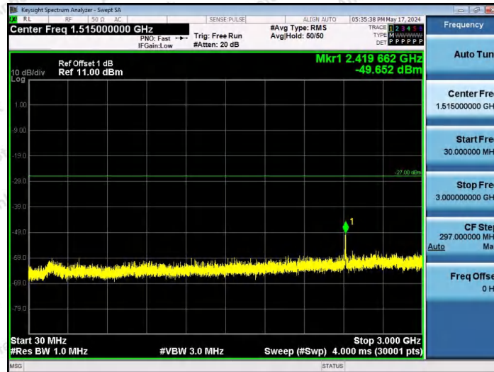
11AX20SISO-Ant1-6415-106Tone-RU53-30~3000-PASS
