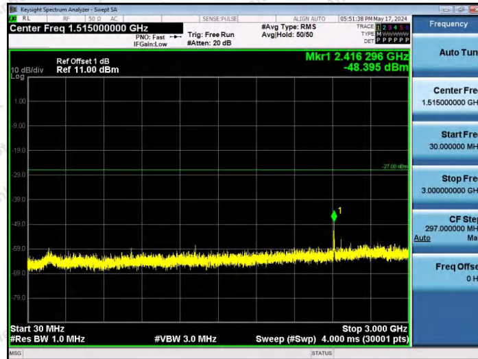
11AX20SISO-Ant1-6435-52Tone-RU37-30~3000-PASS
