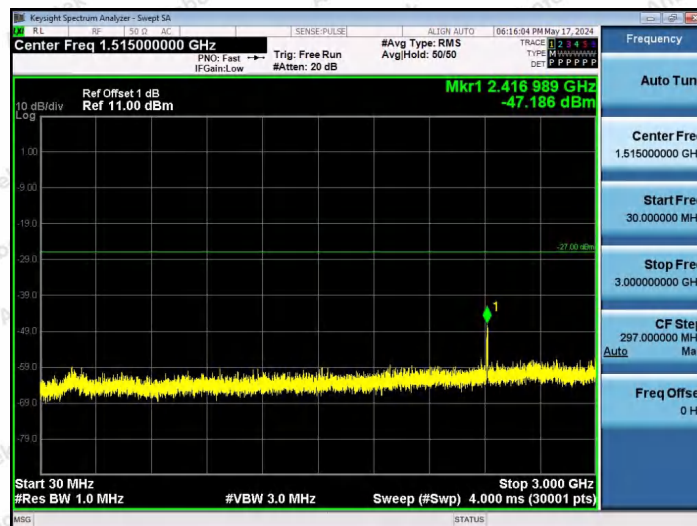
11AX20SISO-Ant1-6475-52Tone-RU39-30~3000-PASS
