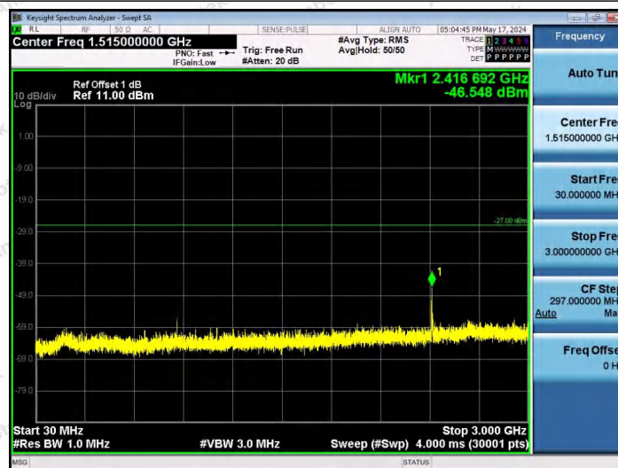
11AX20SISO-Ant1-6175-52Tone-RU40-30~3000-PASS
