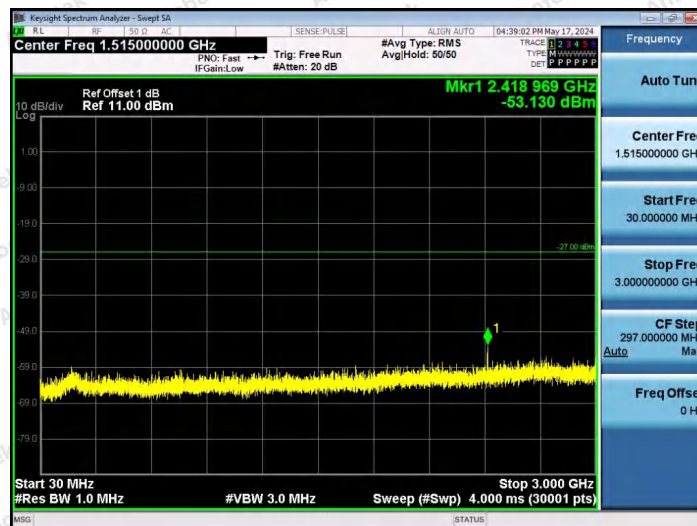
11AX20SISO-Ant1-5955-52Tone-RU39-30~3000-PASS
