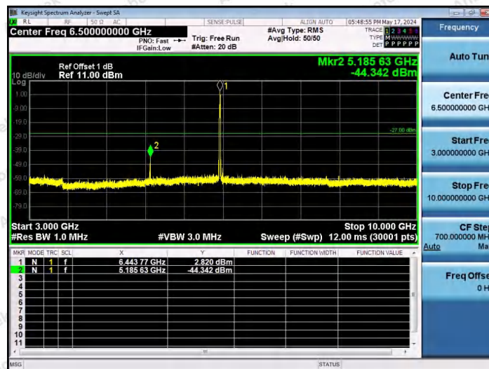
11AX20SISO-Ant1-6435-26Tone-RU8-3000~10000-PASS
