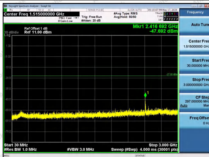
11AX20SISO-Ant1-6175-106Tone-RU54-30~3000-PASS
