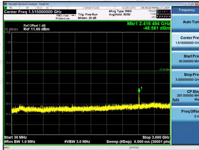
11AX20SISO-Ant1-6435-106Tone-RU53-30~3000-PASS
