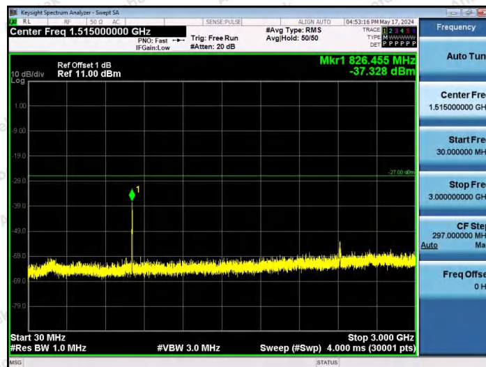
11AX20SISO-Ant1-6175-26Tone-RU4-30~3000-PASS
