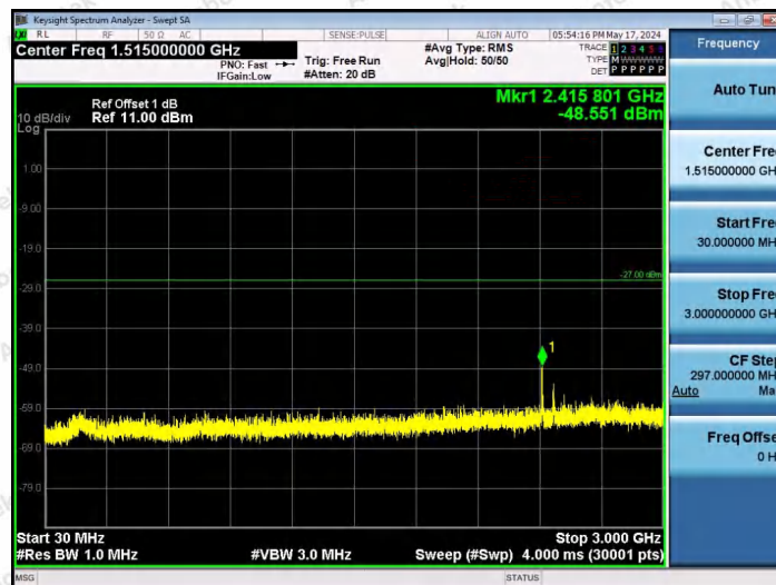
11AX20SISO-Ant1-6435-52Tone-RU39-30~3000-PASS
