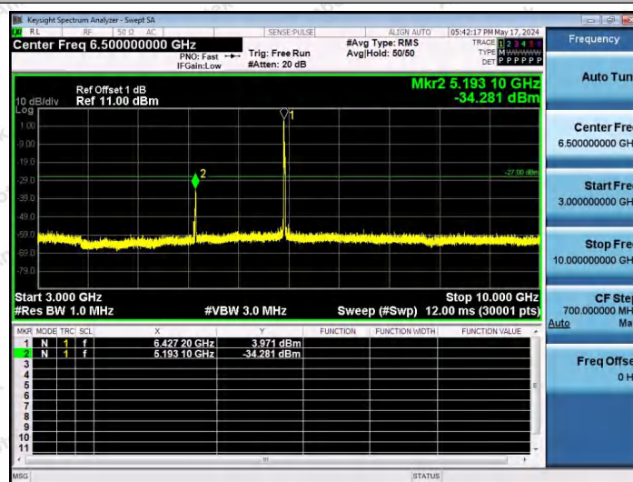
11AX20SISO-Ant1-6435-26Tone-RU0-3000~10000-PASS
