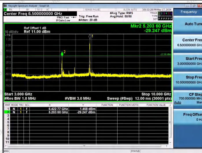
11AX20SISO-Ant1-6415-52Tone-RU40-3000~10000-PASS
