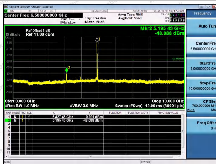
11AX20SISO-Ant1-6435-52Tone-RU37-3000~10000-PASS
