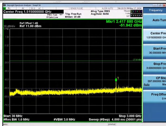
11AX20SISO-Ant1-6475-26Tone-RU8-30~3000-PASS
