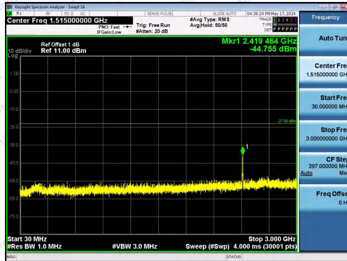
11AX20SISO-Ant1-5955-52Tone-RU37-30~3000-PASS
