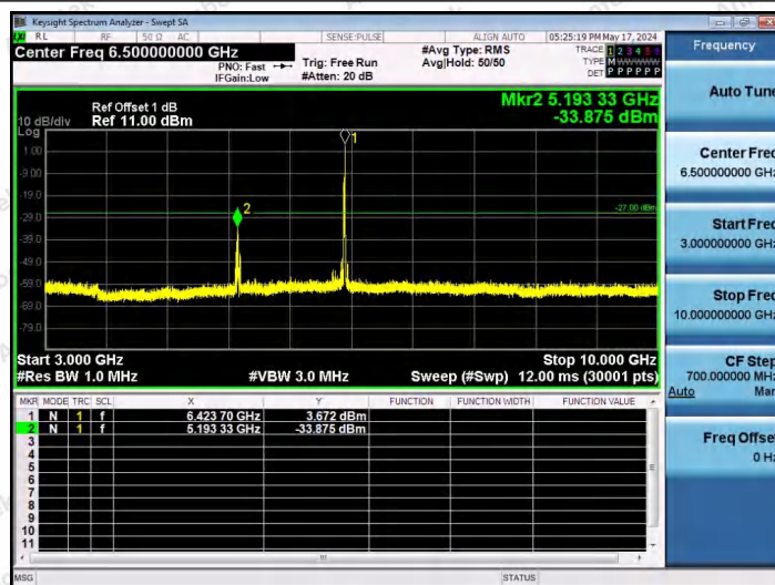
11AX20SISO-Ant1-6415-26Tone-RU8-3000~10000-PASS
