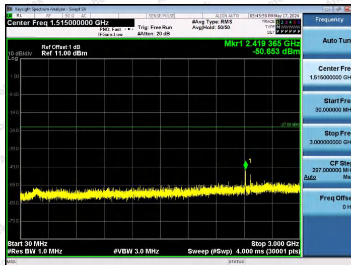
11AX20SISO-Ant1-6435-26Tone-RU4-30~3000-PASS
