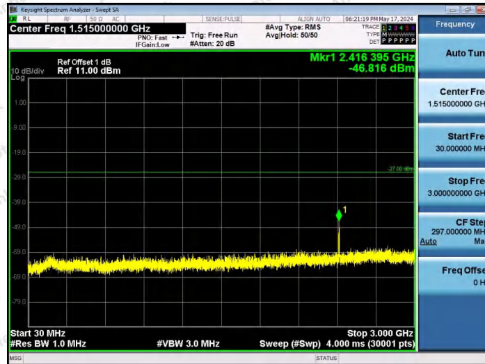
11AX20SISO-Ant1-6475-106Tone-RU53-30~3000-PASS
