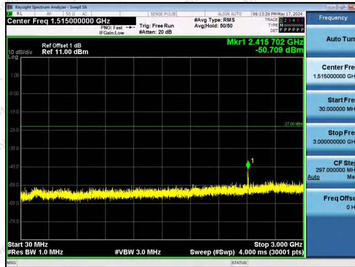
11AX20SISO-Ant1-6475-52Tone-RU37-30~3000-PASS
