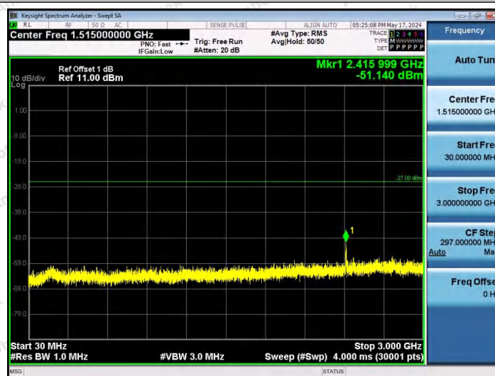
11AX20SISO-Ant1-6415-26Tone-RU8-30~3000-PASS
