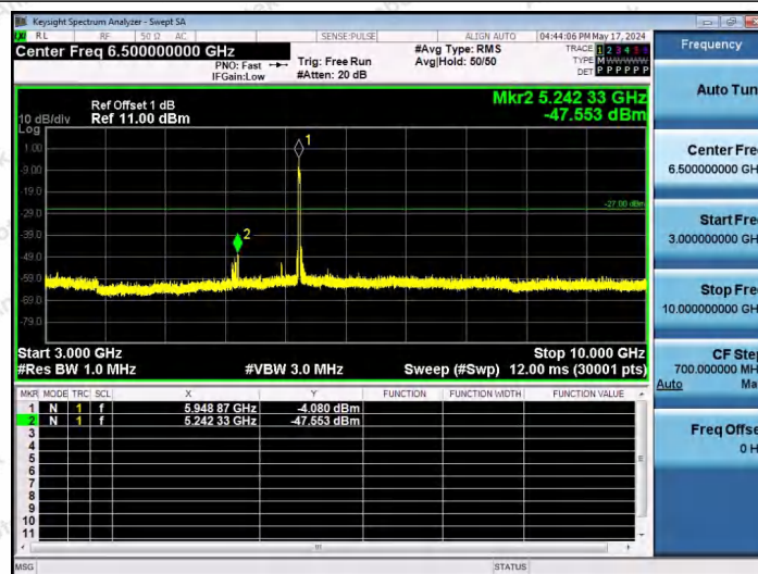
11AX20SISO-Ant1-5955-106Tone-RU53-3000~10000-PASS
