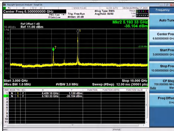
11AX20SISO-Ant1-6435-52Tone-RU39-3000~10000-PASS
