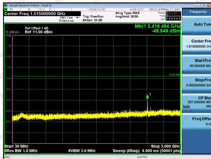
11AX20SISO-Ant1-6415-26Tone-RU4-30~3000-PASS
