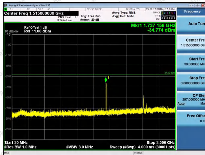
11AX20SISO-Ant1-6415-106Tone-RU54-30~3000-PASS
