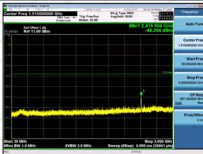
11AX20SISO-Ant1-5955-26Tone-RU8-30~3000-PASS
