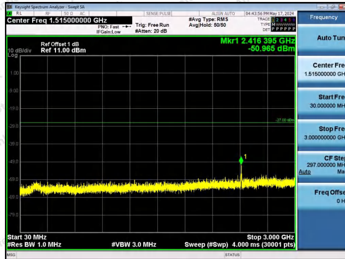
11AX20SISO-Ant1-5955-106Tone-RU53-30~3000-PASS
