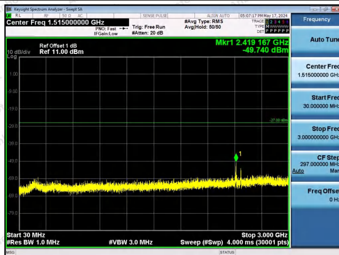
11AX20SISO-Ant1-6175-106Tone-RU53-30~3000-PASS
