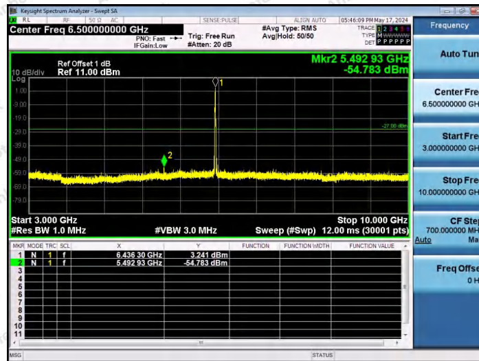
11AX20SISO-Ant1-6435-26Tone-RU4-3000~10000-PASS
