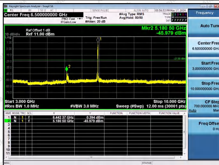
11AX20SISO-Ant1-6435-52Tone-RU40-3000~10000-PASS
