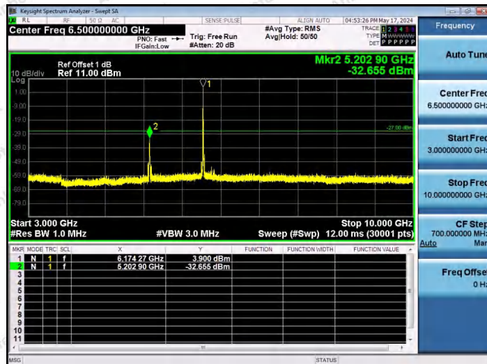
11AX20SISO-Ant1-6175-26Tone-RU4-3000~10000-PASS
