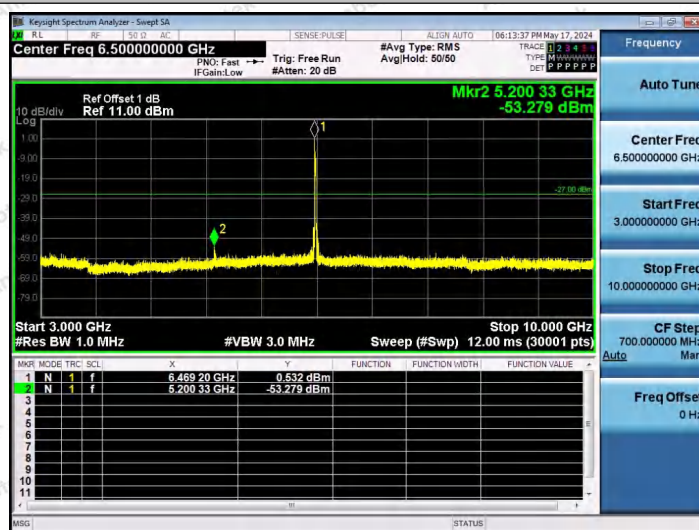
11AX20SISO-Ant1-6475-52Tone-RU37-3000~10000-PASS
