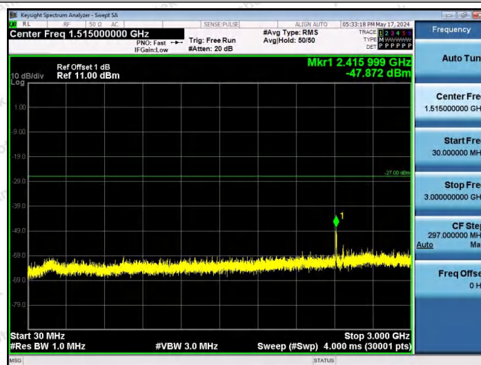
11AX20SISO-Ant1-6415-52Tone-RU40-30~3000-PASS
