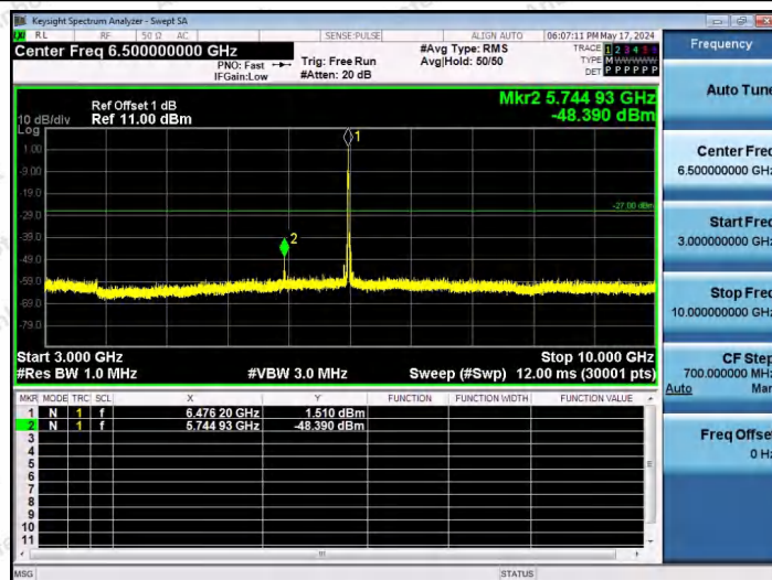
11AX20SISO-Ant1-6475-26Tone-RU4-3000~10000-PASS
