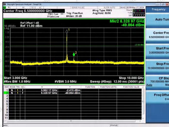
11AX20SISO-Ant1-5955-52Tone-RU40-3000~10000-PASS
