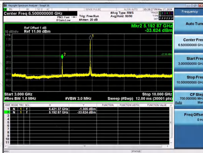
11AX20SISO-Ant1-6415-106Tone-RU54-3000~10000-PASS
