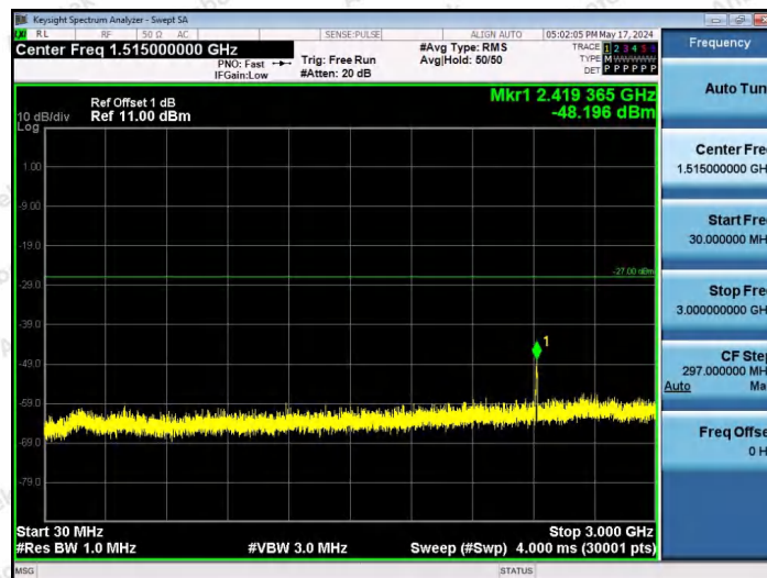
11AX20SISO-Ant1-6175-52Tone-RU39-30~3000-PASS
