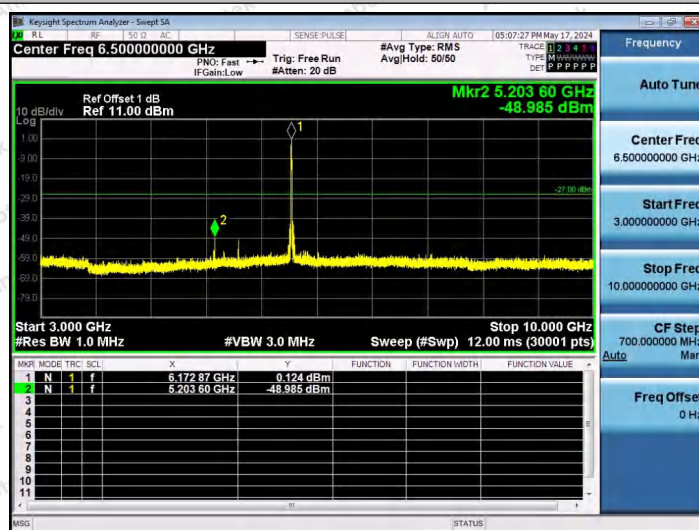
11AX20SISO-Ant1-6175-106Tone-RU53-3000~10000-PASS
