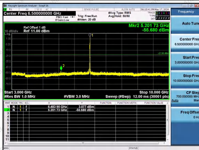
11AX20SISO-Ant1-6475-26Tone-RU8-3000~10000-PASS
