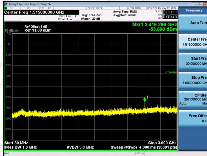
11AX20SISO-Ant1-6435-26Tone-RU0-30~3000-PASS
