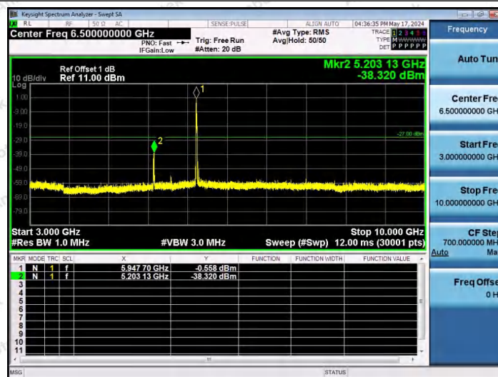
11AX20SISO-Ant1-5955-52Tone-RU37-3000~10000-PASS
