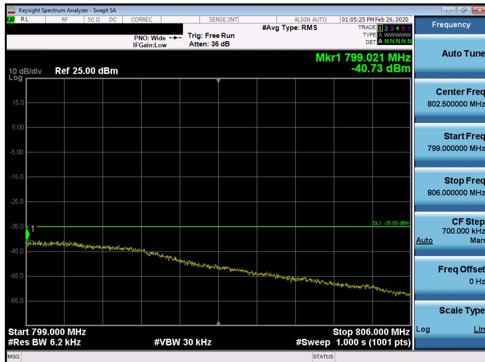
Plot 7-11. Upper Extended Band Edge Plot (Band 14 - 5MHz QPSK - Full RB Configuration)
