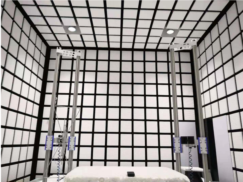
Pic3. Radiated spurious emission (Above 1GHz)
