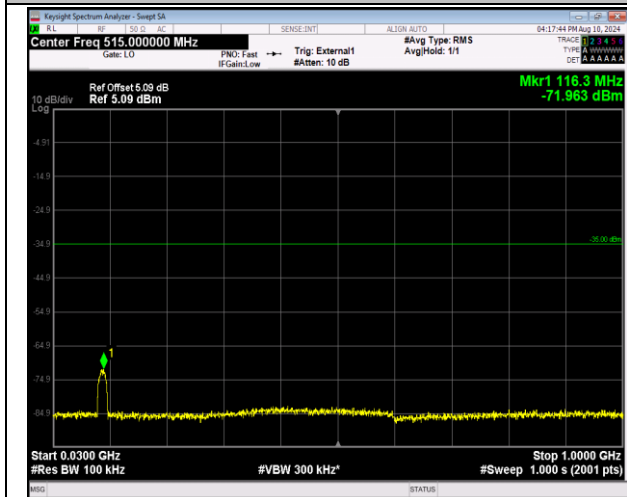
41-41-20MHz-5MHz-QPSK-QPSK-41440-41557-100RB#0-25RB#0-30~1000MHz-PASS
