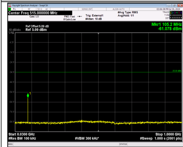
41-41-5MHz-20MHz-64QAM-64QAM-41373-41490-1RB# 0-0RB#0-30~1000MHz-PASS
