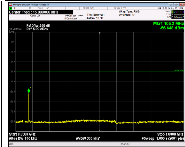
41-41-20MHz-5MHz-16QAM-16QAM-41440-41557-1RB# 0-0RB#0-30~1000MHz-PASS
