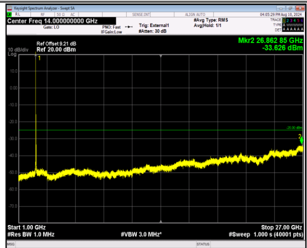
41-41-20MHz-5MHz-QPSK-QPSK-40595-40712-1RB#0-0R B#0-1000~27000MHz-PASS
