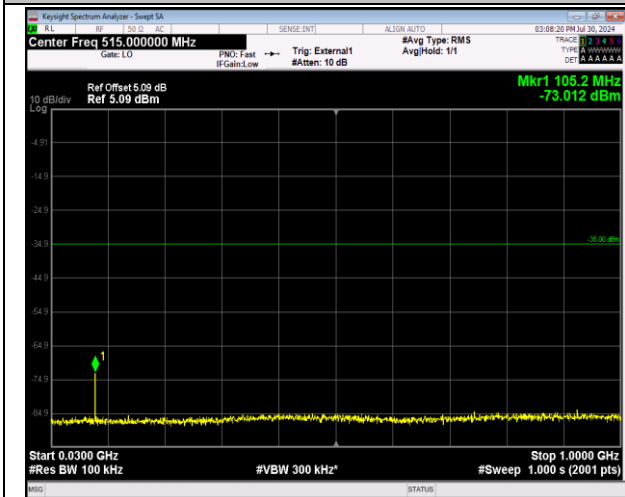
41-41-5MHz-20MHz-64QAM-64QAM-41373-41490-1RB# 0-1RB#99-30~1000MHz-PASS
