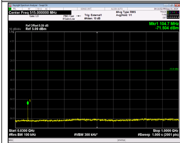
41-41-20MHz-5MHz-16QAM-16QAM-41440-41557-1RB# 0-1RB#24-30~1000MHz-PASS
