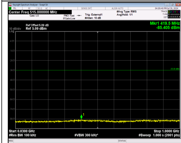
41-41-20MHz-5MHz-64QAM-64QAM-40595-40712-1RB# 0-1RB#24-30~1000MHz-PASS
