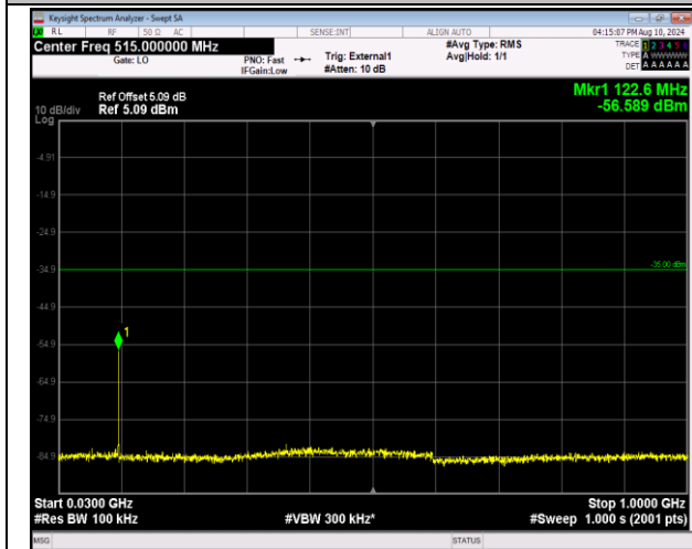
41-41-20MHz-5MHz-16QAM-16QAM-41440-41557-1RB# 99-0RB#0-30~1000MHz-PASS
