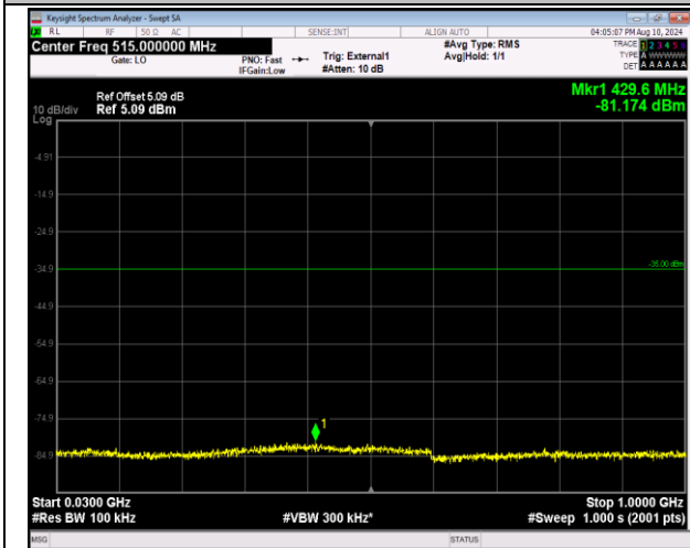
41-41-20MHz-5MHz-QPSK-QPSK-40595-40712-1RB#0- ORB#0-30~1000MHz-PASS
