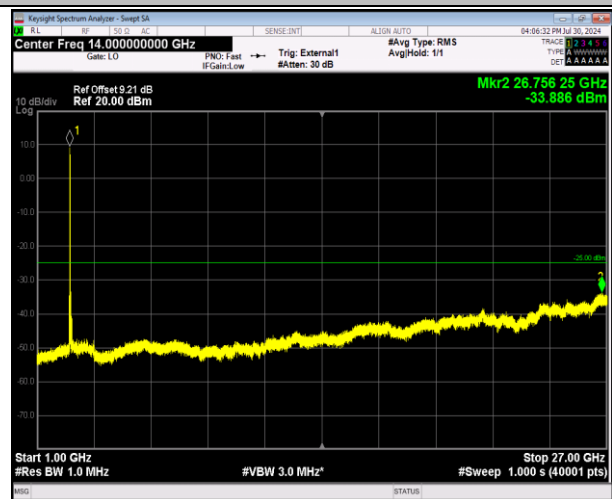
41-41-20MHz-5MHz-64QAM-64QAM-39750-39867-1RB#0- 1RB#24-1000~27000MHz-PASS
