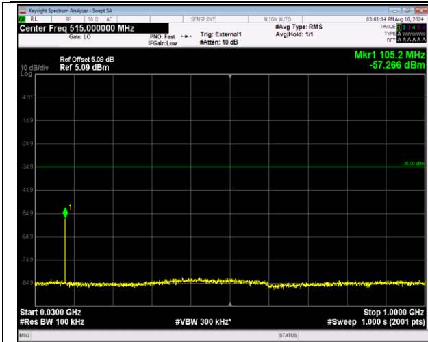
41-41-5MHz-20MHz-16QAM-16QAM-41373-41490-1RB# 0-0RB#0-30~1000MHz-PASS
