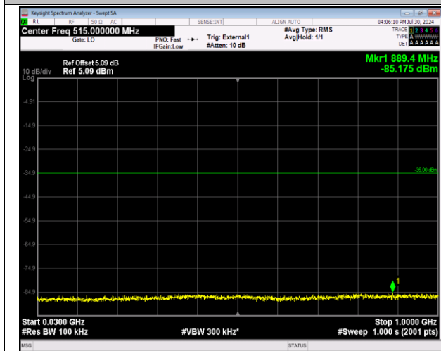
41-41-20MHz-5MHz-64QAM-64QAM-39750-39867-1RB# 0-1RB#24-30~1000MHz-PASS
