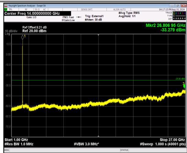
41-41-20MHz-5MHz-16QAM-16QAM-41440-41557-1RB#0- 1RB#24-1000~27000MHz-PASS
