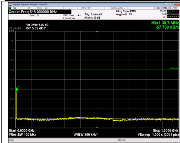
41-41-20MHz-5MHz-64QAM-64QAM-40595-40712-1RB# 99-ORB#0-30~1000MHz-PASS
