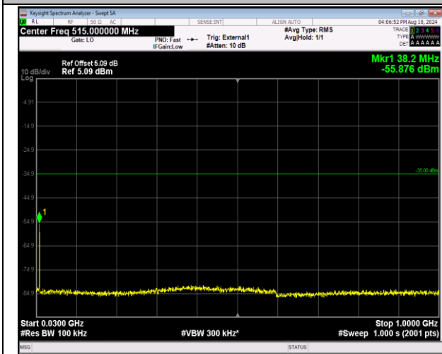
41-41-20MHz-5MHz-QPSK-QPSK-40595-40712-1RB#99-0RB#0-30~1000MHz-PASS
