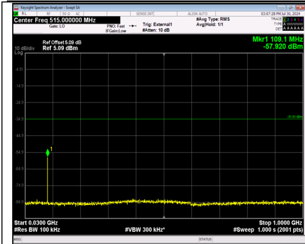
41-41-5MHz-20MHz-64QAM-64QAM-41373-41490-1RB# 24-ORB#0-30~1000MHz-PASS
