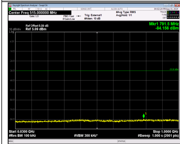
41-41-20MHz-5MHz-16QAM-16QAM-39750-39867-1RB# 0-1RB#24-30~1000MHz-PASS
