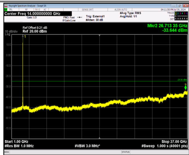
41-41-20MHz-5MHz-64QAM-64QAM-41440-41557-1RB#0- 0RB#0-1000~27000MHz-PASS
