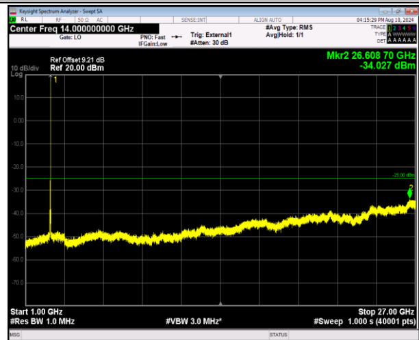
41-41-20MHz-5MHz-16QAM-16QAM-41440-41557-1RB#99 -0RB#0-1000~27000MHz-PASS
