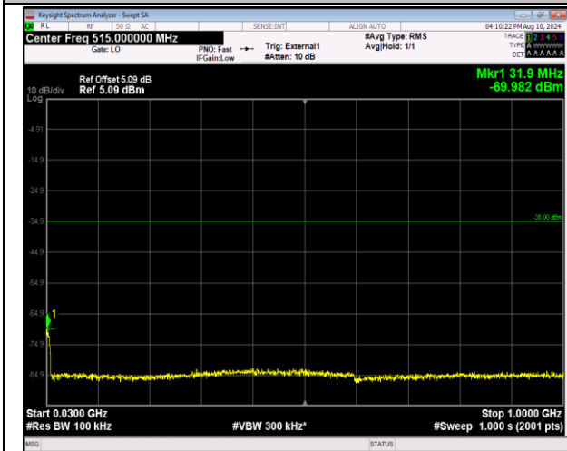
41-41-20MHz-5MHz-QPSK-QPSK-40595-40712-100RB#0-25RB#0-30~1000MHz-PASS
