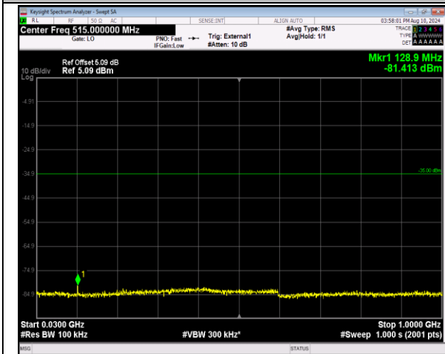
41-41-20MHz-5MHz-QPSK-QPSK-39750-39867-1RB#0-ORB#0-30~1000MHz-PASS
