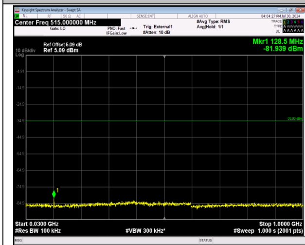
41-41-20MHz-5MHz-64QAM-64QAM-39750-39867-1RB# 0-0RB#0-30~1000MHz-PASS
