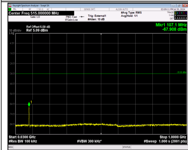
41-41-5MHz-20MHz-64QAM-64QAM-41373-41490-25RB #0-100RB#0-30~1000MHz-PASS
