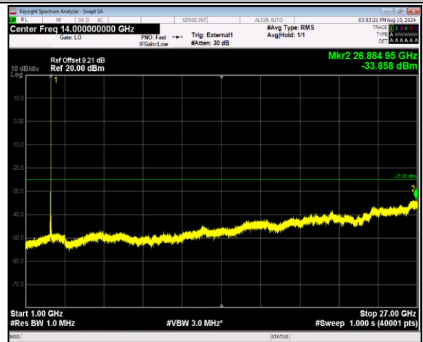
41-41-5MHz-20MHz-16QAM-16QAM-41373-41490-1RB#24 -0RB#0-1000~27000MHz-PASS
