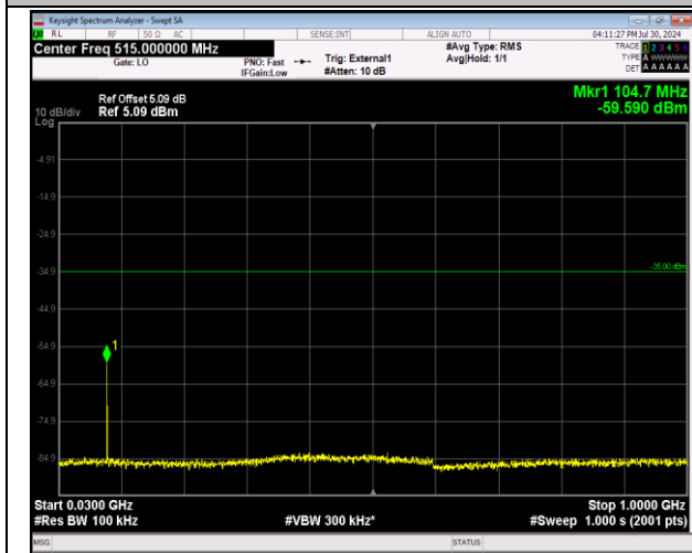
41-41-20MHz-5MHz-64QAM-64QAM-41440-41557-1RB# 0-0RB#0-30~1000MHz-PASS
