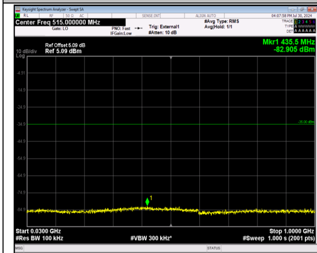
41-41-20MHz-5MHz-64QAM-64QAM-40595-40712-1RB# 0-0RB#0-30~1000MHz-PASS
