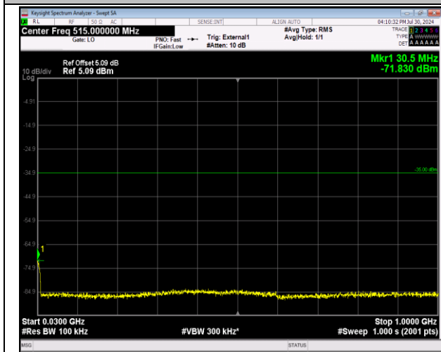
41-41-20MHz-5MHz-64QAM-64QAM-40595-40712-100RB# B#0-25RB#0-30~1000MHz-PASS
