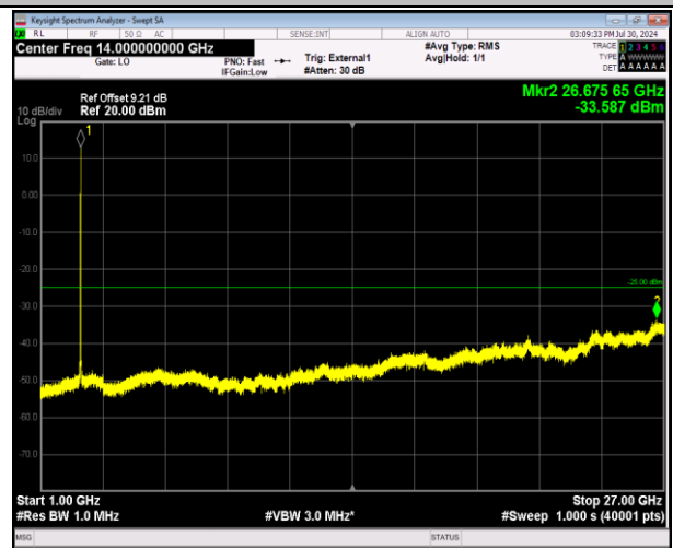
41-41-5MHz-20MHz-64QAM-64QAM-41373-41490-25RB#0 -100RB#0-1000~27000MHz-PASS
