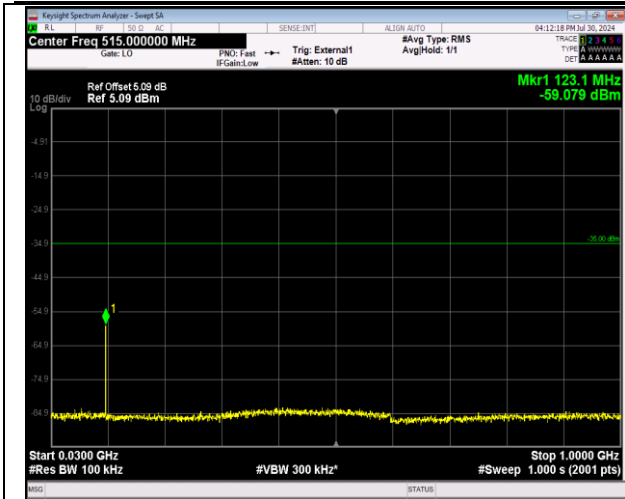
41-41-20MHz-5MHz-64QAM-64QAM-41440-41557-1RB# 99-ORB#0-30~1000MHz-PASS
