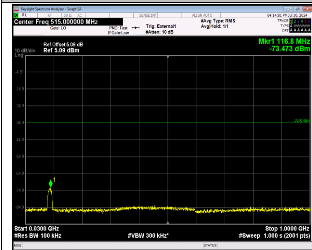
41-41-20MHz-5MHz-64QAM-64QAM-41440-41557-100R B#0-25RB#0-30~1000MHz-PASS
