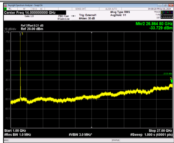
41-41-20MHz-5MHz-64QAM-64QAM-40595-40712-1RB#0- 0RB#0-1000~27000MHz-PASS
