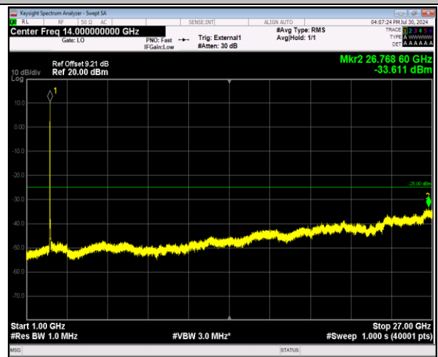
41-41-20MHz-5MHz-64QAM-64QAM-39750-39867-100RB# 0-25RB#0-1000~27000MHz-PASS
