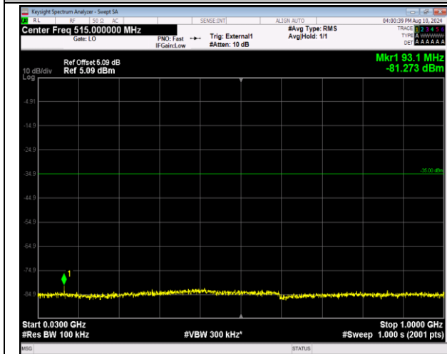
41-41-20MHz-5MHz-16QAM-16QAM-39750-39867-1RB# 99-ORB#0-30~1000MHz-PASS
