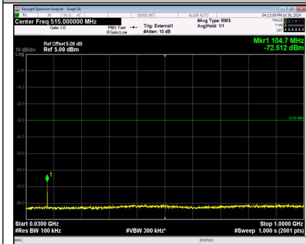
41-41-20MHz-5MHz-64QAM-64QAM-41440-41557-1RB# 0-1RB#24-30~1000MHz-PASS
