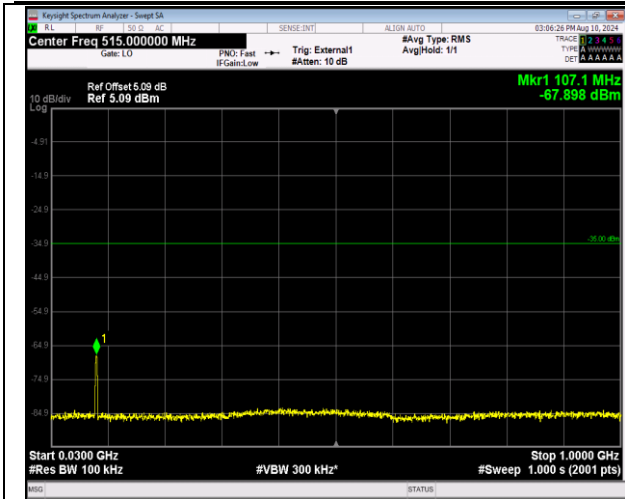
41-41-5MHz-20MHz-16QAM-16QAM-41373-41490-25RB #0-100RB#0-30~1000MHz-PASS
