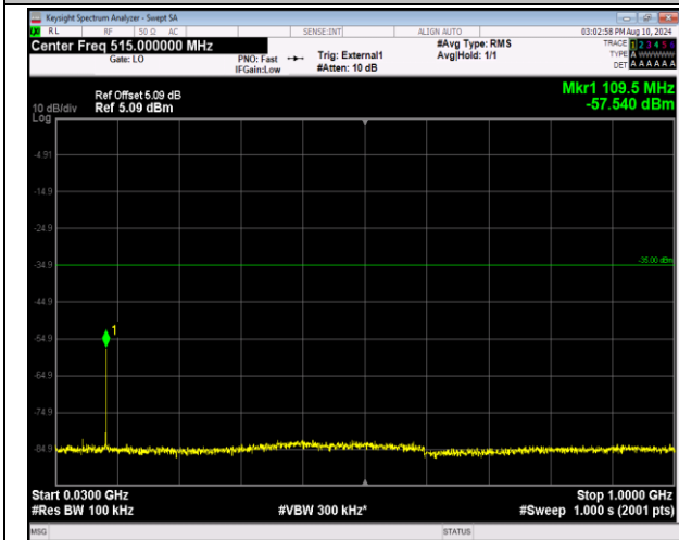
41-41-5MHz-20MHz-16QAM-16QAM-41373-41490-1RB# 24-0RB#0-30~1000MHz-PASS
