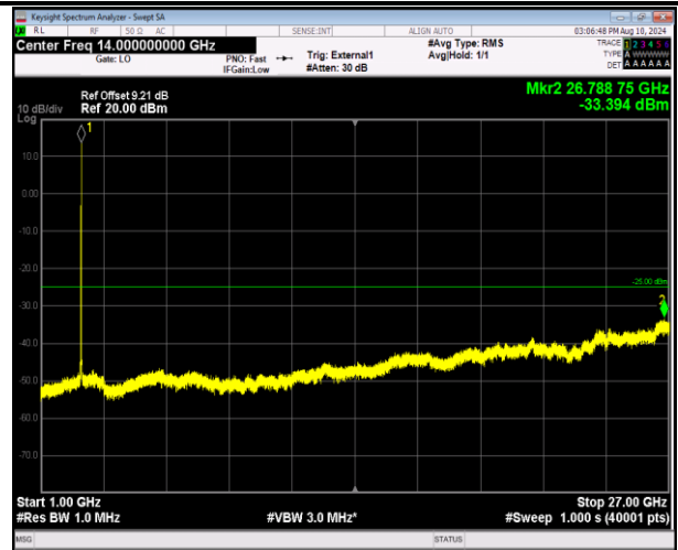
41-41-5MHz-20MHz-16QAM-16QAM-41373-41490-25RB#0 -100RB#0-1000~27000MHz-PASS
