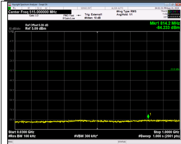
41-41-20MHz-5MHz-QPSK-QPSK-39750-39867-1RB#0-1RB#24-30~1000MHz-PASS
