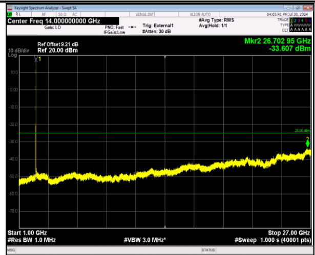
41-41-20MHz-5MHz-64QAM-64QAM-39750-39867-1RB#99 -ORB#0-1000~27000MHz-PASS
