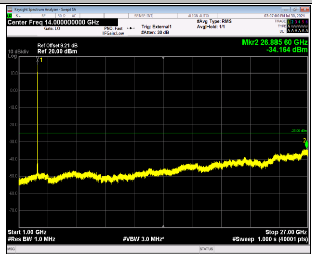
41-41-5MHz-20MHz-64QAM-64QAM-41373-41490-1RB#0- 0RB#0-1000~27000MHz-PASS
