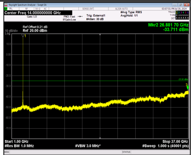
41-41-5MHz-20MHz-64QAM-64QAM-41373-41490-1RB#24 -ORB#0-1000~27000MHz-PASS
