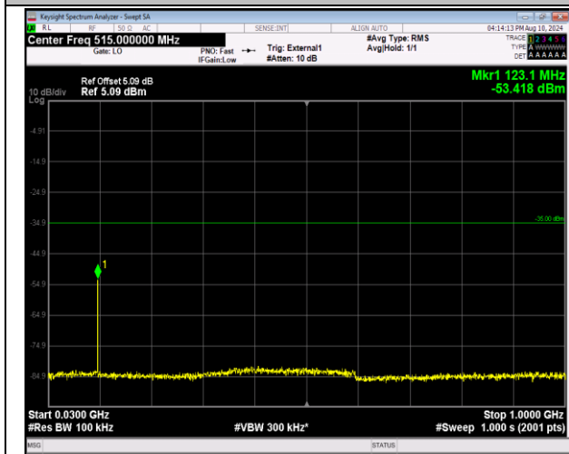
41-41-20MHz-5MHz-QPSK-QPSK-41440-41557-1RB#99-0RB#0-30~1000MHz-PASS
