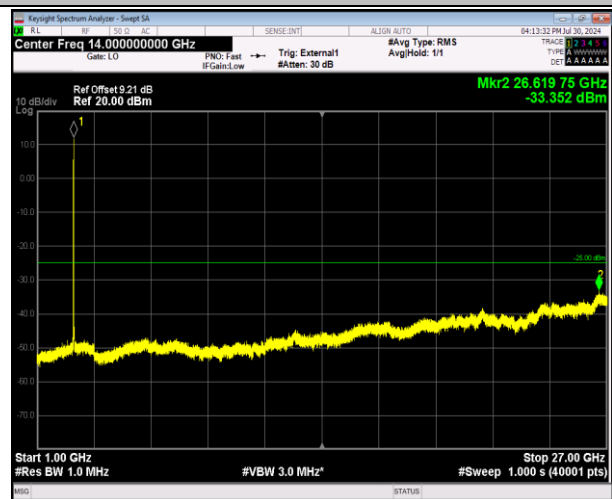
41-41-20MHz-5MHz-64QAM-64QAM-41440-41557-1RB#0- 1RB#24-1000~27000MHz-PASS
