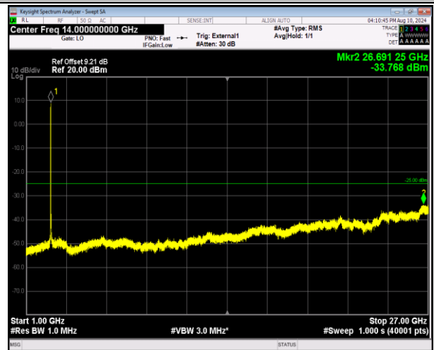
41-41-20MHz-5MHz-QPSK-QPSK-40595-40712-100RB#0-25RB#0-1000~27000MHz-PASS
