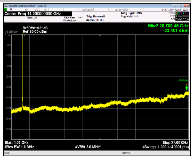
41-41-20MHz-5MHz-QPSK-QPSK-40595-40712-1RB#99-0RB#0-1000~27000MHz-PASS
