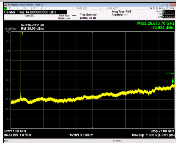
41-41-20MHz-5MHz-16QAM-16QAM-39750-39867-1RB#99 -ORB#0-1000~27000MHz-PASS
