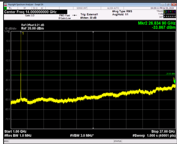
41-41-20MHz-5MHz-64QAM-64QAM-40595-40712-1RB#99 -ORB#0-1000~27000MHz-PASS
