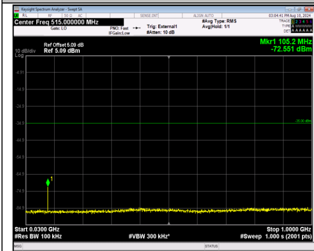
41-41-5MHz-20MHz-16QAM-16QAM-41373-41490-1RB# 0-1RB#99-30~1000MHz-PASS
