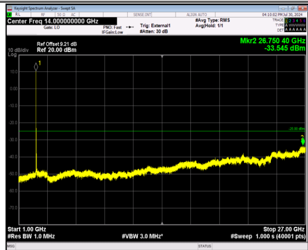
41-41-20MHz-5MHz-64QAM-64QAM-40595-40712-1RB#0- 1RB#24-1000~27000MHz-PASS
