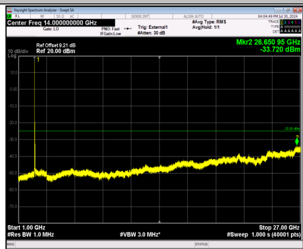
41-41-20MHz-5MHz-64QAM-64QAM-39750-39867-1RB#0- 0RB#0-1000~27000MHz-PASS
