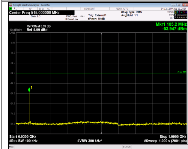
41-41-20MHz-5MHz-QPSK-QPSK-41440-41557-1RB#0-ORB#0-30~1000MHz-PASS
