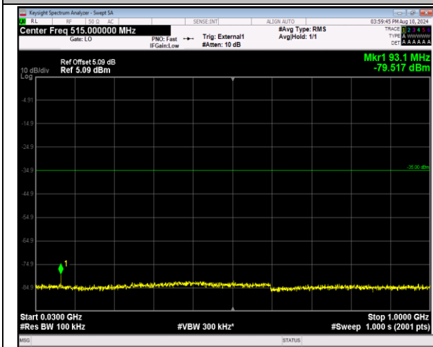
41-41-20MHz-5MHz-QPSK-QPSK-39750-39867-1RB#99-0RB#0-30~1000MHz-PASS
