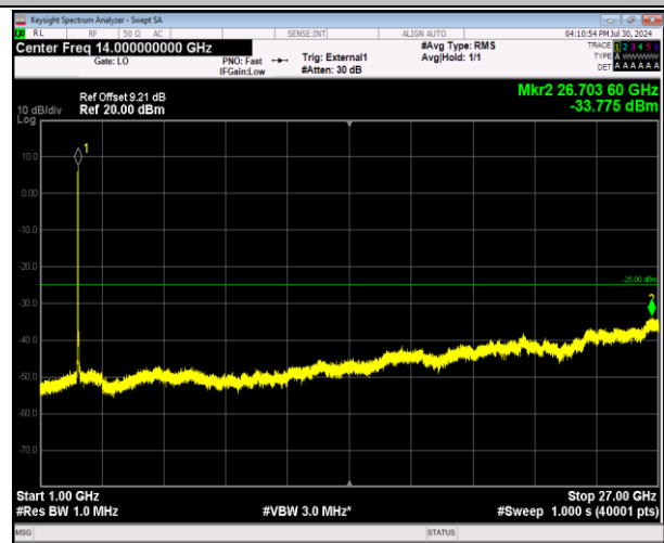
41-41-20MHz-5MHz-64QAM-64QAM-40595-40712-100RB# 0-25RB#0-1000~27000MHz-PASS
