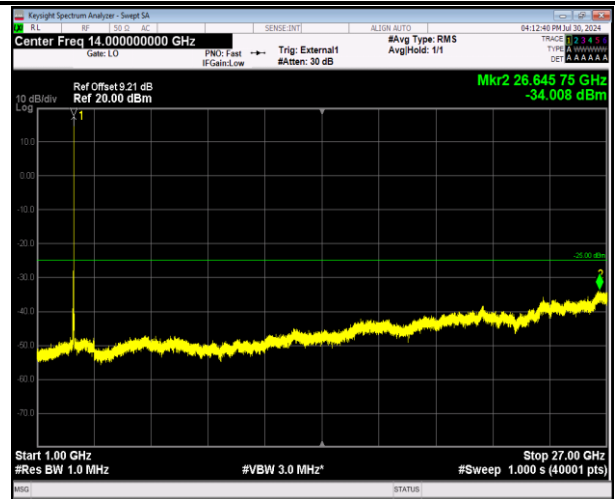
41-41-20MHz-5MHz-64QAM-64QAM-41440-41557-1RB#99 -ORB#0-1000~27000MHz-PASS
