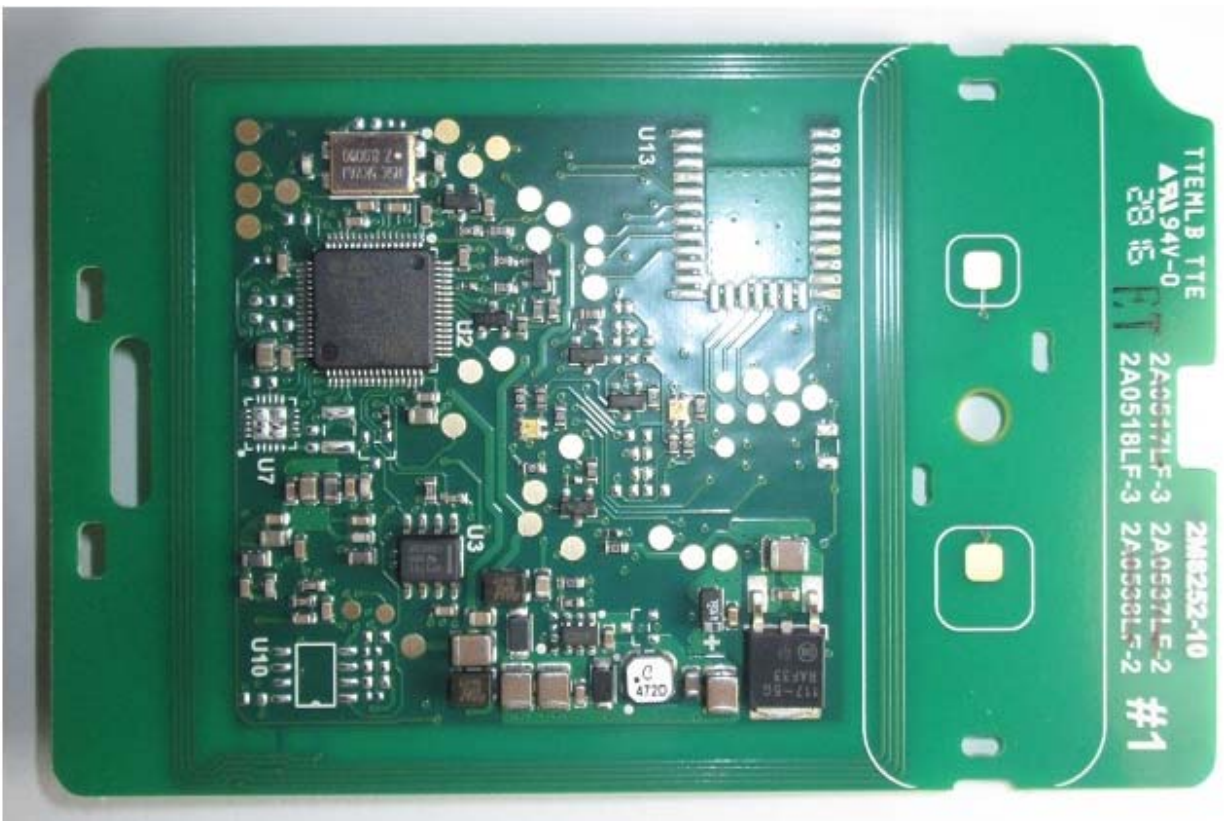
T11 Mifare - PCB (Front Side)
