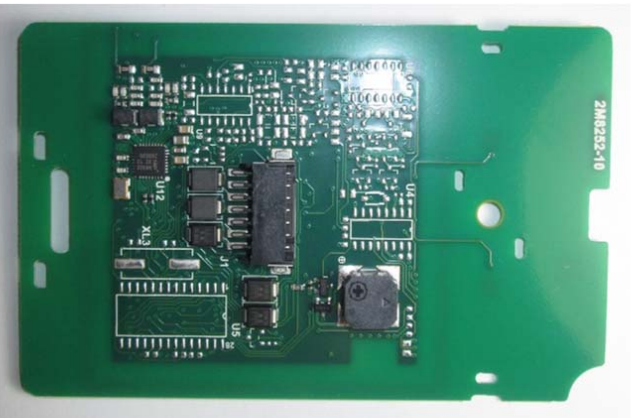
T11 Mifare - PCB (Rear Side)
