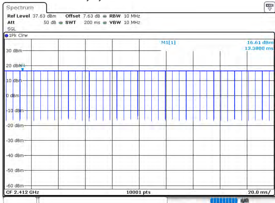
Duty Cycle NVNT 802.11b 2412MHz
