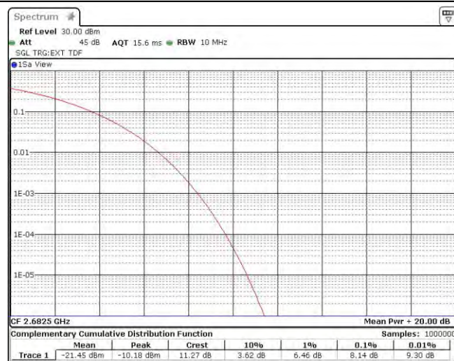
Band41-15MHz-QPSK-41515-75RB#0
