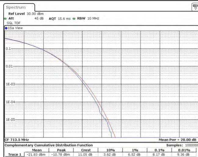
Band12-5MHz-QPSK-23155-25RB#0
