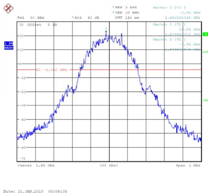
Fig.13 Channel 661- Emission Bandwidth (-26dBc BW)
