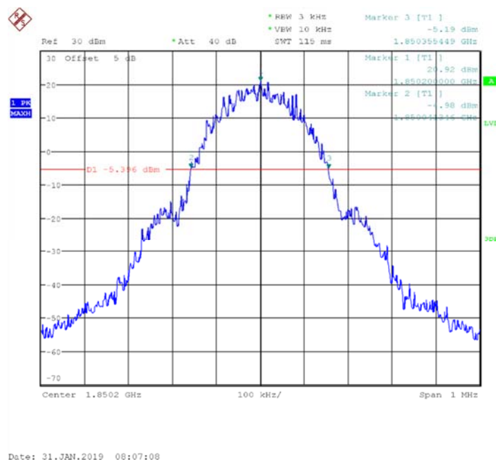
Fig.14 Channel 512- Emission Bandwidth (-26dBc BW)
