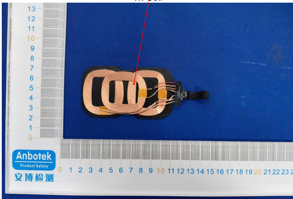
Tx Coil
