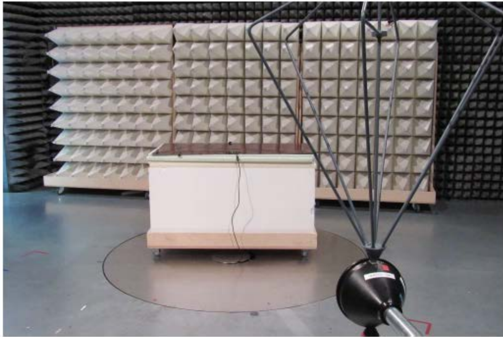
Radiated Setup A
