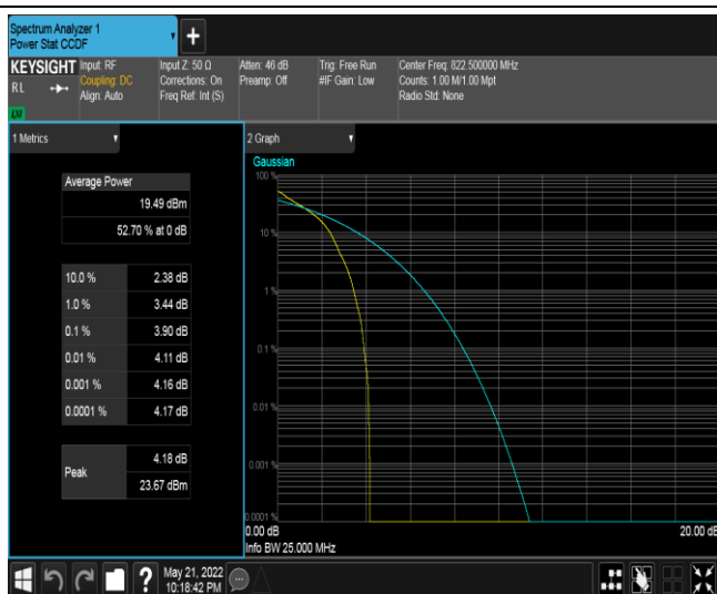
Band18-5MHz-QPSK-23925-25RB#0
