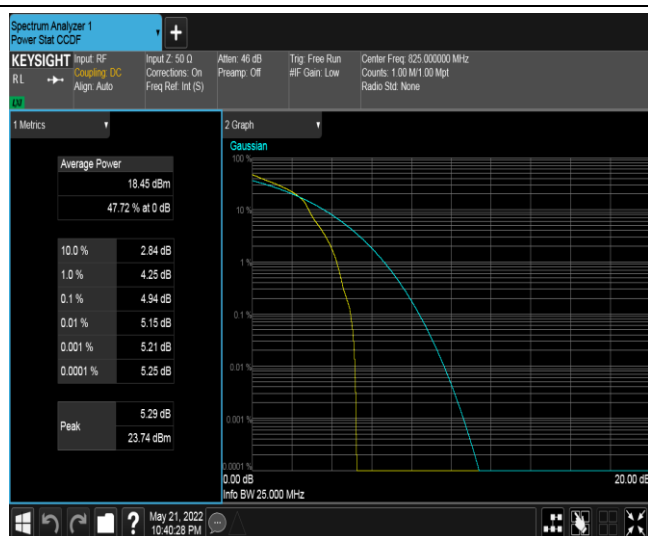
Band18-10MHz-16QAM-23950-50RB#0
