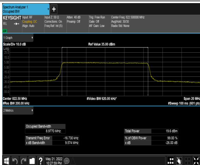
Band18-10MHz-QPSK-23950-50RB#0
