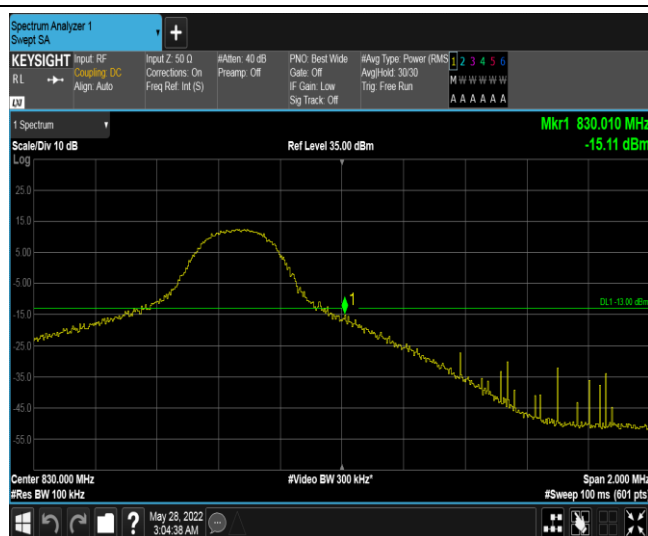
Band18-5MHz-16QAM-23975-25RB#0
