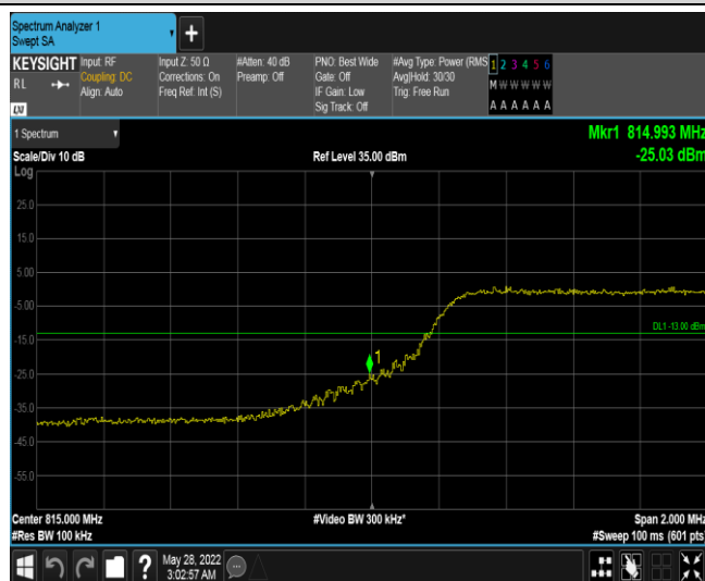
Band18-5MHz-QPSK-23875-25RB#0
