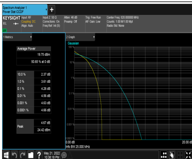
Band18-10MHz-QPSK-239000-50RB#0
