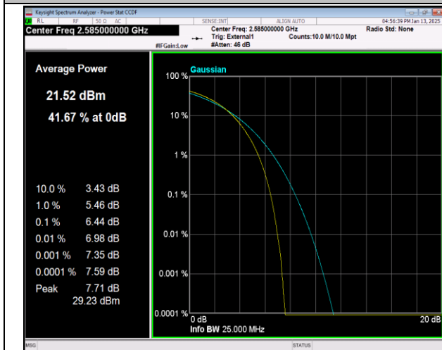
38-38-15MHz-15MHz-QPSK-QPSK-37825-37975-75RB#0-75RB#0-PASS
