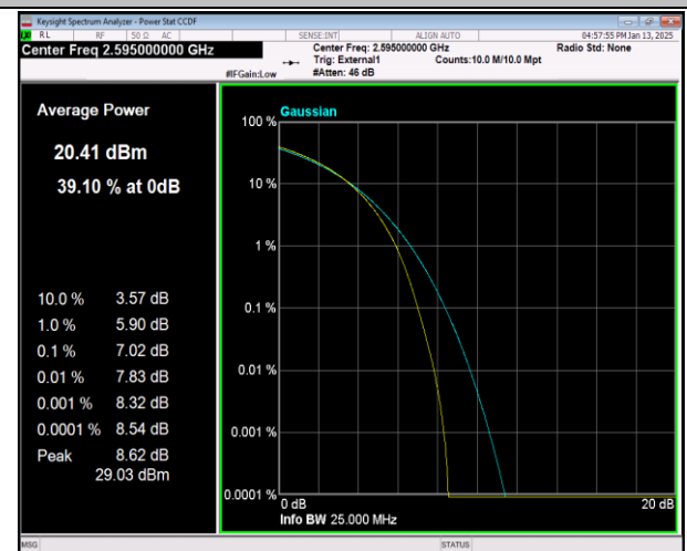
38-38-15MHz-15MHz-16QAM-16QAM-37925-38075-75RB#0-75RB#0-PASS
