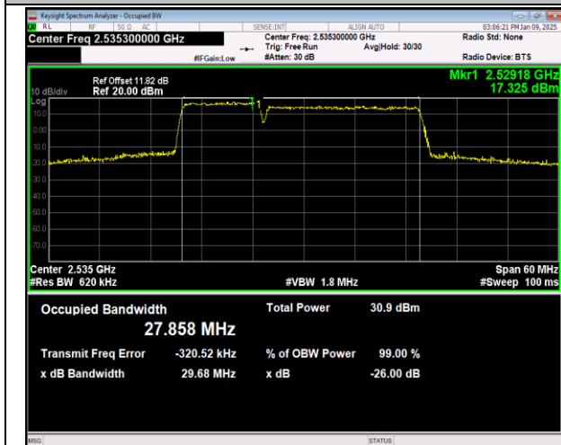
7-7-10MHz-20MHz-QPSK-QPSK-21006-21150-50RB#0-100RB#0-PASS
