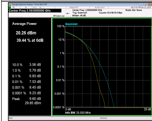
41-41-20MHz-20MHz-QPSK-QPSK-40521-40719-100RB# 0-100RB#0-PASS
