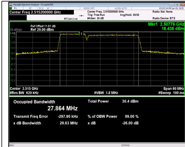
7-7-10MHz-20MHz-QPSK-QPSK-20805-20949-50RB#0-100RB#0-PASS
