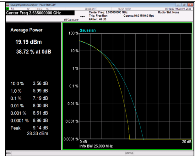
7-7-20MHz-20MHz-16QAM-16QAM-21001-21199-100RB#0-100RB#0-PASS
