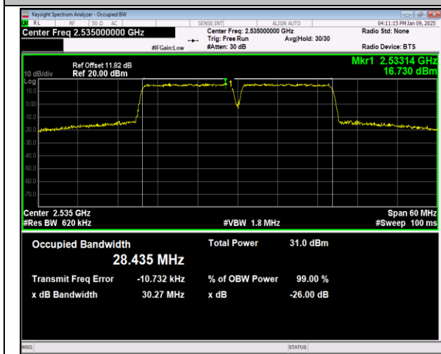
7-7-15MHz-15MHz-QPSK-QPSK-21025-21175-75RB#0-75RB#0-PASS
