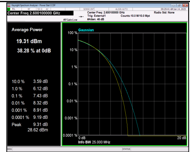
38-38-20MHz-20MHz-16QAM-16QAM-37952-38150-100R B#0-100RB#0-PASS
