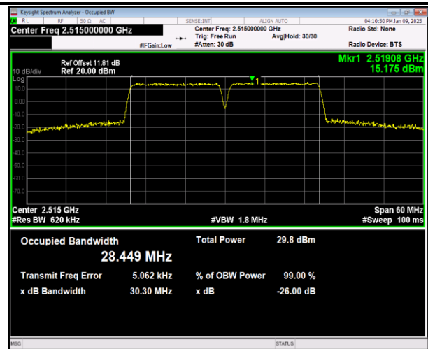
7-7-15MHz-15MHz-16QAM-16QAM-20825-20975-75RB#0-75RB#0-PASS
