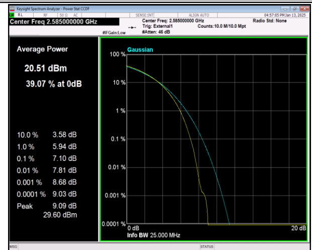
38-38-15MHz-15MHz-16QAM-16QAM-37825-37975-75RB#0-75RB#0-PASS
