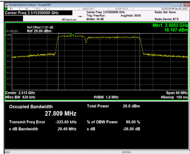
7-7-10MHz-20MHz-16QAM-16QAM-20805-20949-50RB#0-100RB#0-PASS
