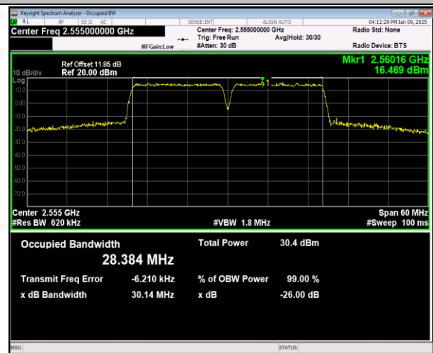
7-7-15MHz-15MHz-16QAM-16QAM-21225-21375-75RB#0-75RB#0-PASS
