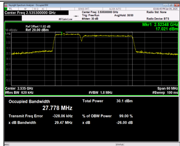
7-7-10MHz-20MHz-16QAM-16QAM-21006-21150-50RB#0-100RB#0-PASS
