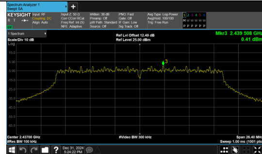
In-Band Reference Level IEEE 802.11n_Channel 6_20MHz_Antenna 0
