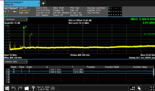
30.0 MHz - 25000.0 MHz IEEE 802.11g_Channel 11_20MHz_Antenna 0
