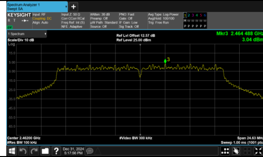
In-Band Reference Level IEEE 802.11g_Channel 11_20MHz_Antenna 0
