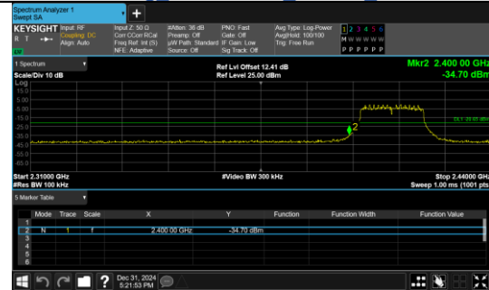
Out Of Band Emission IEEE 802.11n_Channel 1_20MHz_Antenna 0
