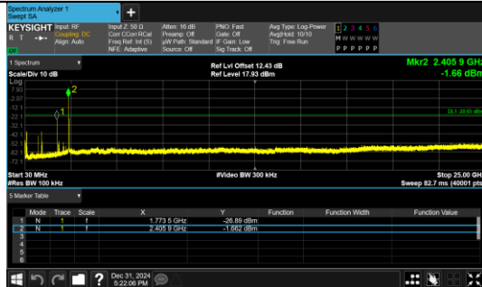
30.0 MHz - 25000.0 MHz IEEE 802.11n_Channel 1_20MHz_Antenna 0
