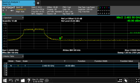
Out Of Band Emission IEEE 802.11g_Channel 11_20MHz_Antenna 0
