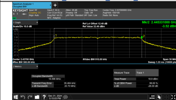
IEEE 802.11g Channel 6 20MHz Antenna 0
