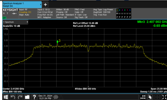
In-Band Reference Level IEEE 802.11n_Channel 1_20MHz_Antenna 0
