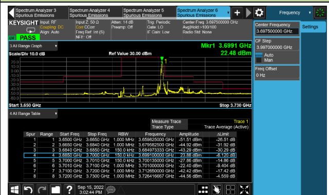
20MHz Channel Bandwidth - 1RB
