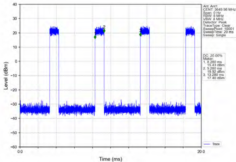
n78d_30kHz_MIMO_NTNV_100MHz_CP-OFDM 64 QAM_3649.98MHz_Inner_Full
