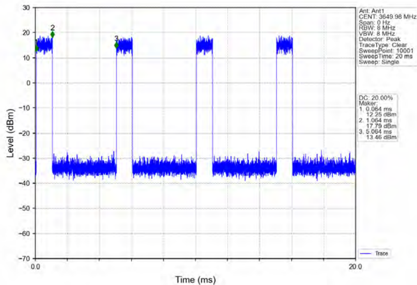
n78d_30kHz_MIMO_NTNV_100MHz_CP-OFDM_256_QAM_3649.98MHz_Inner_Full
