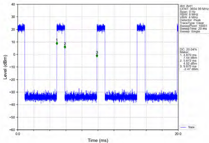
n78d_30kHz_MIMO_NTNV_90MHz_CP-OFDM 64 QAM_3654.99MHz_Inner_Full
