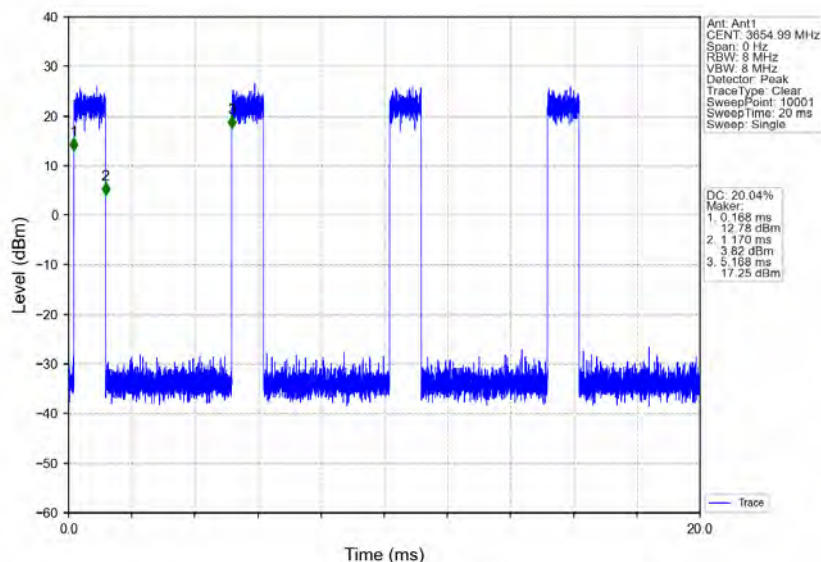
n78d_30kHz_MIMO_NTNV_90MHz_CP-OFDM_16_QAM_3654.99MHz_Inner_Full
