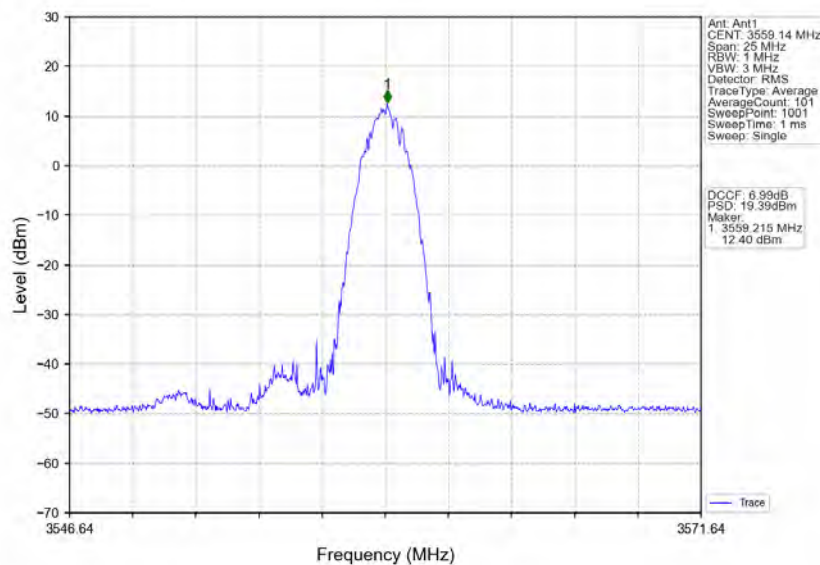
n78d_30kHz_MIMO_NTNV_10MHz_CP-OFDM_16_QAM_3555MHz_Edge_1RB_Right
