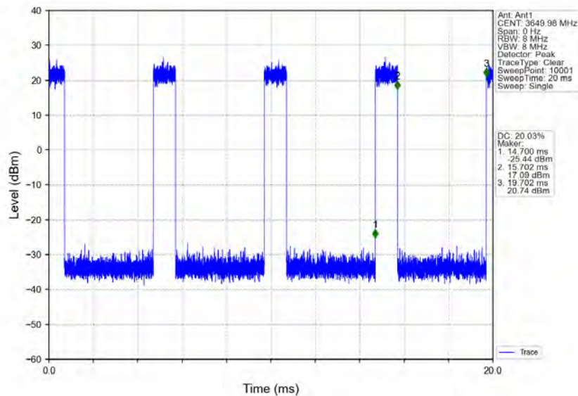
n78d_30kHz_MIMO_NTNV_100MHz_CP-OFDM QPSK_3649.98MHz_Inner_Full
