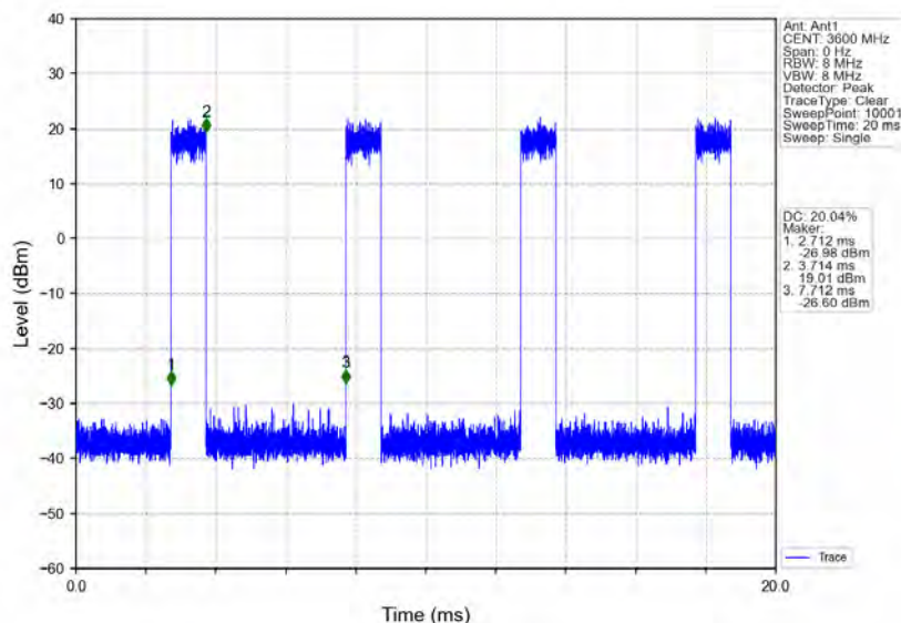
n78d_30kHz_MIMO_NTNV_100MHz_CP-OFDM 256 QAM_3600MHz_Inner_Full
