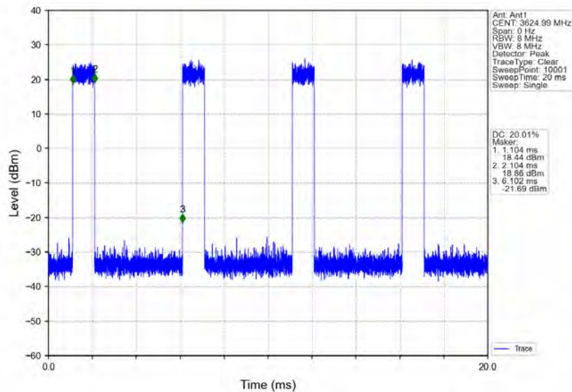
n78d_30kHz_MIMO_NTNV_90MHz_CP-OFDM 64 QAM_3624.99MHz_Inner_Full
