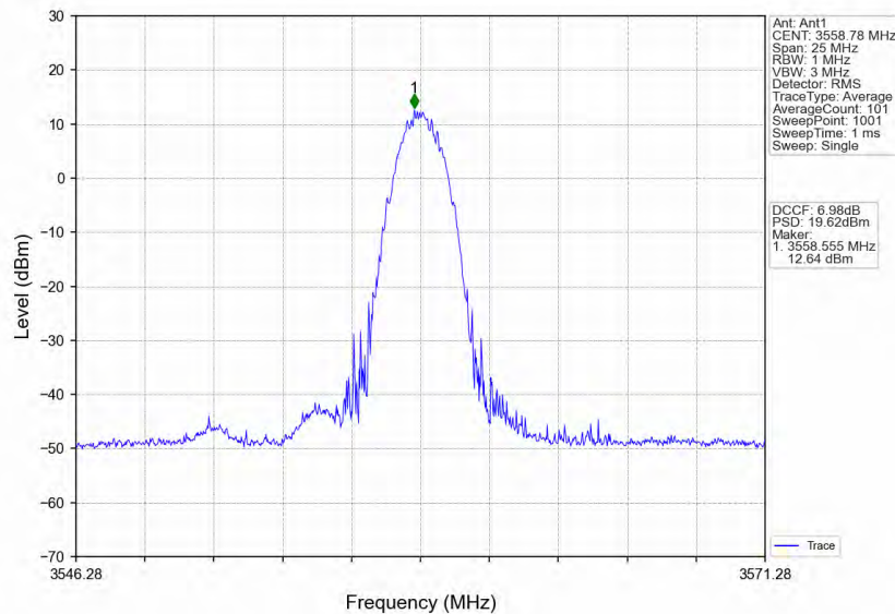
n78d_30kHz_MIMO_NTNV_10MHz_CP-OFDM_16_QAM_3555MHz_Inner_1RB_Right
