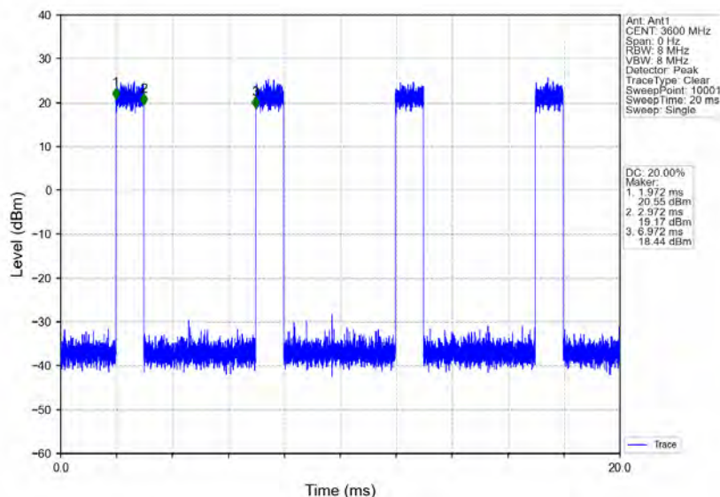
n78d_30kHz_MIMO_NTNV_100MHz_CP-OFDM_QPSK_3600MHz_Inner_Full
