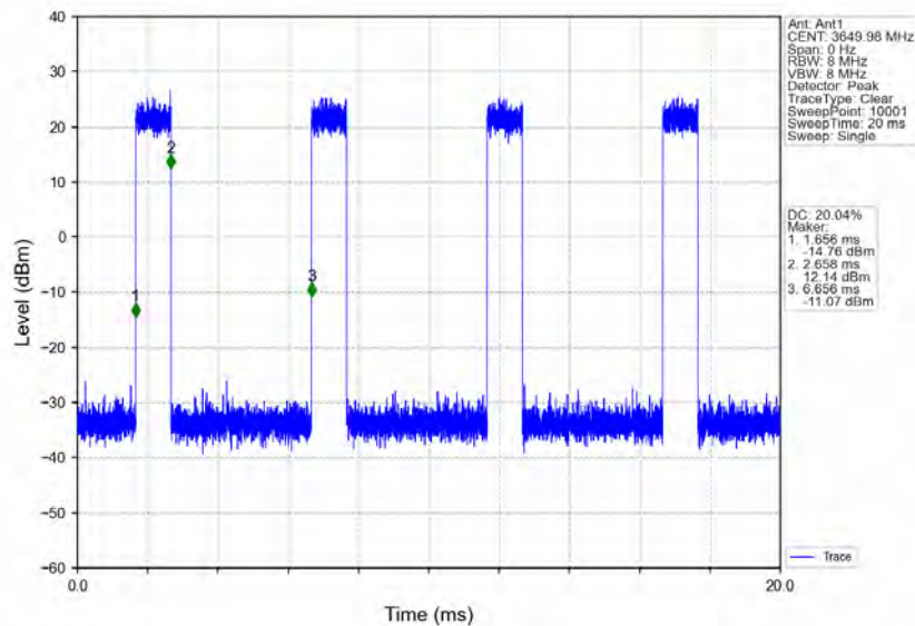
n78d_30kHz_MIMO_NTNV_100MHz_CP-OFDM_16_QAM_3649.98MHz_Inner_Full
