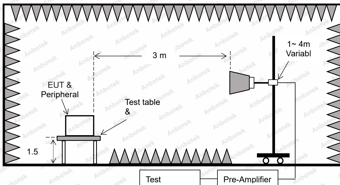
Figure 3. Above 1 GHz
