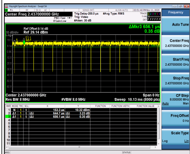
802.11g
