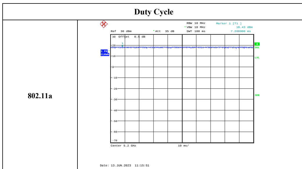
Duty Cycle
