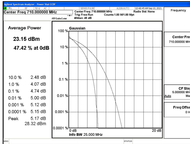
Band17-10MHz-QPSK-23790-50RB#0
