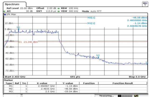
CH11-Bandedge
