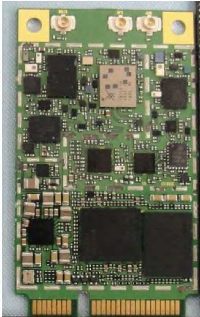
LTE module (without shield)
