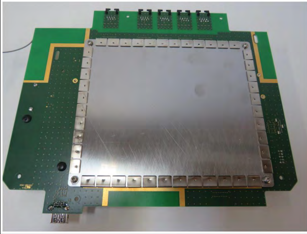
EUT PCB BACK (with shielding)
