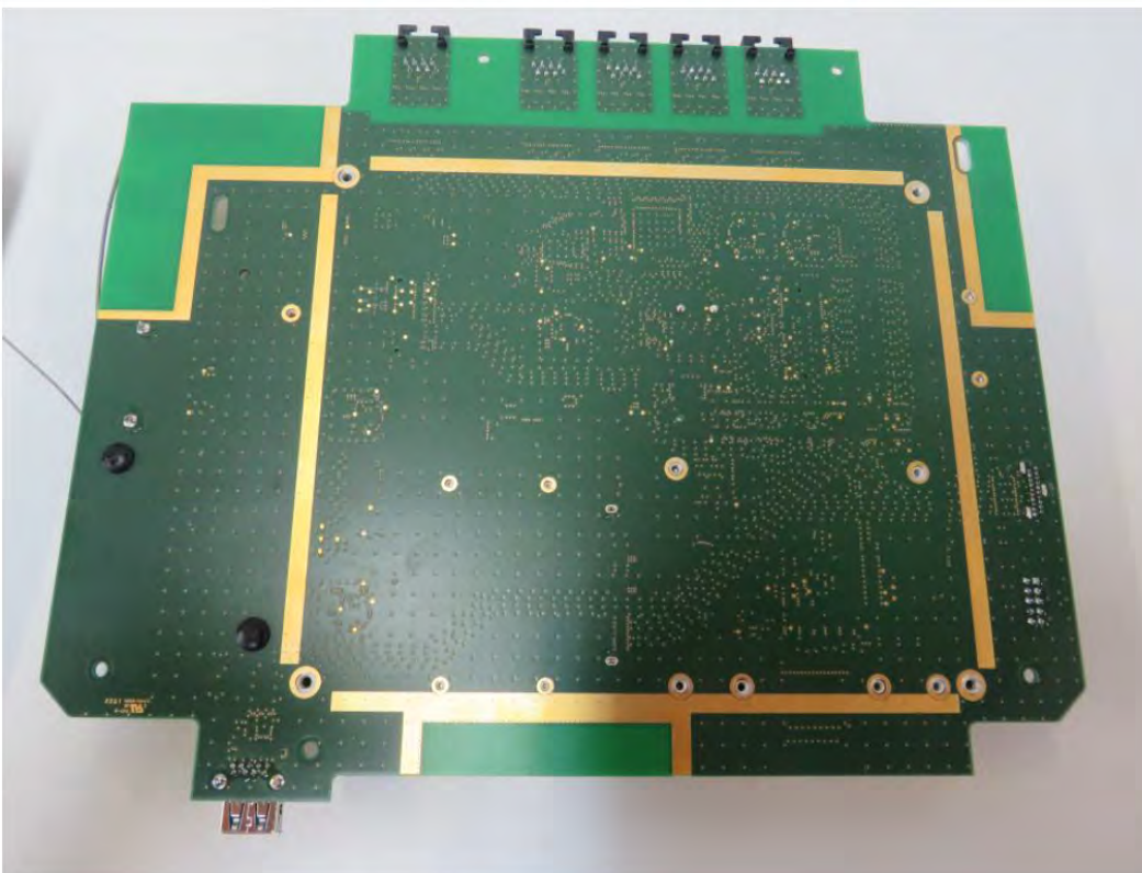
EUT PCB BACK (without shielding)
