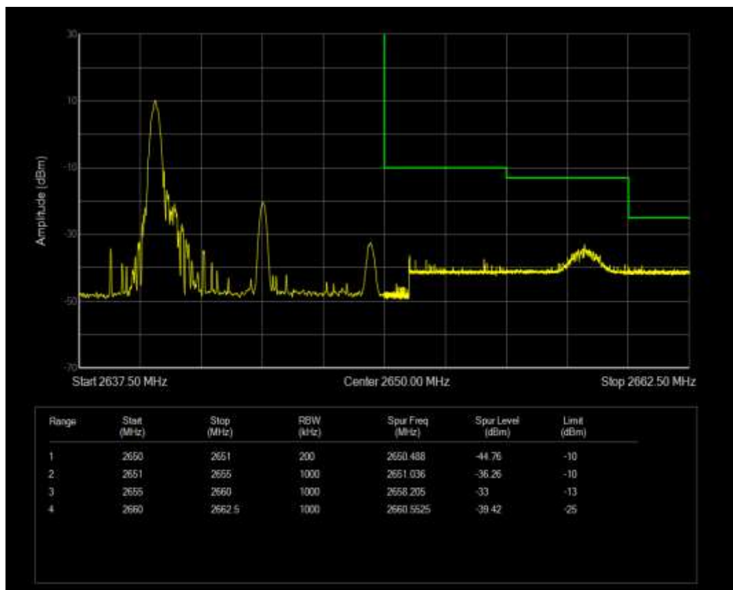
Band41 16QAM BW=10MHz Channel=41140 RB Size=1 Position=#Max
