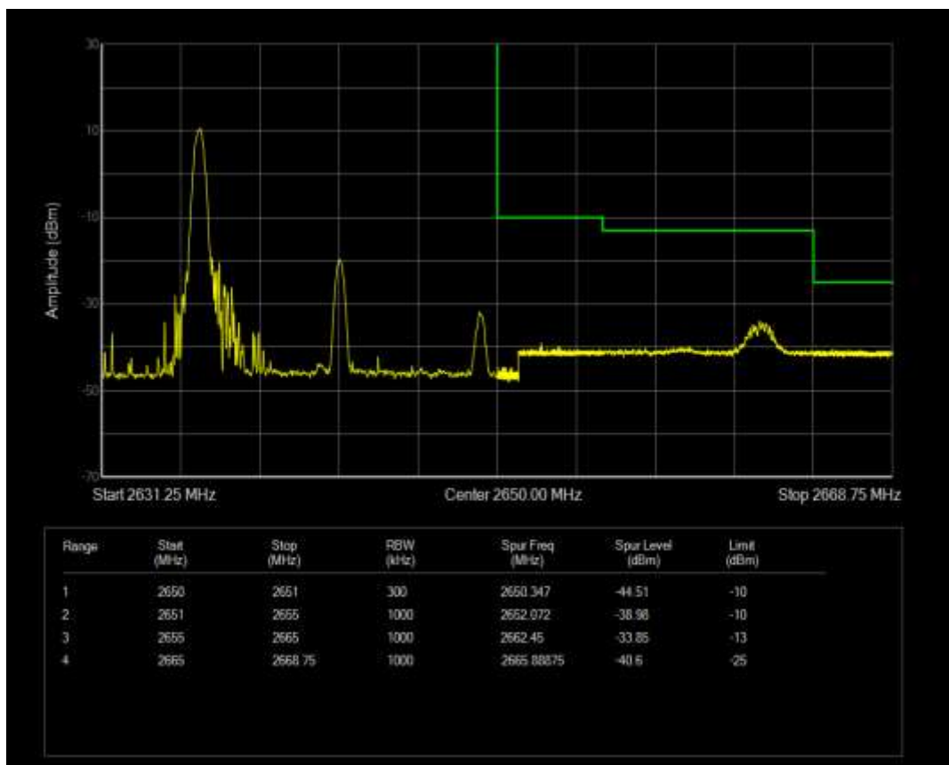
Band41 16QAM BW=15MHz Channel=41115 RB Size=1 Position=#Max
