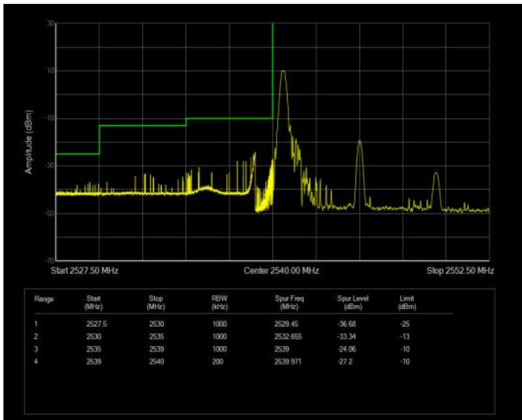
Band41 QPSK BW=10MHz Channel=40140 RB Size=1 Position=#Max
