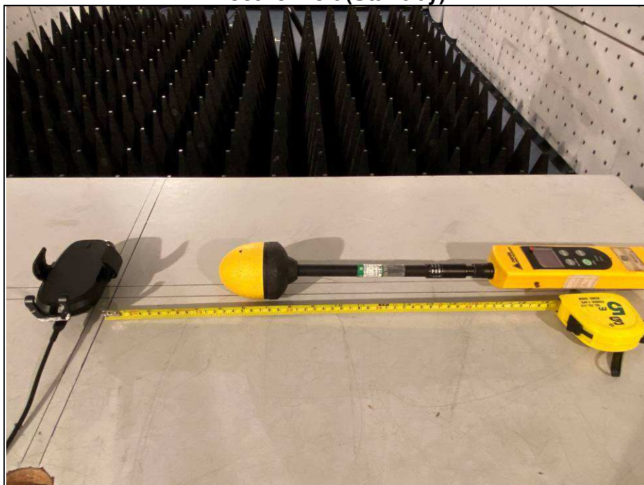
Electric Field(Standby)
