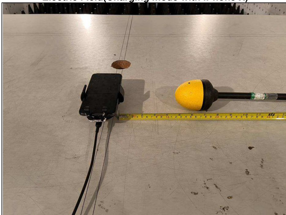
Electric Field(Charging mode with iPhone X)
