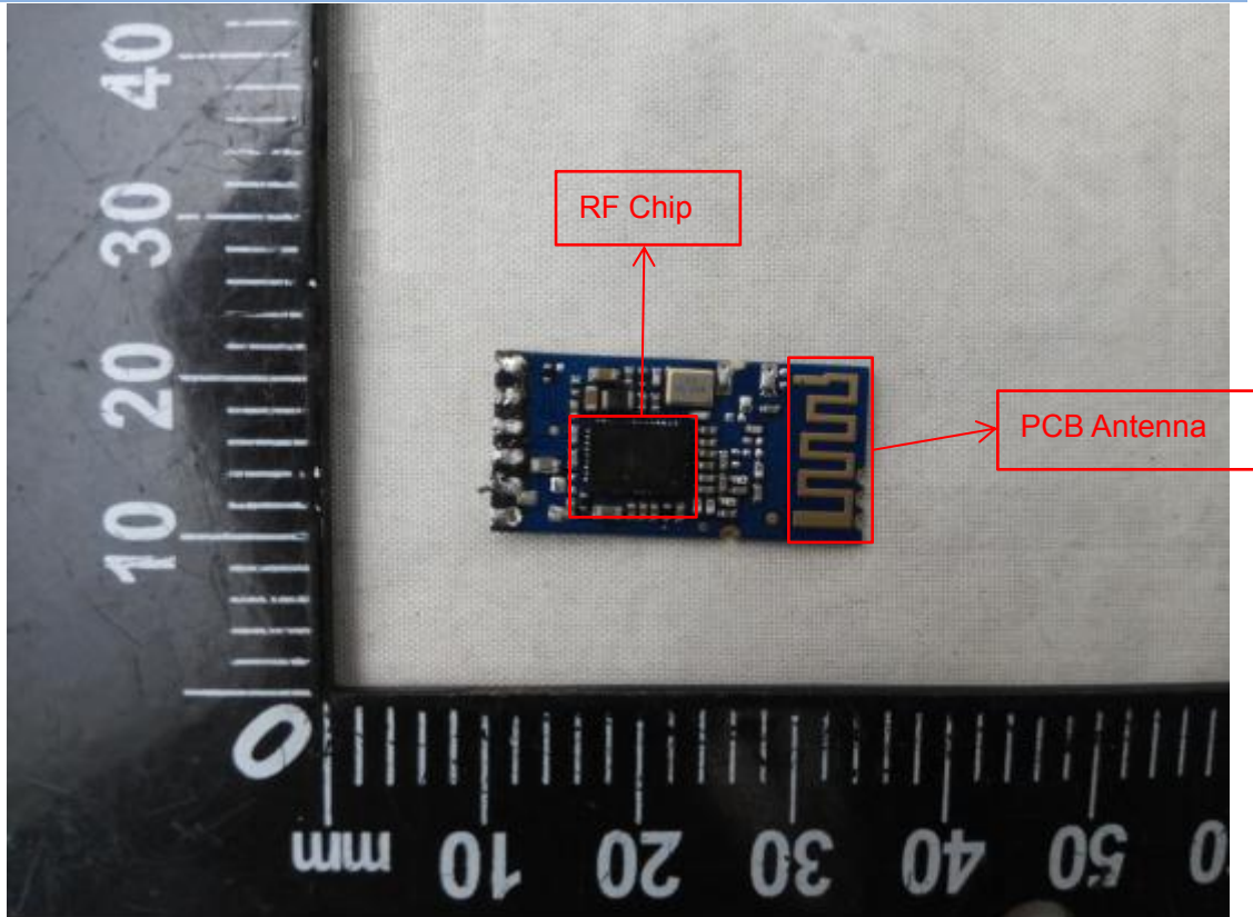
MAIN BOARD BACK VIEW 4
