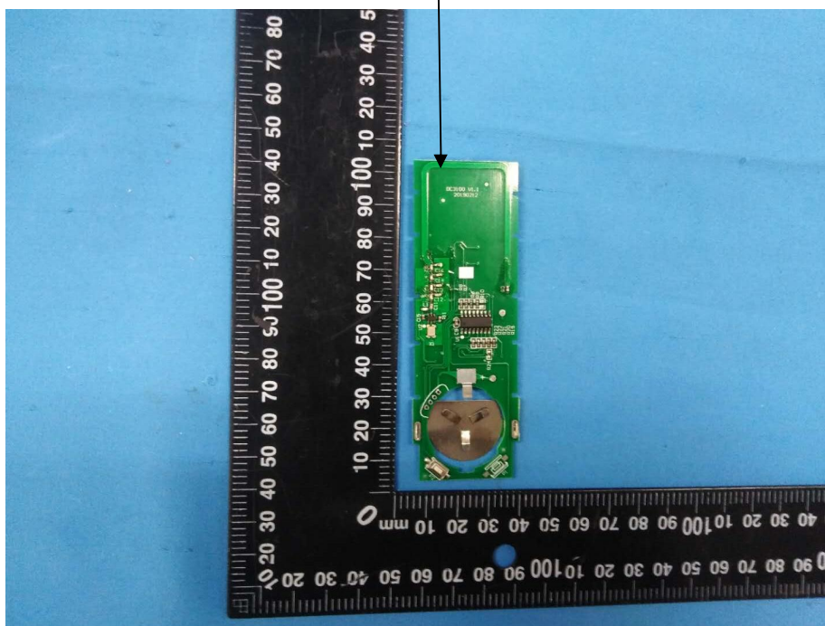
RF Antenna
