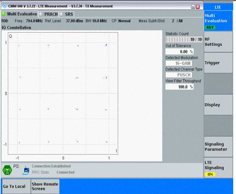
Band12-10MHz-16QAM-23060-1RB#0-PASS
