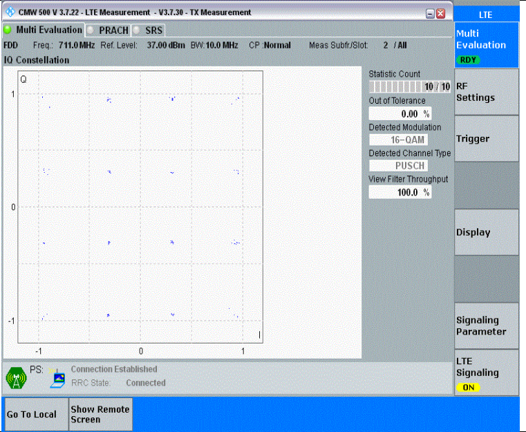
Band12-10MHz-16QAM-23130-1RB#0-PASS
