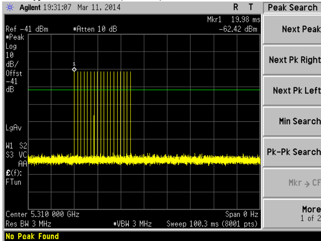
Radar Type 1 Calibration Plot (5310MHz)
