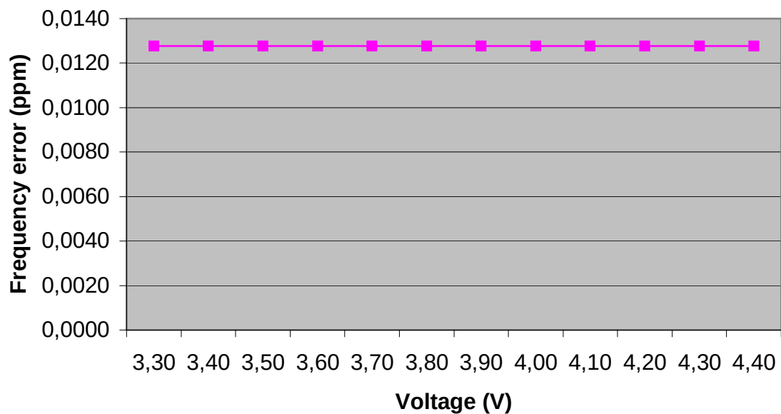
Frequency Error vs. Voltage
