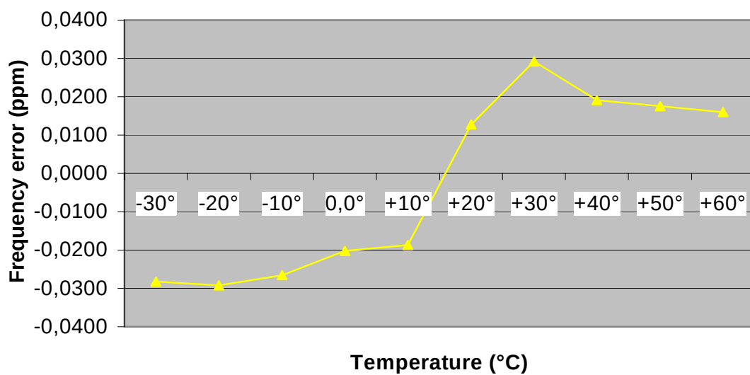
Frequency Error vs. Temperatur
