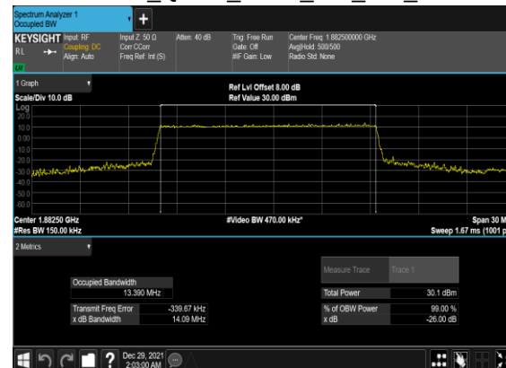
B12_N25(15M)_DFT-s- OFDM_QPSK_Outer_Full_Mid_CH
