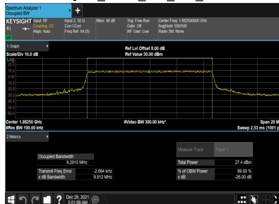
B12_N25(10M)_CP-OFDM_16 QAM_Outer_Full_Mid_CH
