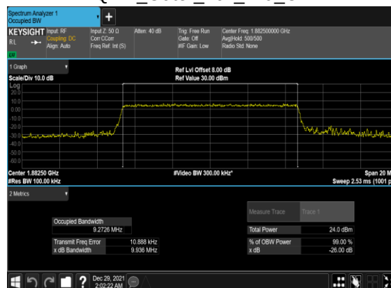
B12_N25(10M)_CP-OFDM_256 QAM_Outer_Full_Mid_CH
