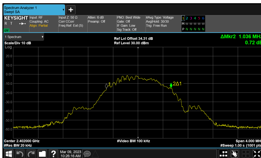
Figure 121 - Core 0 (B) 2402 MHz (CH37) 99% Bandwidth
