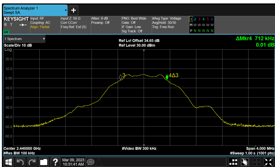
Figure 128 - Core 1 (C) 2440 MHz (CH17) 6 dB Bandwidth
