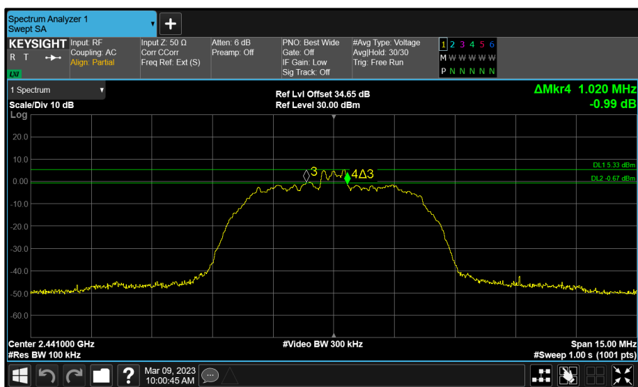
Figure 104 - Core 1 (C) 2441 MHz (CH39) 6 dB Bandwidth
