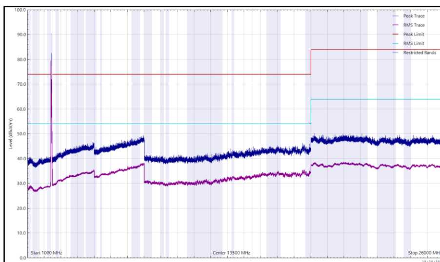
Figure 149 - 2440 MHz (CH17), LE1M, iPA, Core 0 + Core 1, 1 GHz to 26 GHz, Horizontal
