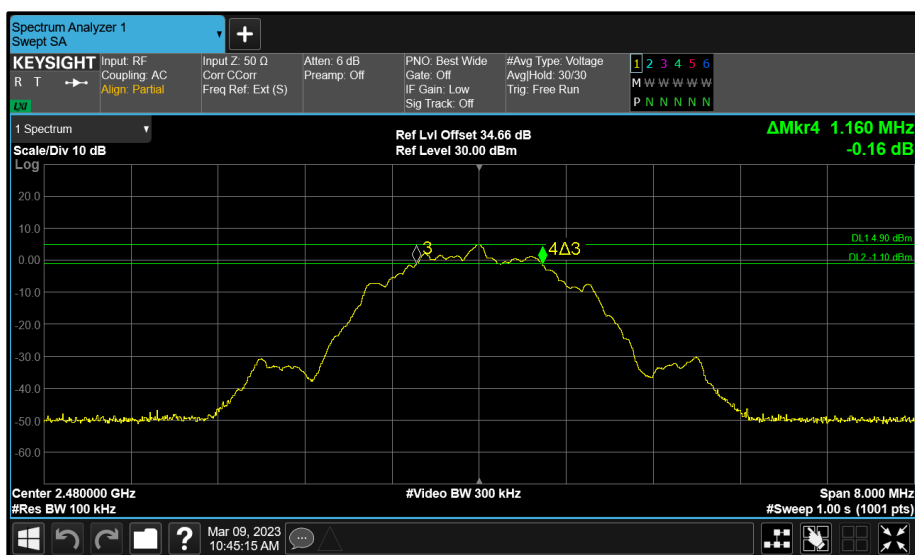
Figure 144 - Core 1 (C) 2480 MHz (CH39) 6 dB Bandwidth
