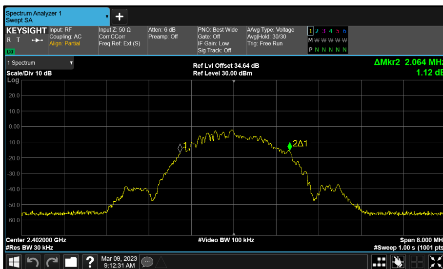
Figure 115 - Core 1 (C) 2402 MHz (CH37) 99% Bandwidth
