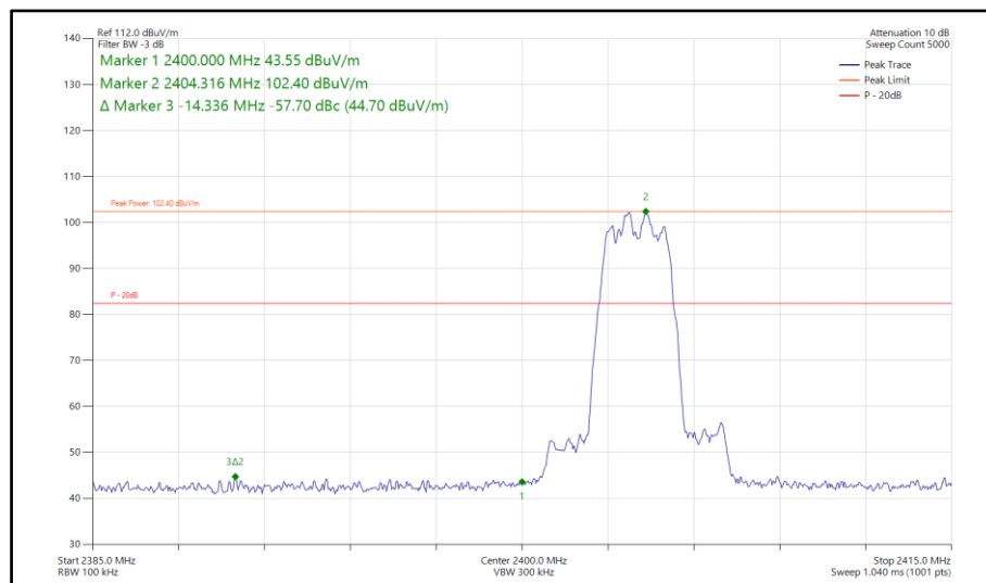
Figure 154 - Bluetooth HDR4, SISO, Core 0 - 2404 MHz, Band Edge Frequency 2400 MHz
