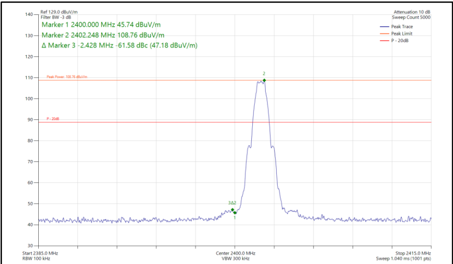
Figure 156 - Bluetooth LE1M, SISO, Core 1 - 2402 MHz Band Edge Frequency 2400 MHz
