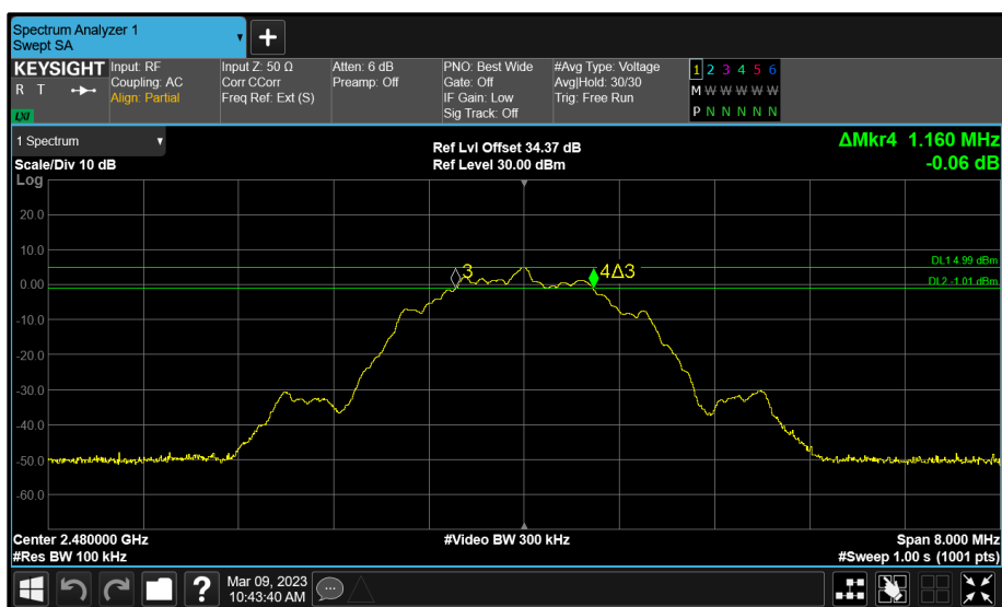
Figure 142 - Core 0 (B) 2480 MHz (CH39) 6 dB Bandwidth
