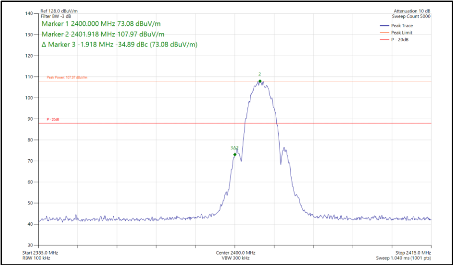
Figure 157 - Bluetooth LE2M, SISO, Core 1 - 2402 MHz Band Edge Frequency 2400 MHz
