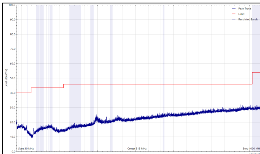
Figure 148 - 2440 MHz (CH17), LE1M, iPA, Core 0 + Core 1, 30 MHz to 1 GHz, Horizontal (Peak)
