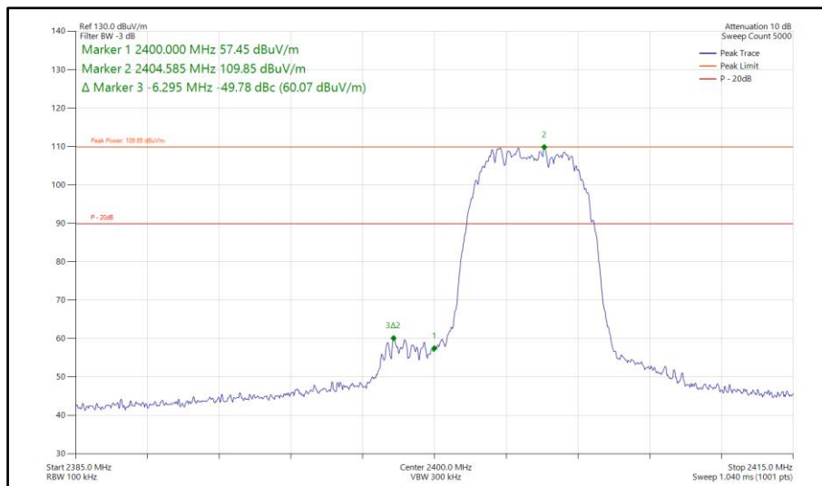
Figure 163 - Bluetooth HDR8, MIMO, Core 0-1 - 2404 MHz, Band Edge Frequency 2400 MHz
