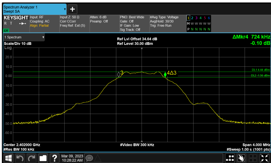
Figure 124 - Core 1 (C) 2402 MHz (CH37) 6 dB Bandwidth
