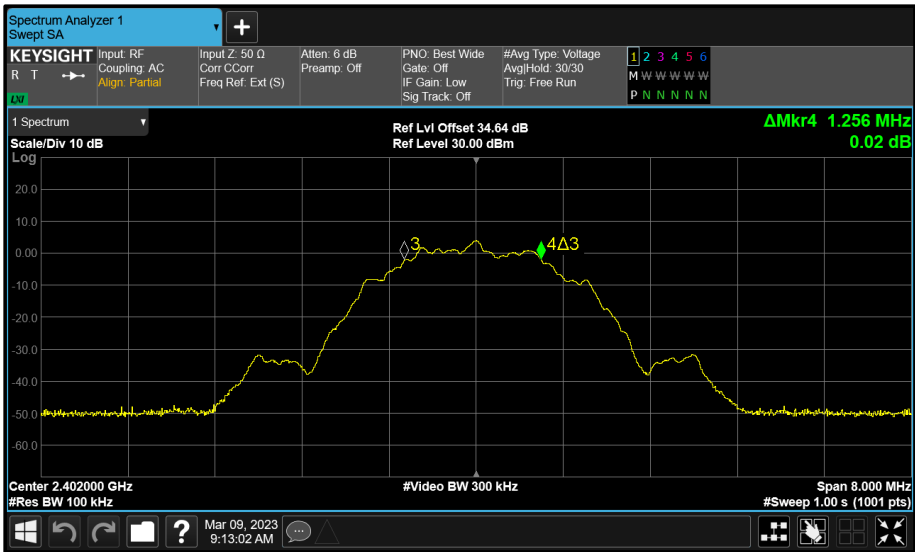
Figure 116 - Core 1 (C) 2402 MHz (CH37) 6 dB Bandwidth
