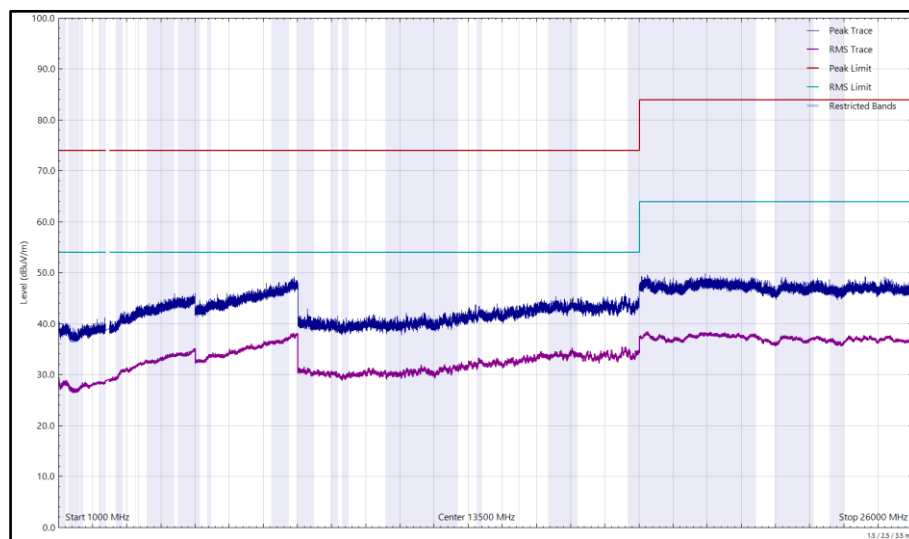
Figure 146 - 2402 MHz (CH37), LE1M, iPA, Core 0 + Core 1, 1 GHz to 26 GHz, Horizontal
