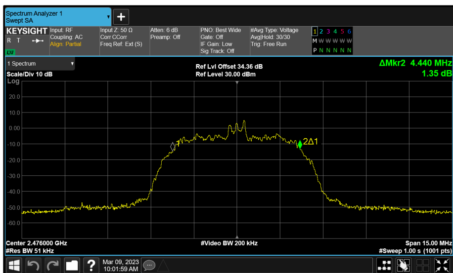
Figure 105 - Core 0 (B) 2476 MHz (CH74) 99% Bandwidth
