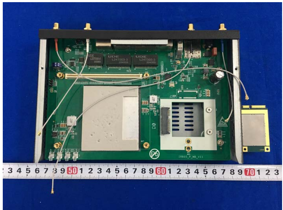
Uncovered View 4
