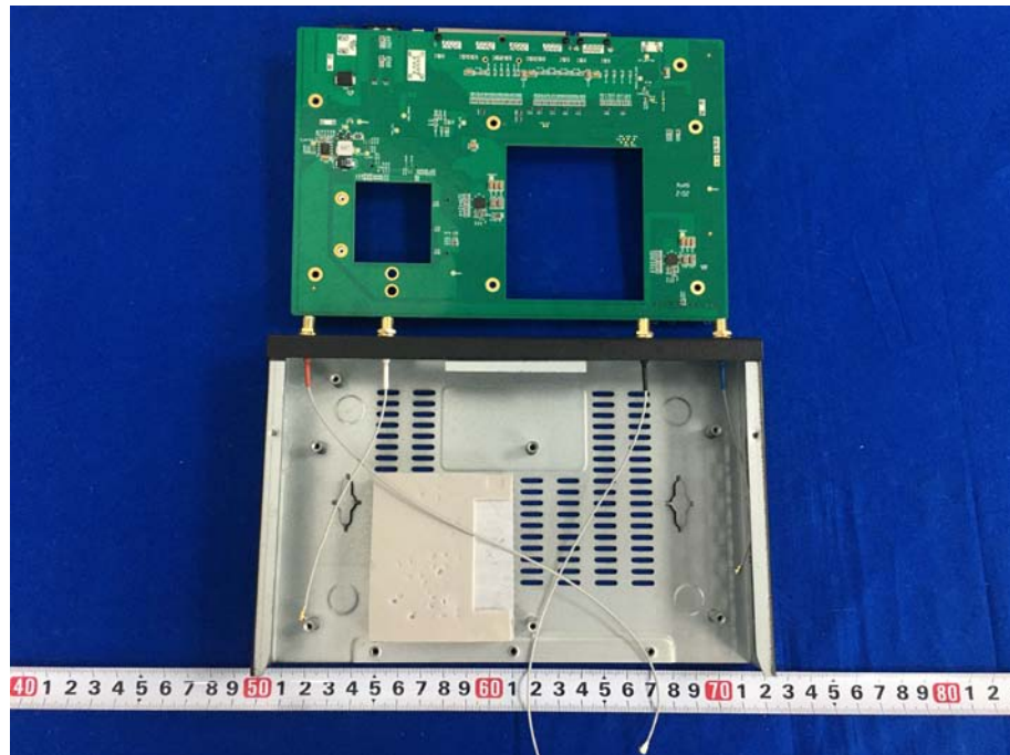
Uncovered View 5
