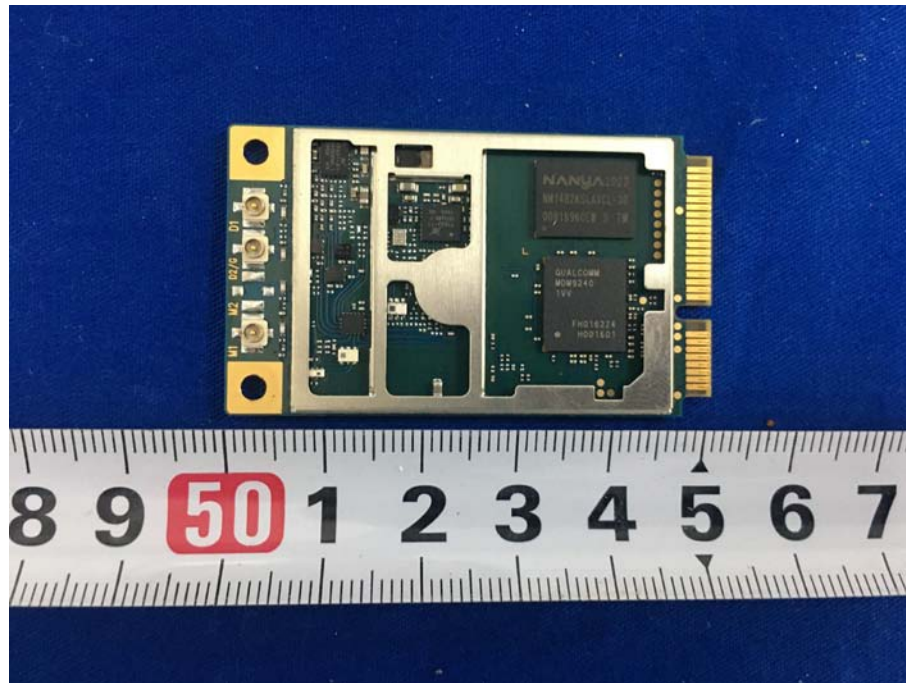
LTE Module Top Shielding off View
