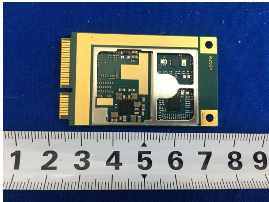
LTE Module Bottom Shielding off View
