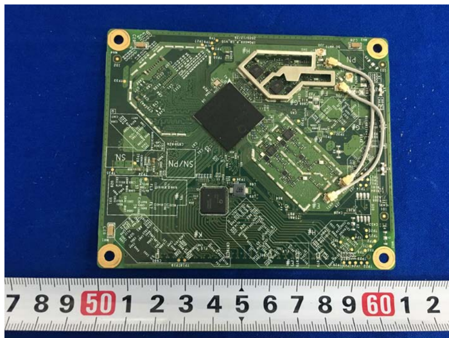
Wi-Fi Module Shielding off View
