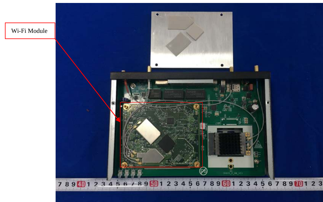
Uncovered View 2
