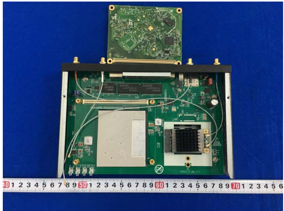
Uncovered View 3
