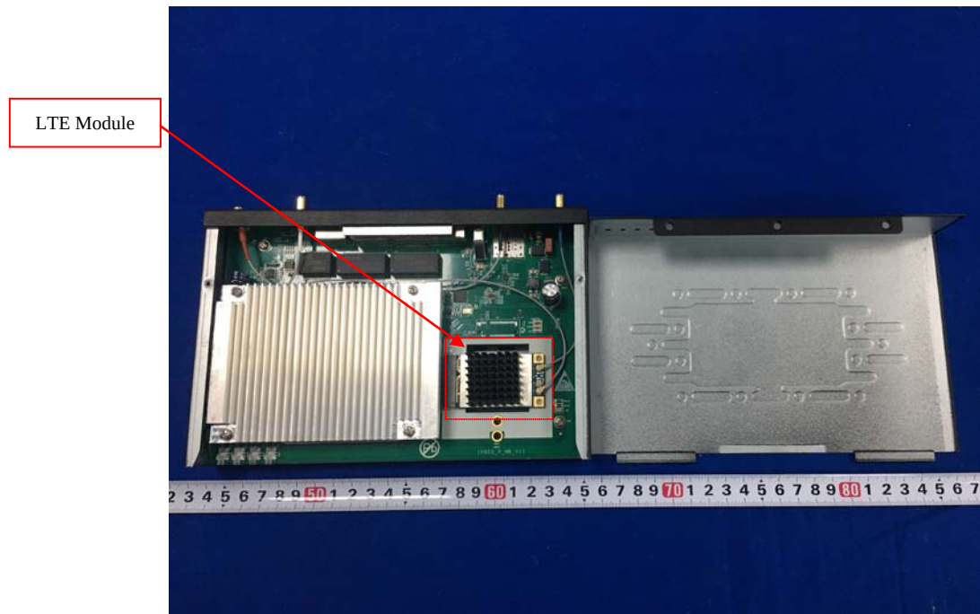
Uncovered View 1
