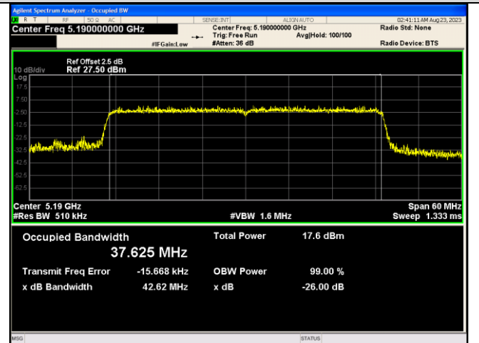
IEEE 802.11ax_Channel 38_40MHz_Antenna 1_RU&amp;Index 484RU65
