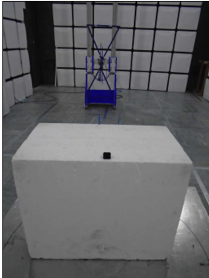
Figure 3 – Radiated Emissions 30 MHz to 1 GHz – Z Axis
