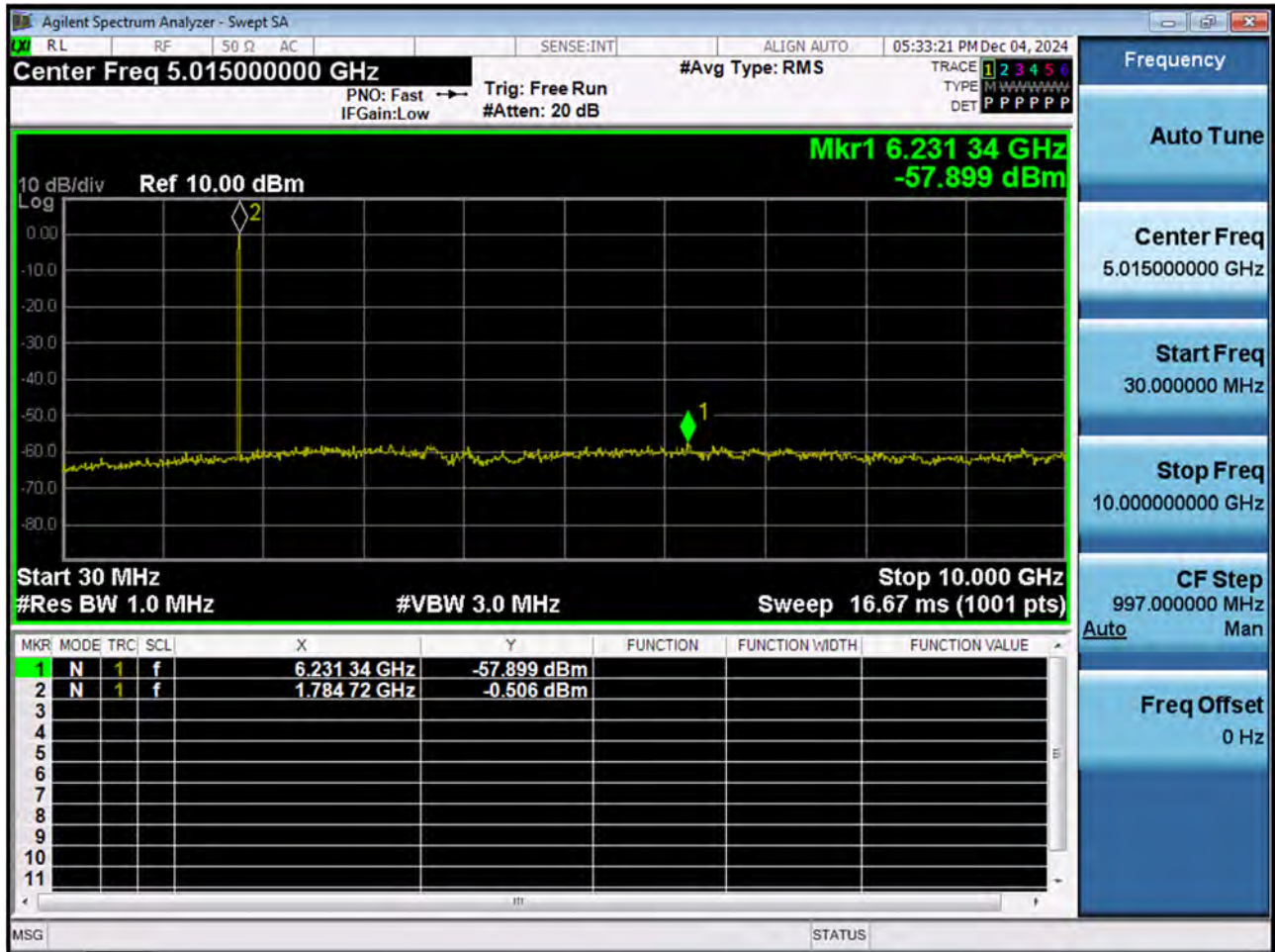
LTE B66_5 M_Conducted Spurious(30 M-10 G)_High_QPSK_1RB
