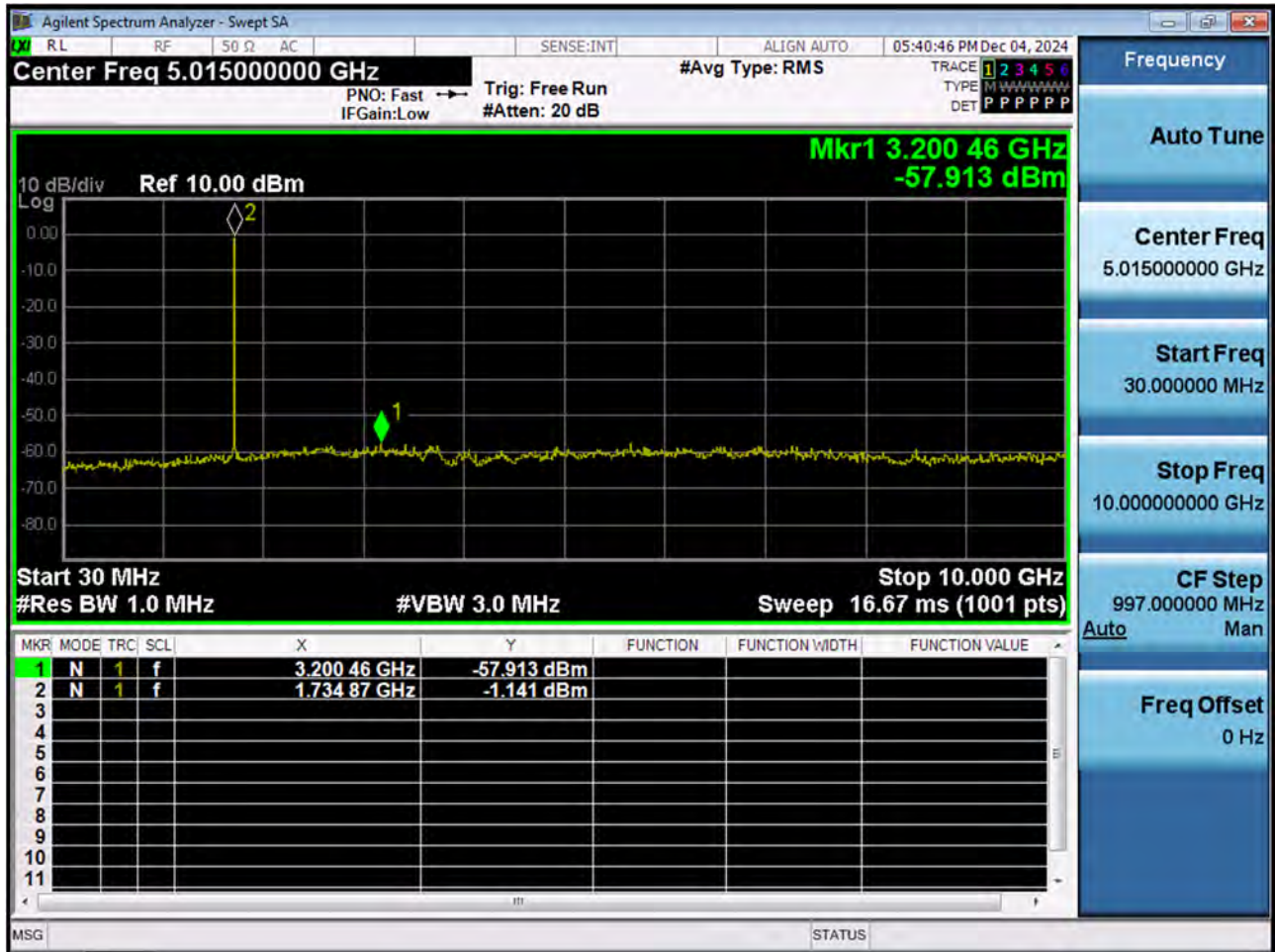
LTE B66_20 M_Conducted Spurious(30 M-10 G)_Mid_QPSK_1RB
