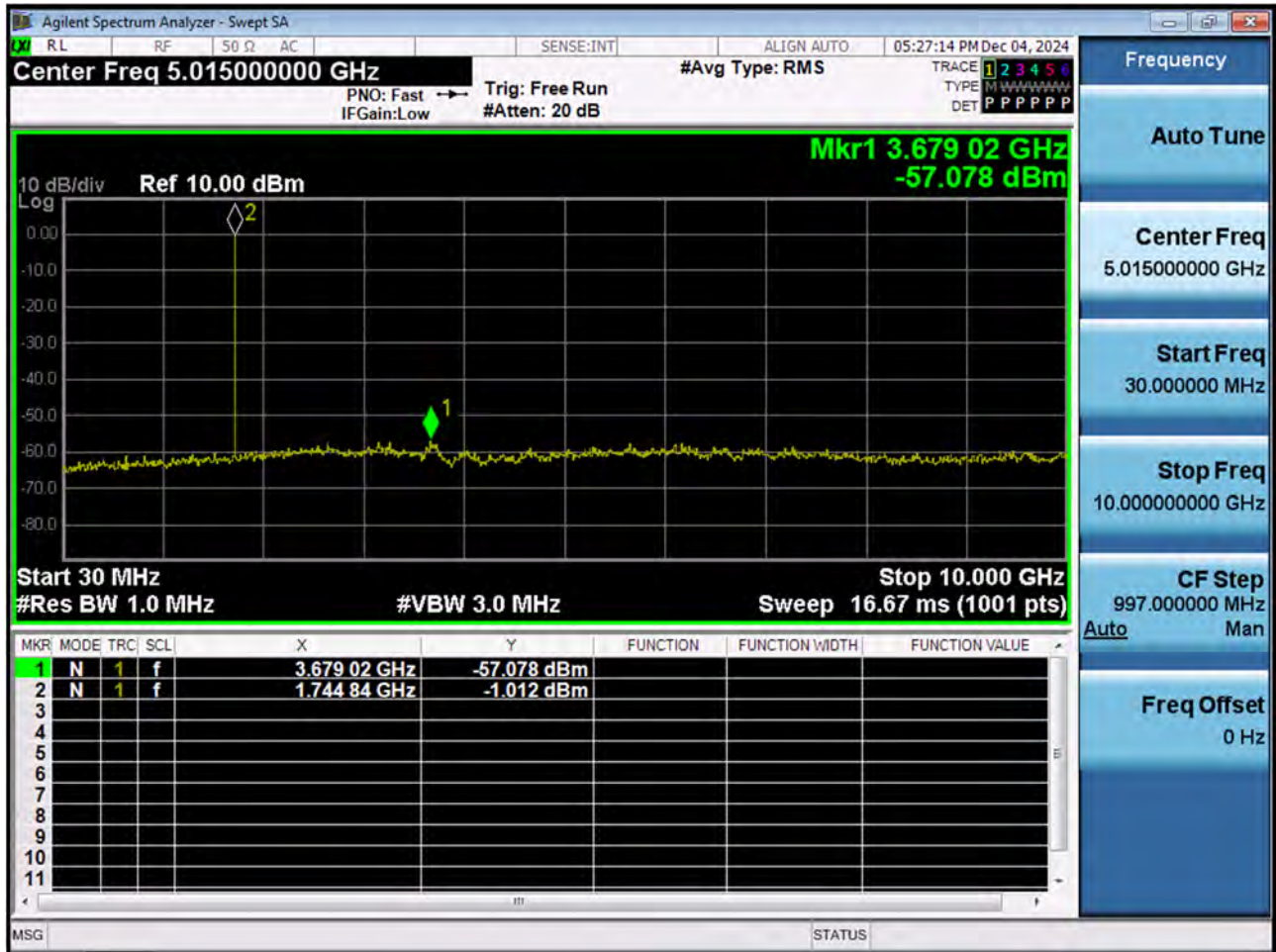
LTE B66_1.4M_Conducted Spurious(30 M-10 G)_Mid_QPSK_1RB
