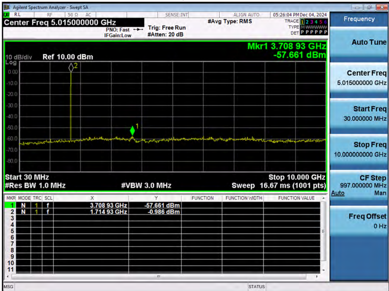
LTE B66_1.4M_Conducted Spurious(30 M-10 G)_Low_QPSK_1RB
