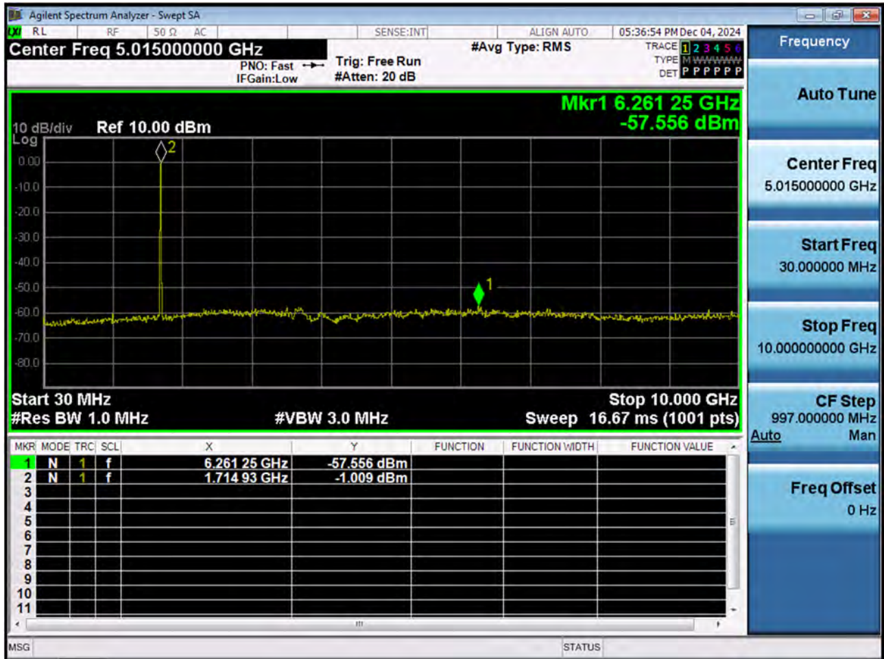
LTE B66_15 M_Conducted Spurious(30 M-10 G)_Low_QPSK_1RB
