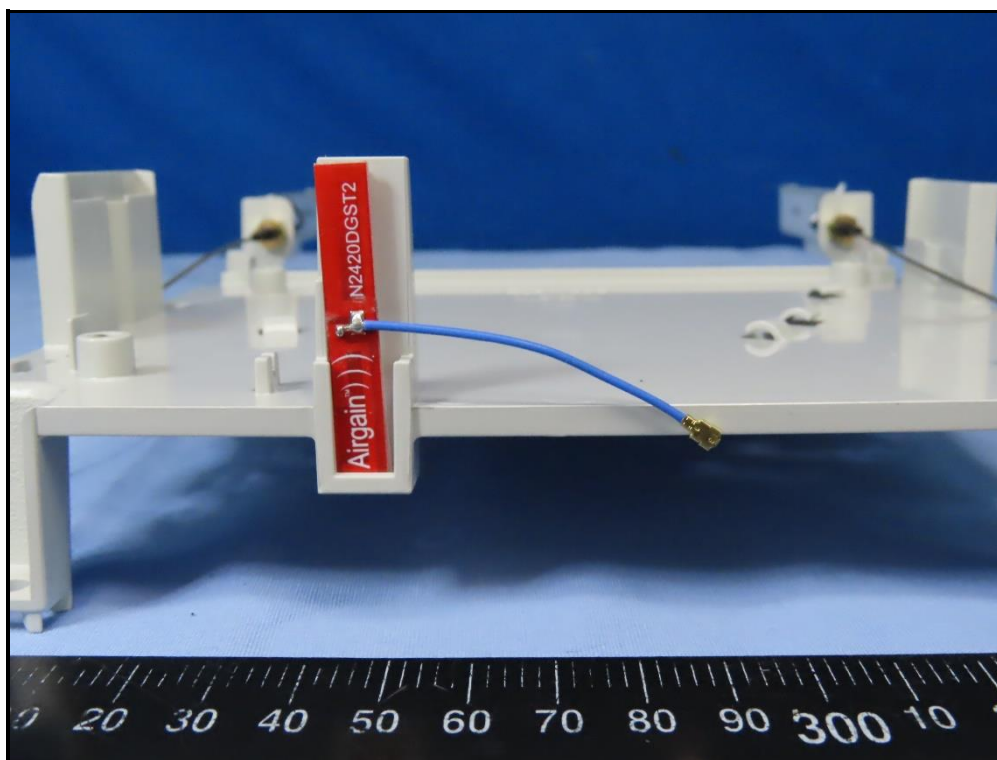
Ant No.2 (Brand: airgain, Model: 65-031-212003B)
