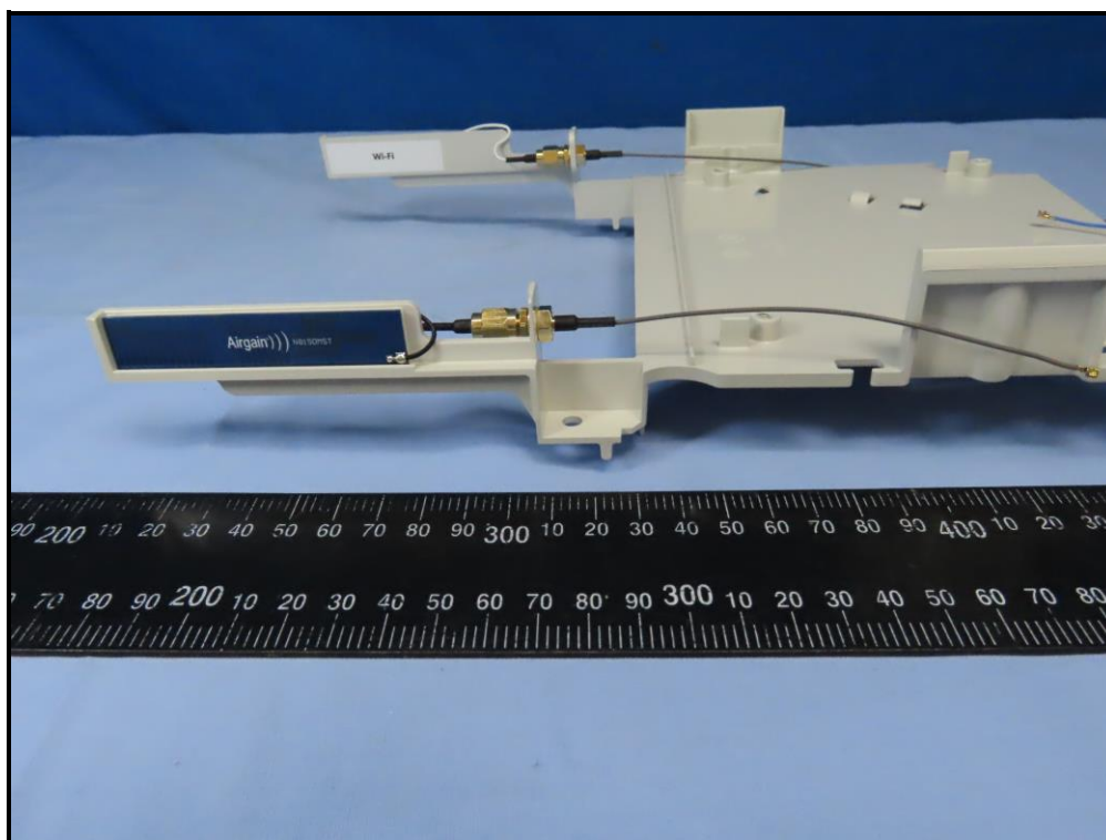
Ant No.3 (Brand: airgain, Model: 65-031-212001B)
