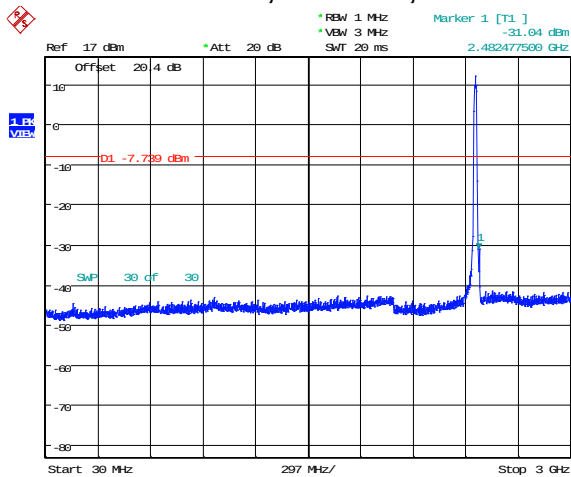
Figure 4-41: Spurious Conducted RF Emissions 802.11n, Channel 6, MCS 0
