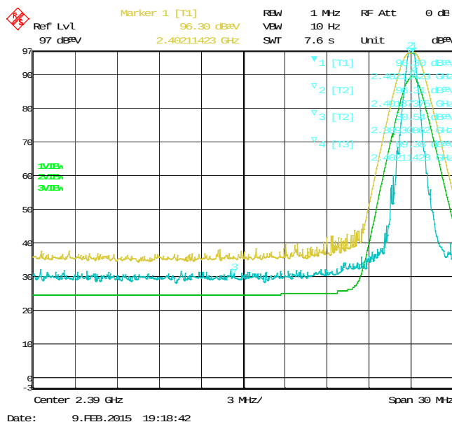
Figure 2-2: Band-Edge Compliance of RF Rad. Emissions. Bluetooth, Single freq., Static PBRS, DH5, Channel 0, Pol: H
