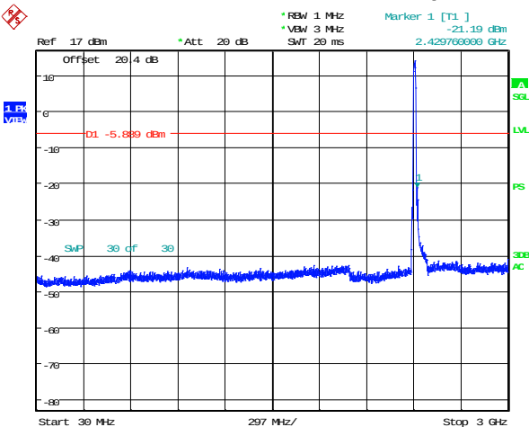
Figure 4-35 : Spurious Conducted RF Emissions 802.11b, Channel 6, 1 Mbps
