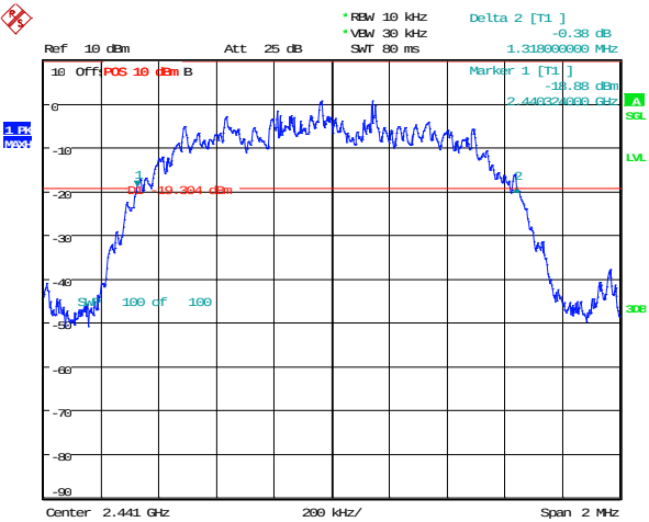
Figure 3-5: 20 dB Bandwidth Single freq., Static PBRS, 2-DH5
