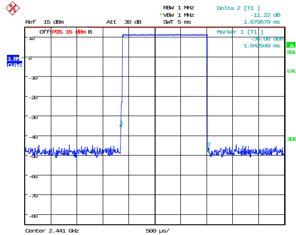
Figure 3-21: Time of Occupancy (Dwell Time) Freq. Hopping, Static PBRS, DH3
