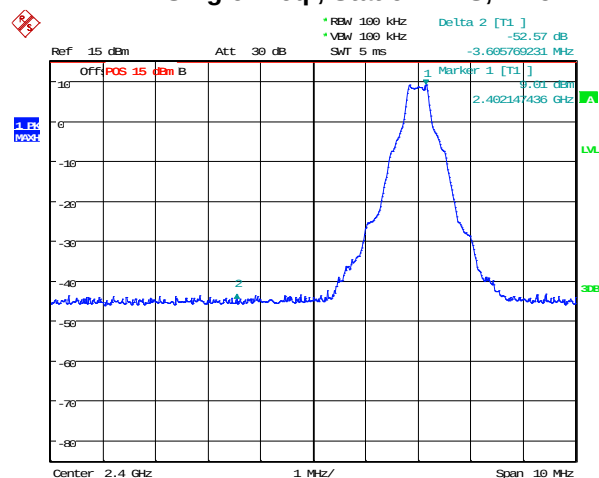
Figure 3-26: Band Edge Compliance Single Freq., Static PBRs, DH5
