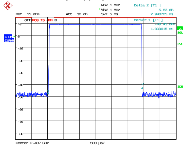
Figure 3-23: Time of Occupancy (Dwell Time) Freq. Hopping, Static PBRS, DH5
