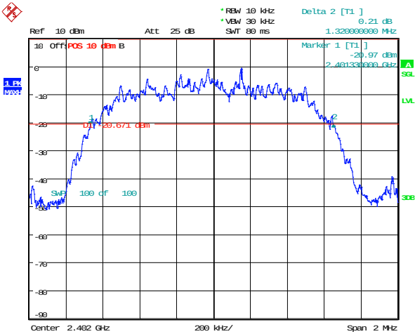
Figure 3-4: 20 dB Bandwidth Single freq., Static PBRS, 2-DH5
