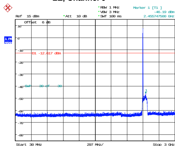
Figure 3-58: Spurious Conducted RF Emissions LE, Channel 0
