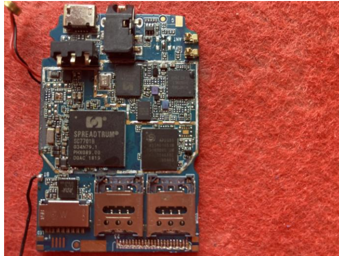
Internal photograph of EUT
