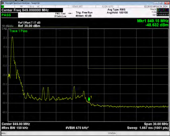
Band26(824-849) QPSK BW=15MHz Channel=26965 RB Size=1 Position=#Max Extended
