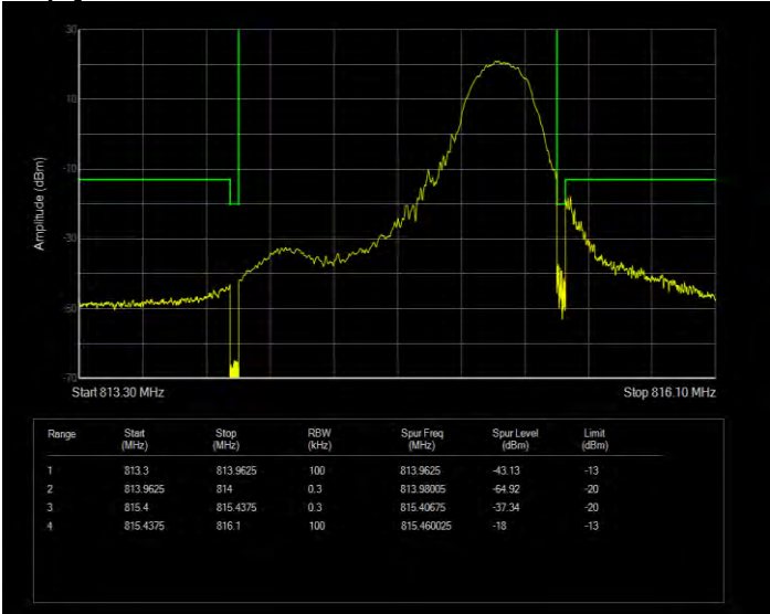
Band26(814-824) QPSK BW=1.4MHz Channel=26697 RB Size=6 Position=#0 Extended
