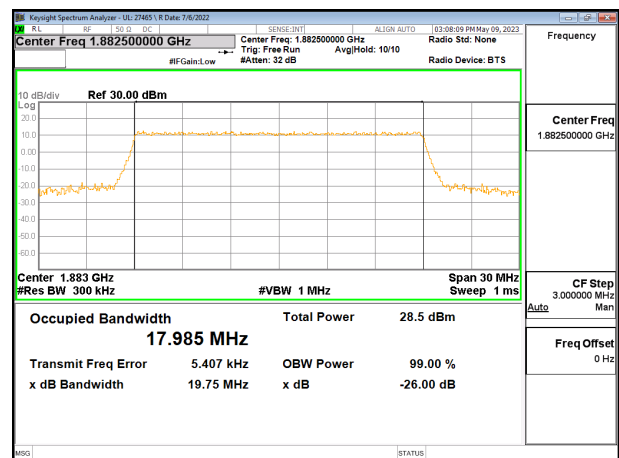
LTE25 20MHz 64QAM MID Ch RB50-24
