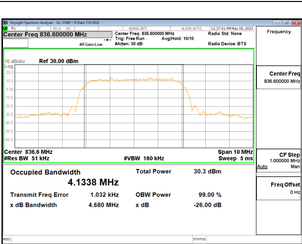
BAND 5 HSDPA MID Channel
