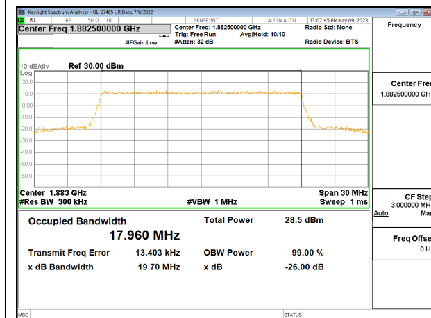
LTE25 20MHz 16QAM MID Ch RB50-24
