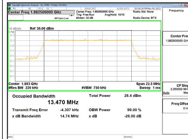
LTE25 15MHz 64QAM MID Ch RB75-0
