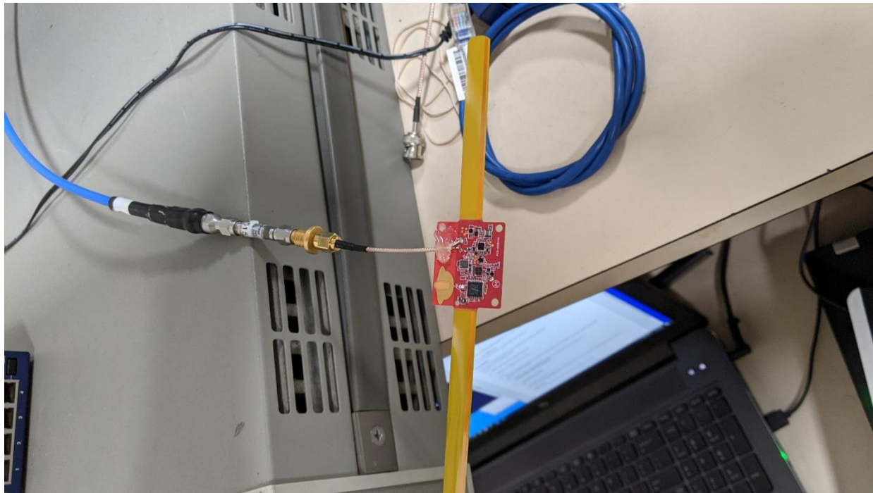
Conducted Test
