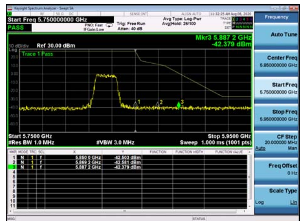
U-NII-3 ,Plot 1,Band Edge-802.11ac(80 MHz),5775MHz,Ant1 ( Right )
