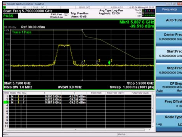
U-NII-3 ,Plot 1,Band Edge-802.11a(20 MHz),5825MHz,Ant1
