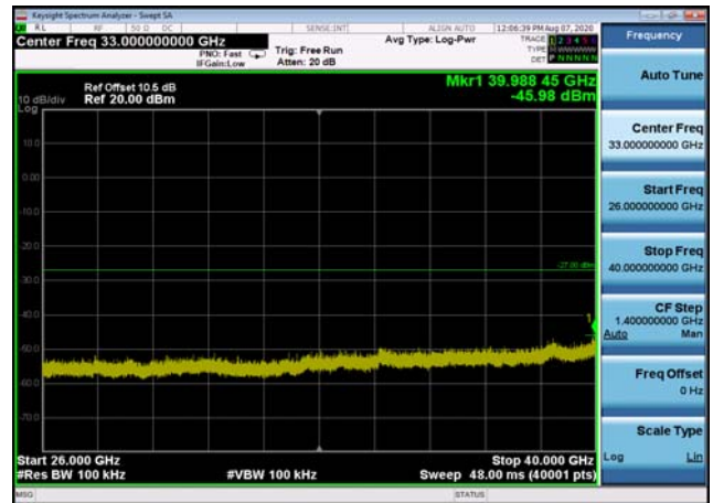
U-NII-3 ,Plot 2,26000MHz~40000MHz-802 .11a(20MHz),5825MHz,Ant1
