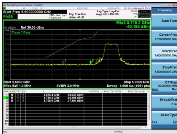
U-NII-3 ,Plot 1,Band Edge-802.11n(20M Hz),5745MHz,Ant1
