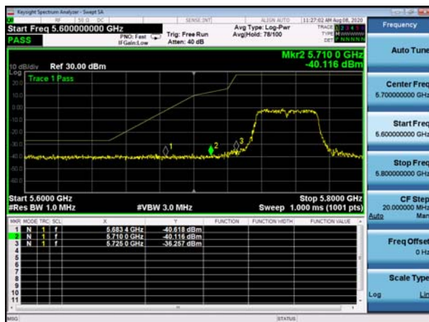
U-NII-3 ,Plot 1,Band Edge-802.11ac(80 MHz),5775MHz,Ant1 ( Left )
