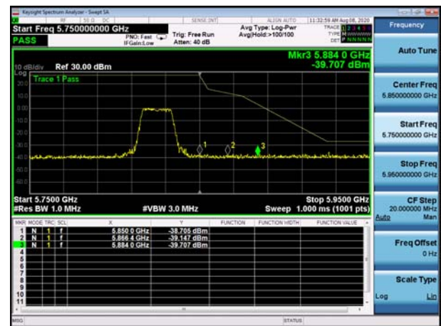
U-NII-3 ,Plot 1,Band Edge-802.11n(20M Hz),5825MHz,Ant1
