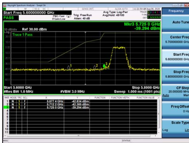
U-NII-3 ,Plot 1,Band Edge-802.11a(20M Hz),5745MHz,Ant1
