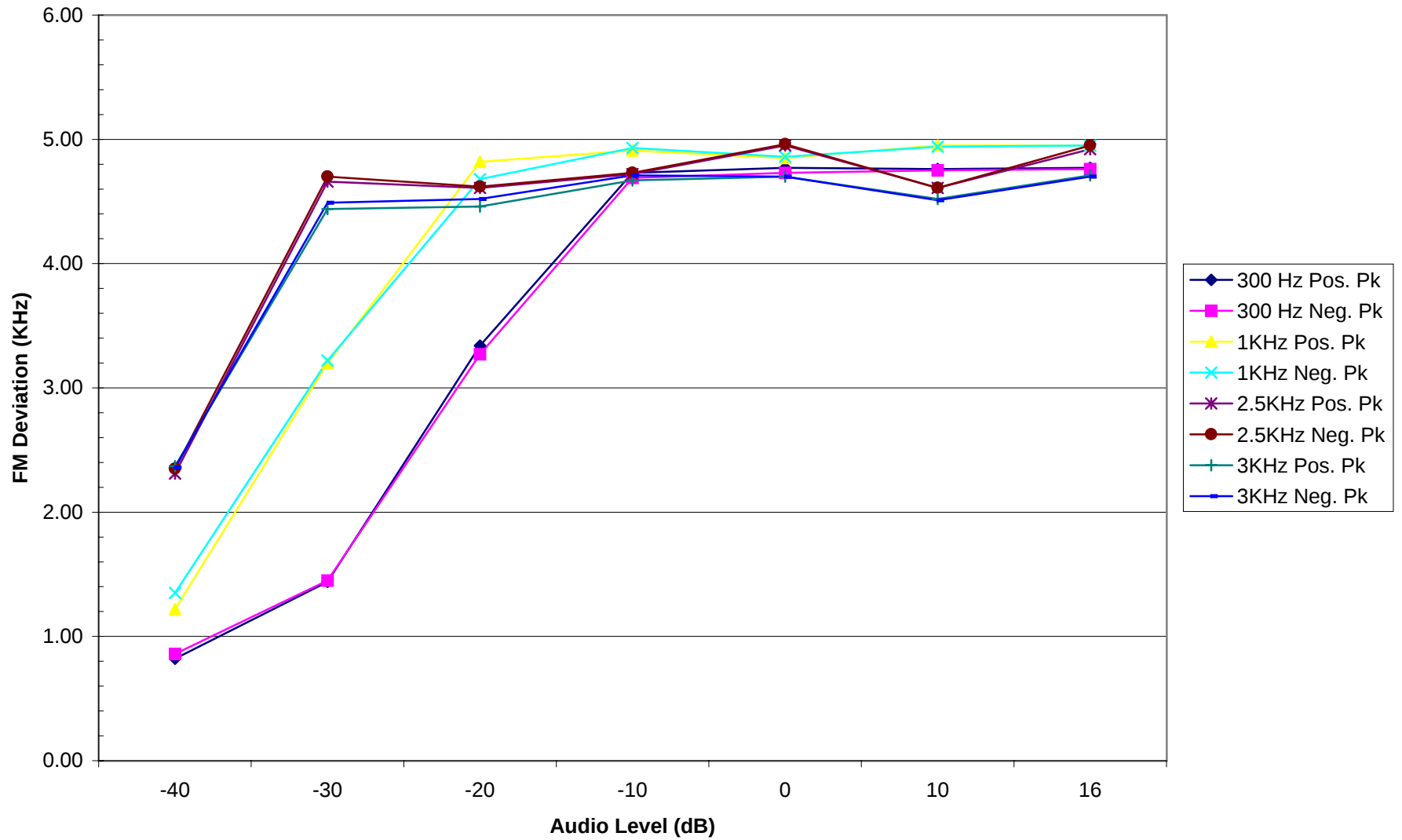
Modulation Limiting Neg/Pos Peaks @156MHz
