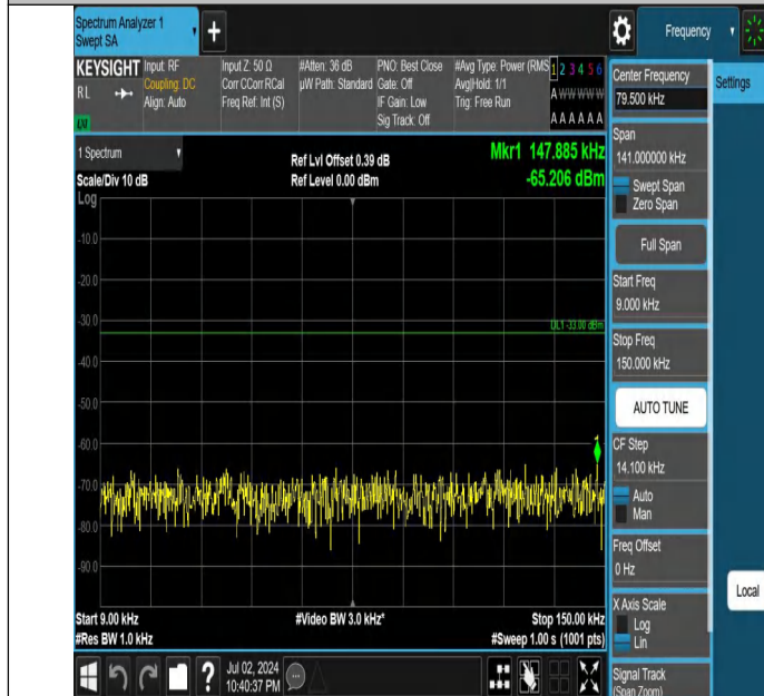
Band5-3MHz-QPSK-20415-1RB#0-0.009~0.15-PASS
