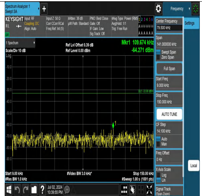
Band5-1.4MHz-QPSK-20643-1RB#5-0.009~0.15-PASS
