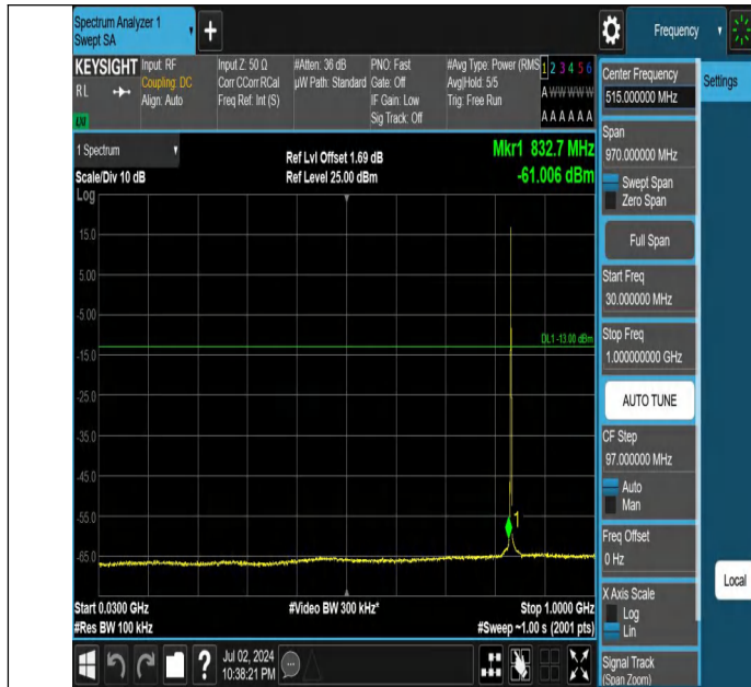
Band5-1.4MHz-QPSK-20525-1RB#0-30~1000-PASS
