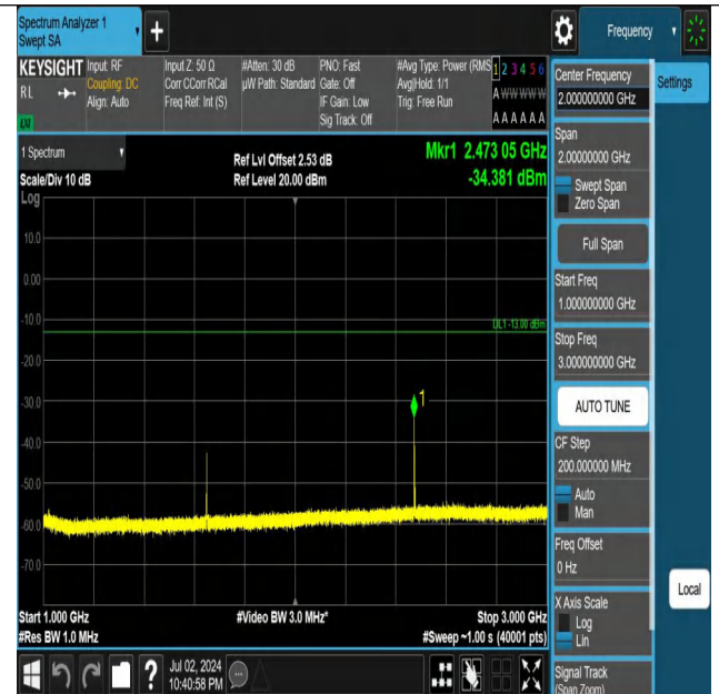
Band5-3MHz-QPSK-20415-1RB#0-1000~3000-PASS
