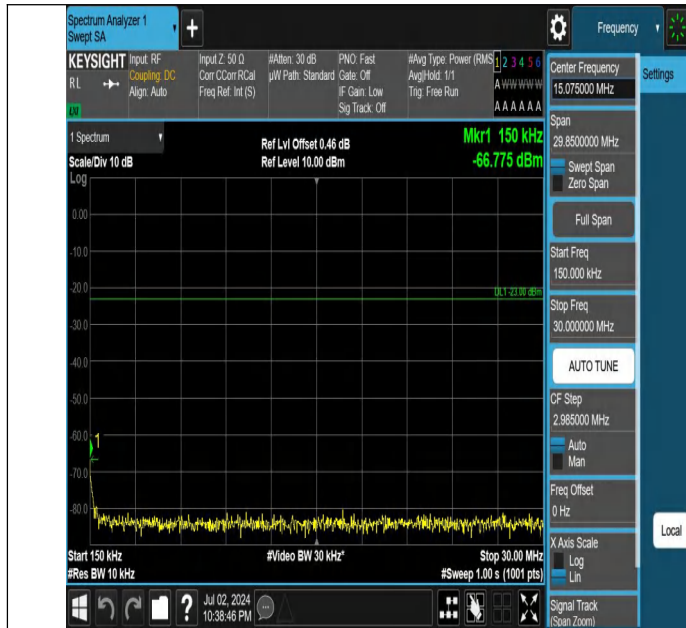
Band5-1.4MHz-QPSK-20525-1RB#5-0.15~30-PASS
