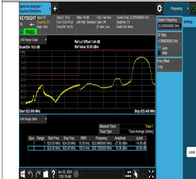
Band5-1.4MHz-QPSK-20407-1RB#5-PASS
