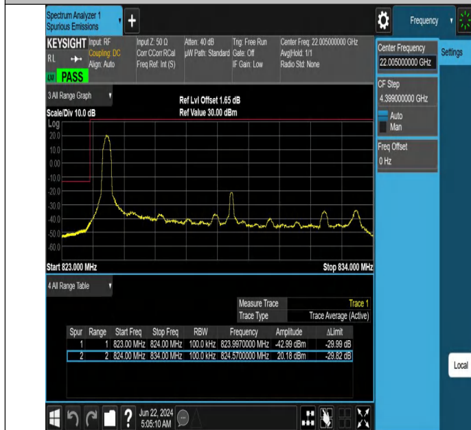
Band5-10MHz-QPSK-20450-1RB#0-PASS
