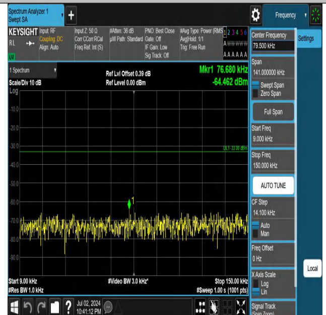
Band5-3MHz-QPSK-20415-1RB#14-0.009~0.15-PASS
