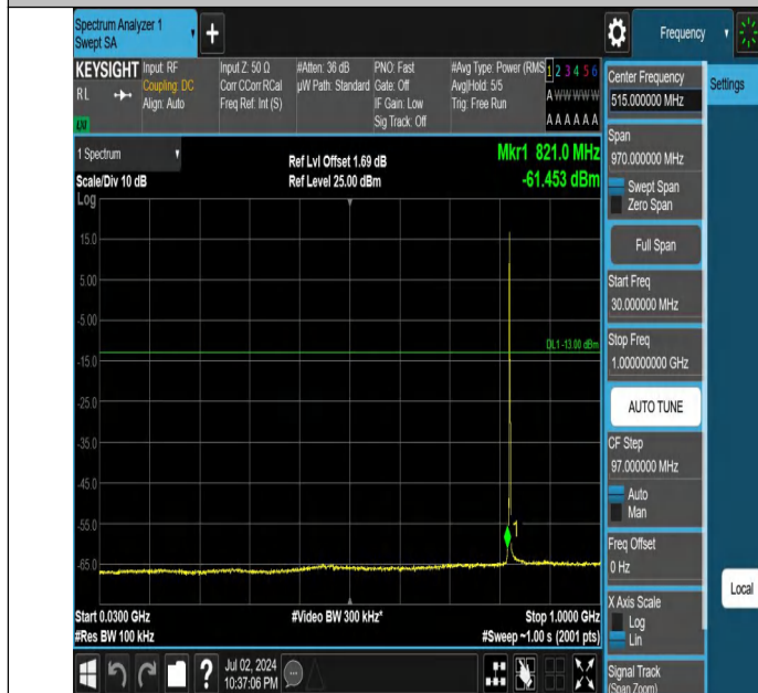
Band5-1.4MHz-QPSK-20407-1RB#0-30~1000-PASS
