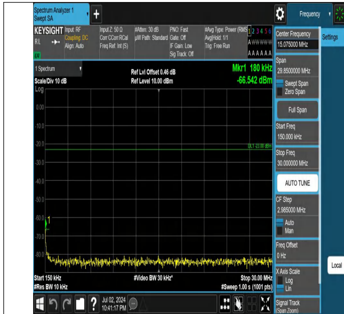
Band5-3MHz-QPSK-20415-1RB#14-0.15~30-PASS
