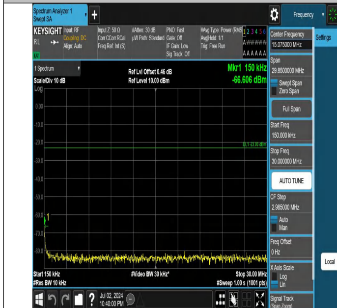
Band5-1.4MHz-QPSK-20643-1RB#5-0.15~30-PASS
