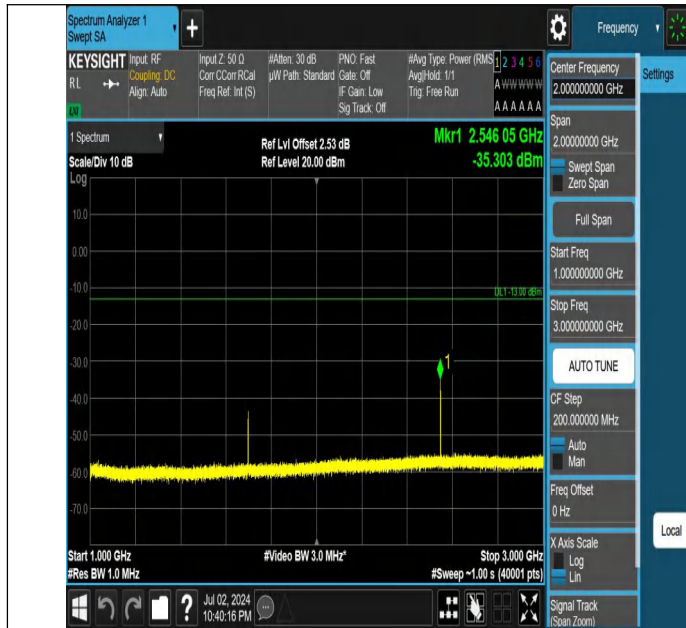
Band5-1.4MHz-QPSK-20643-1RB#5-1000~3000-PASS
