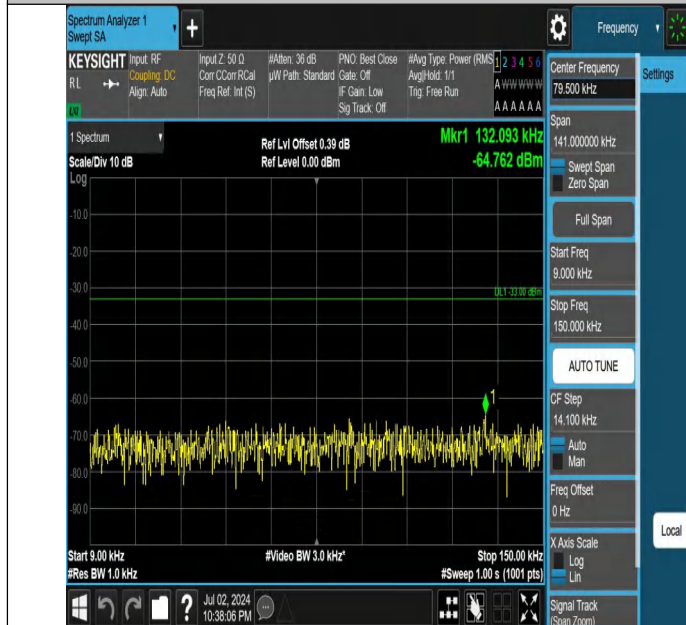
Band5-1.4MHz-QPSK-20525-1RB#0-0.009~0.15-PASS
