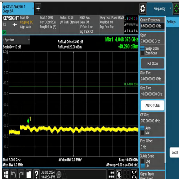
Band5-3MHz-QPSK-20415-1RB#0-3000~10000-PASS
