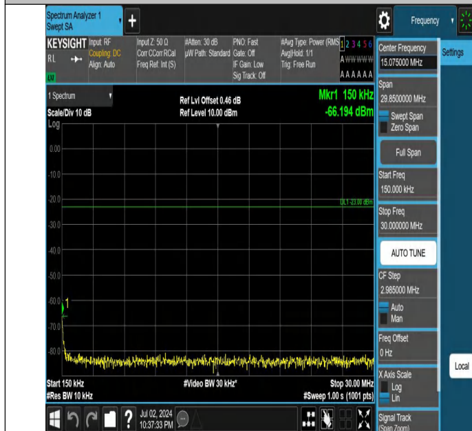
Band5-1.4MHz-QPSK-20407-1RB#5-0.15~30-PASS
