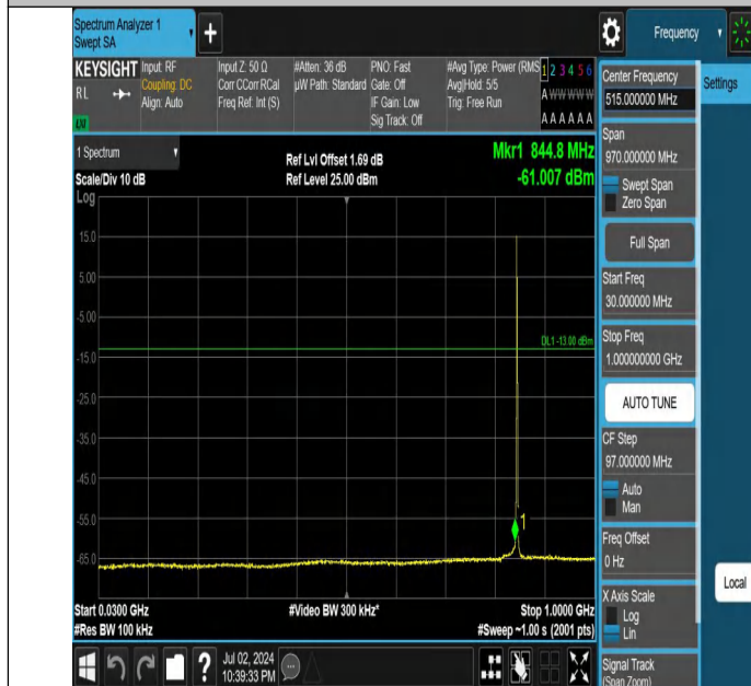
Band5-1.4MHz-QPSK-20643-1RB#0-30~1000-PASS
