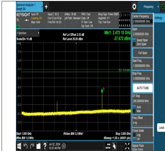
Band5-1.4MHz-QPSK-20407-1RB#5-1000~3000-PASS
