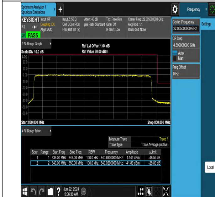
Band5-10MHz-QPSK-20600-50RB#0-PASS
