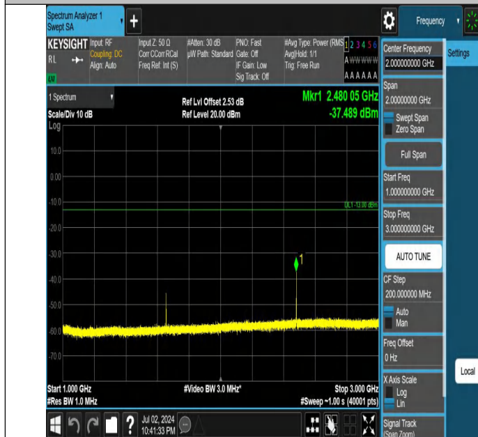
Band5-3MHz-QPSK-20415-1RB#14-1000~3000-PASS
