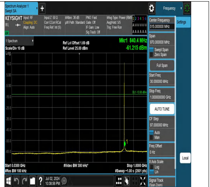
Band5-1.4MHz-QPSK-20525-1RB#5-30~1000-PASS
