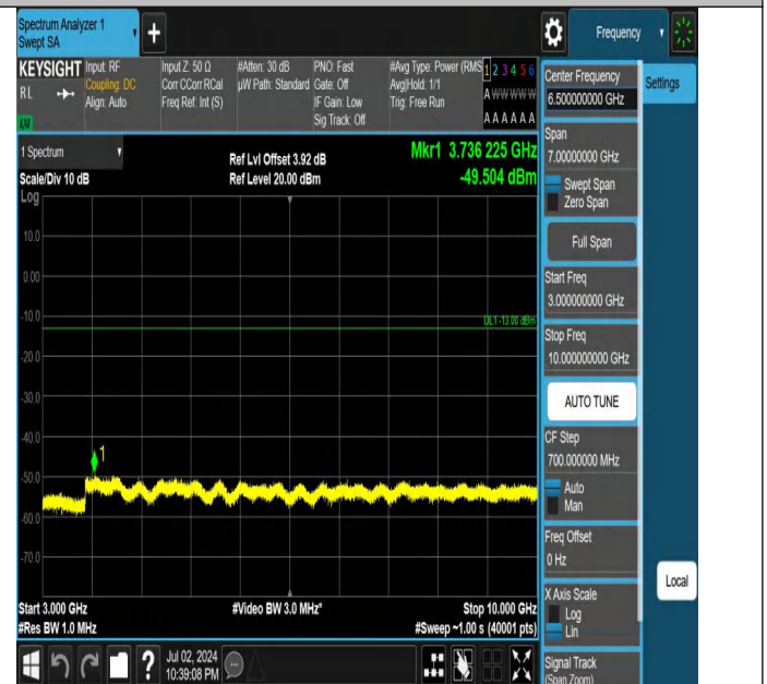
Band5-1.4MHz-QPSK-20525-1RB#5-3000~10000-PASS
