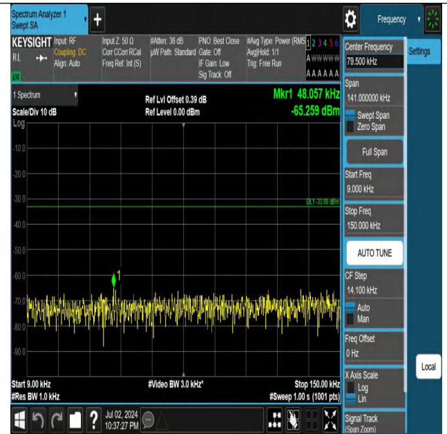
Band5-1.4MHz-QPSK-20407-1RB#5-0.009~0.15-PASS
