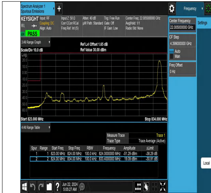
Band5-10MHz-QPSK-20450-1RB#49-PASS
