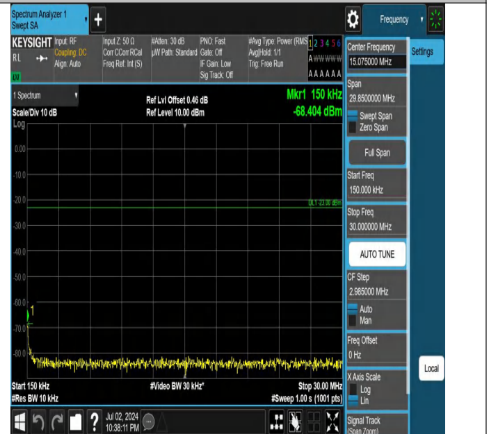
Band5-1.4MHz-QPSK-20525-1RB#0-0.15~30-PASS
