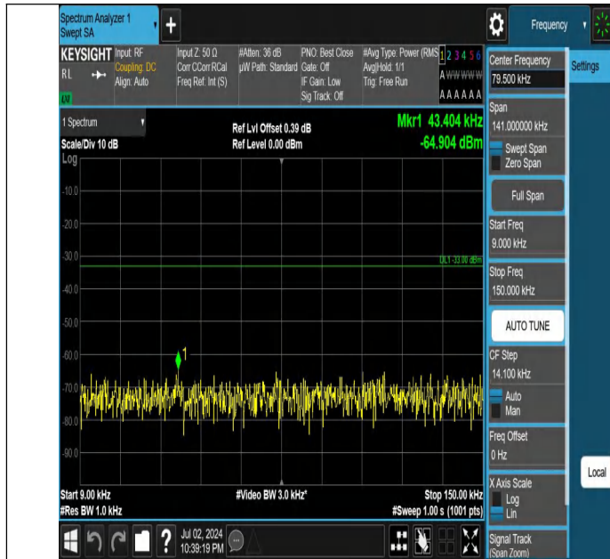
Band5-1.4MHz-QPSK-20643-1RB#0-0.009~0.15-PASS
