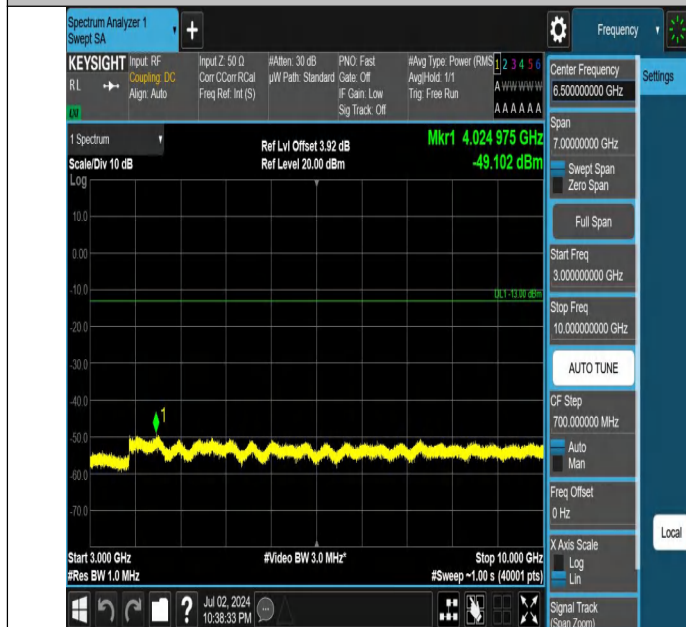
Band5-1.4MHz-QPSK-20525-1RB#0-3000~10000-PASS
