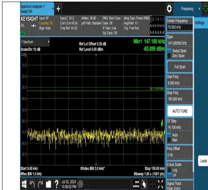
Band5-1.4MHz-QPSK-20407-1RB#0-0.009~0.15-PASS
