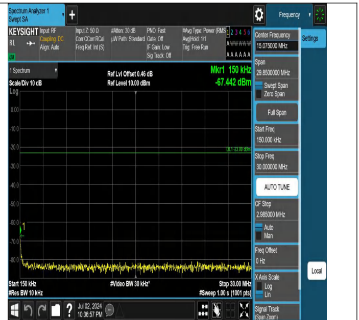
Band5-1.4MHz-QPSK-20407-1RB#0-0.15~30-PASS
