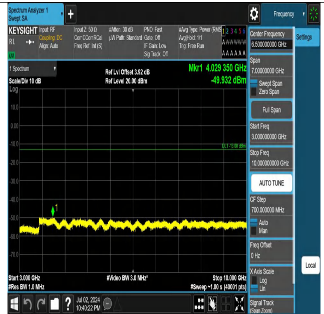
Band5-1.4MHz-QPSK-20643-1RB#5-3000~10000-PASS
