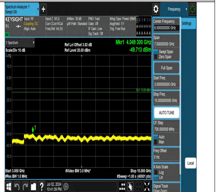
Band5-3MHz-QPSK-20415-1RB#14-3000~10000-PASS
