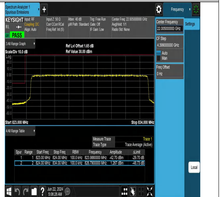
Band5-10MHz-QPSK-20450-50RB#0-PASS
