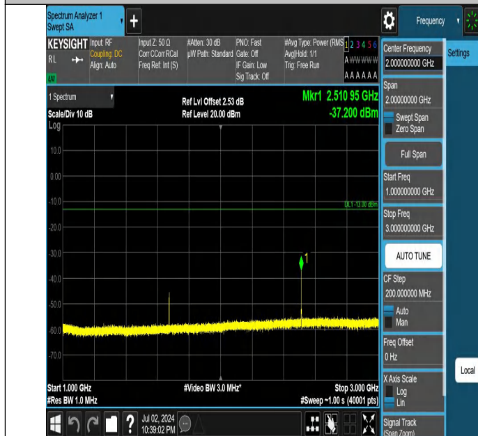
Band5-1.4MHz-QPSK-20525-1RB#5-1000~3000-PASS
