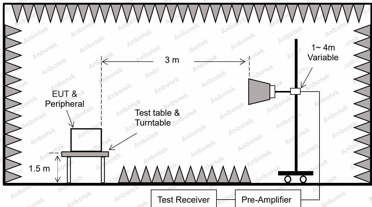
Figure 3. Above 1 GHz
