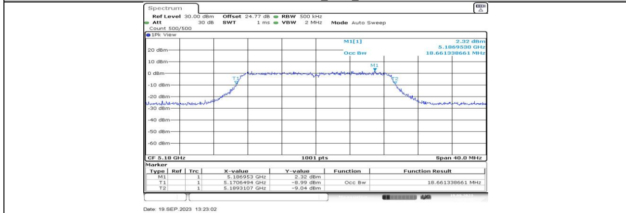
11AC20MIMO_Ant4_5180
