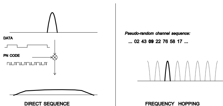
Forms of spread spectrum - direct sequence and frequency hopping
