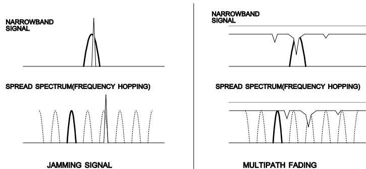
Narrow-band versus spread-spectrum transmission
