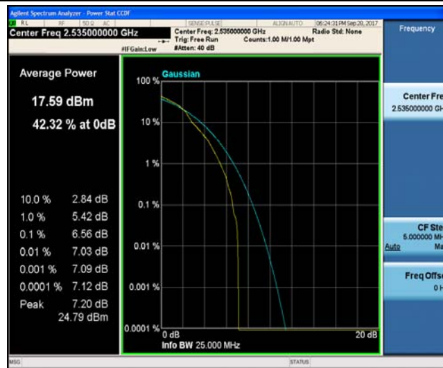
Band7_15MHz_QPSK_21100_75RB#0_6.28_13_PASS
