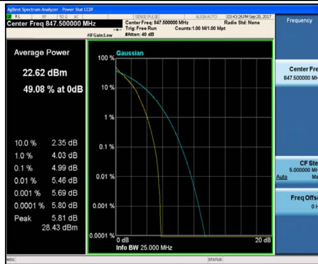
Band5_3MHz_16QAM_20635_15RB#0_5.80_13_PASS
