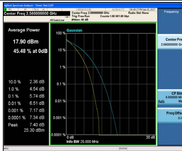
Band7_20MHz_16QAM_21350_100RB#0_6.51_13_PASS
