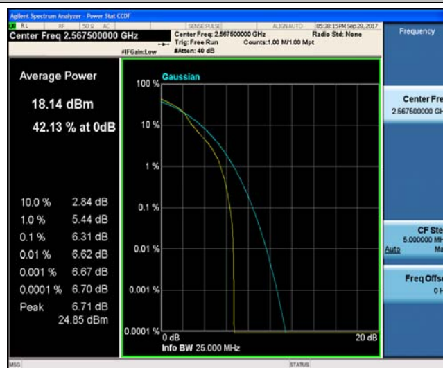
Band7_5MHz_QPSK_21425_25RB#0_5.97_13_PASS
