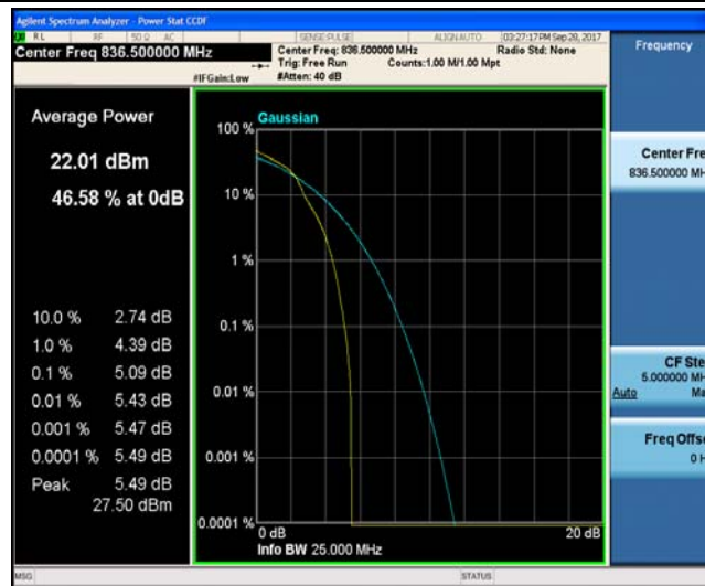
Band5_1.4MHz_QPSK_20525_6RB#0_4.70_13_PASS
