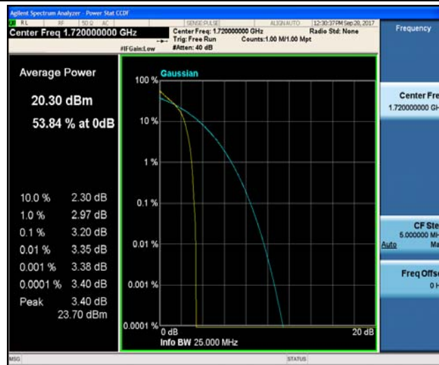
Band4_20MHz_16QAM_20050_1RB#0_4.10_13_PASS
