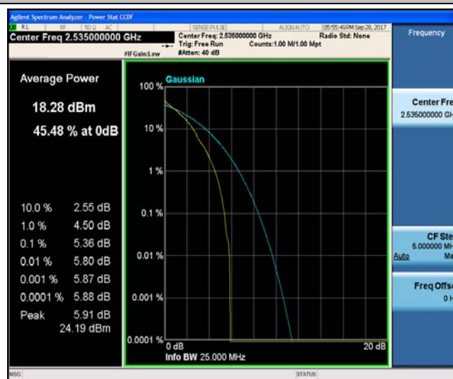
Band7_10MHz_16QAM_21100_1RB#0_6.34_13_PASS
