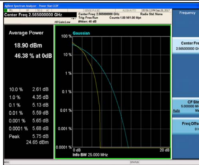
Band7_10MHz_16QAM_21400_1RB#0_6.11_13_PASS
