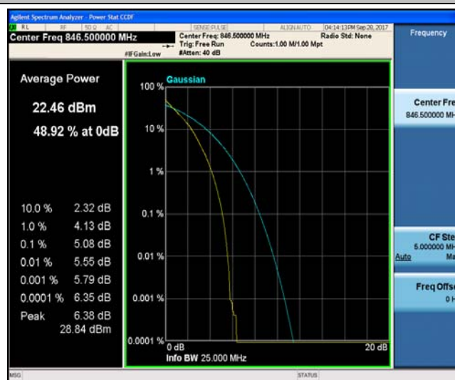
Band5_5MHz_16QAM_20625_25RB#0_5.85_13_PASS
