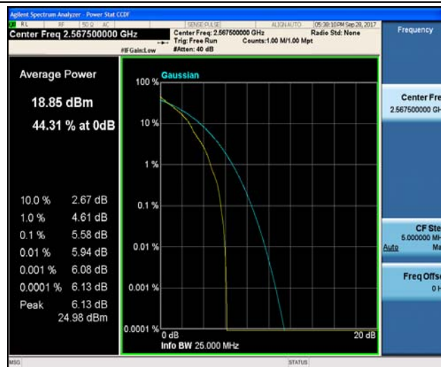
Band7_5MHz_16QAM_21425_1RB#0_6.31_13_PASS
