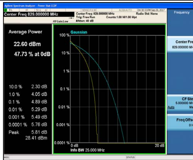
Band5_10MHz_16QAM_20450_50RB#0_5.68_13_PASS
