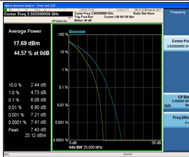
Band7_5MHz_16QAM_20775_25RB#0_6.83_13_PASS
