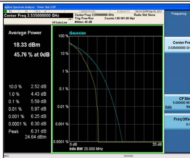
Band7_15MHz_16QAM_21100_1RB#0_6.56_13_PASS
