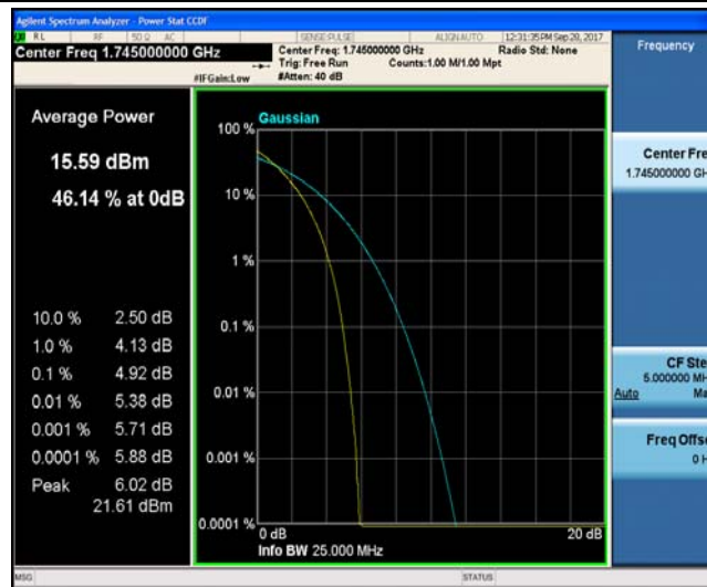
Band4_20MHz_16QAM_20300_100RB#0_5.76_13_PASS
