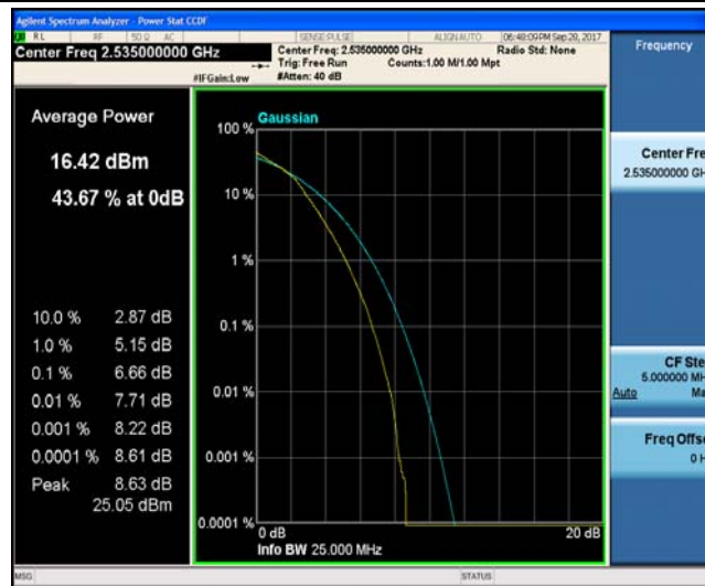
Band7_20MHz_QPSK_21100_1RB#0_5.59_13_PASS
