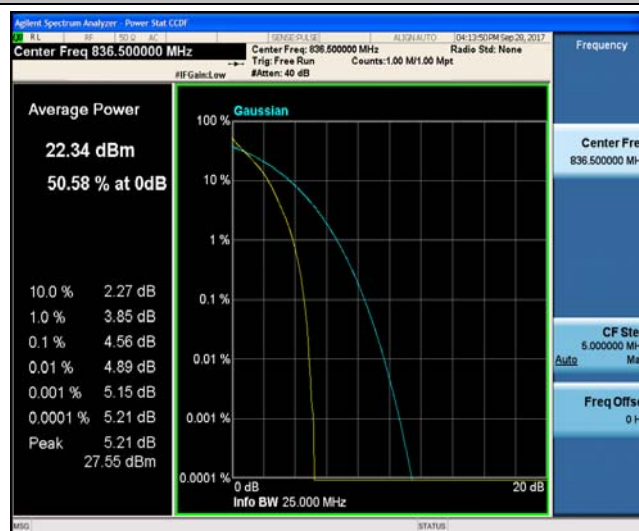
Band5_5MHz_16QAM_20525_25RB#0_5.44_13_PASS
