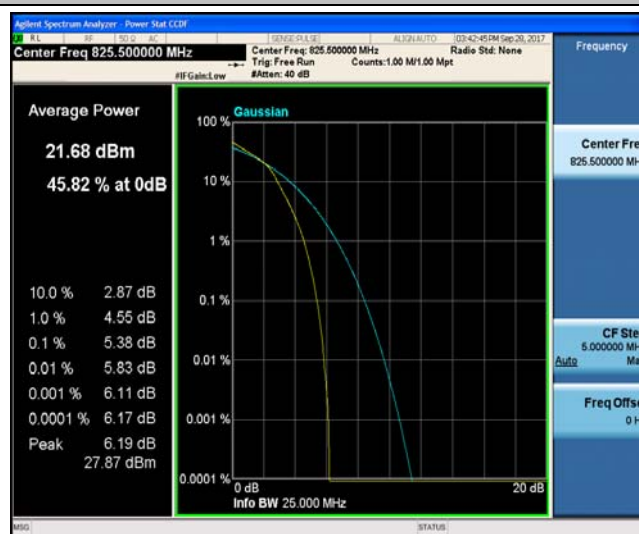
Band5_3MHz_QPSK_20415_1RB#0_3.57_13_PASS
