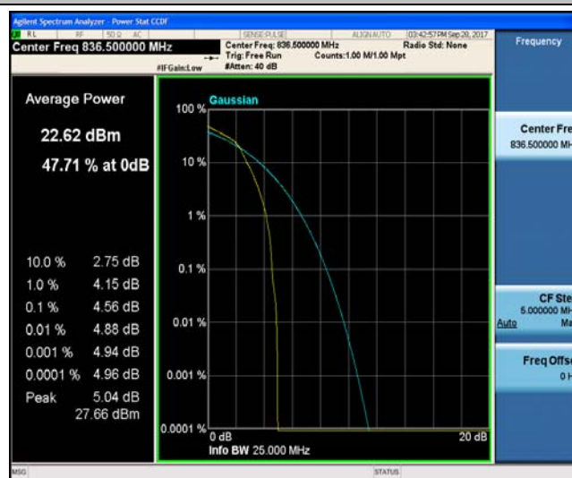
Band5_3MHz_QPSK_20635_15RB#0_4.99_13_PASS
