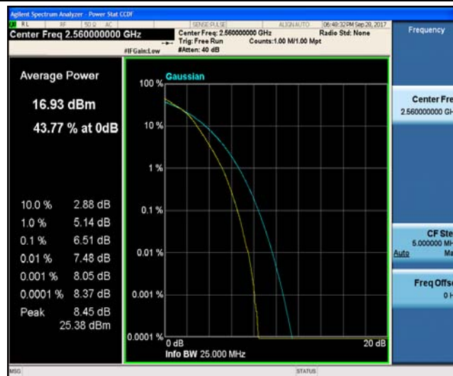
Band7_20MHz_QPSK_21350_1RB#0_5.24_13_PASS
