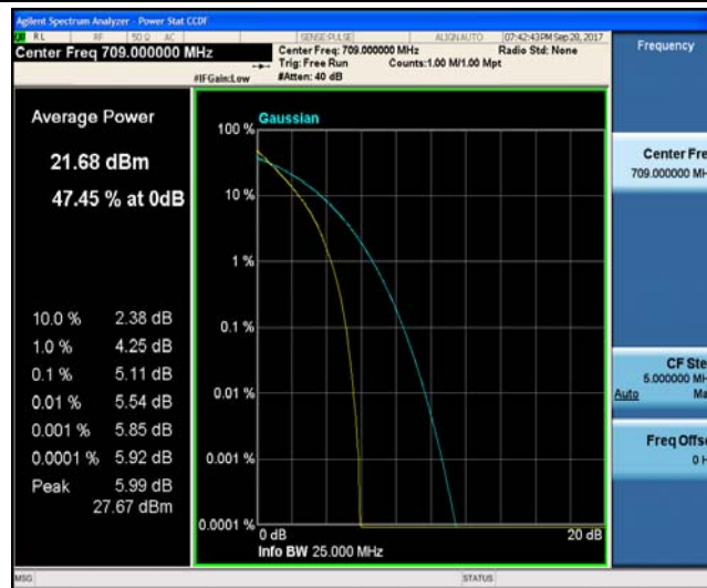
Band17_10MHz_16QAM_23780_50RB#0_5.92_13_PASS
