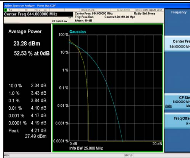
Band5_10MHz_16QAM_20600_1RB#0_4.78_13_PASS
