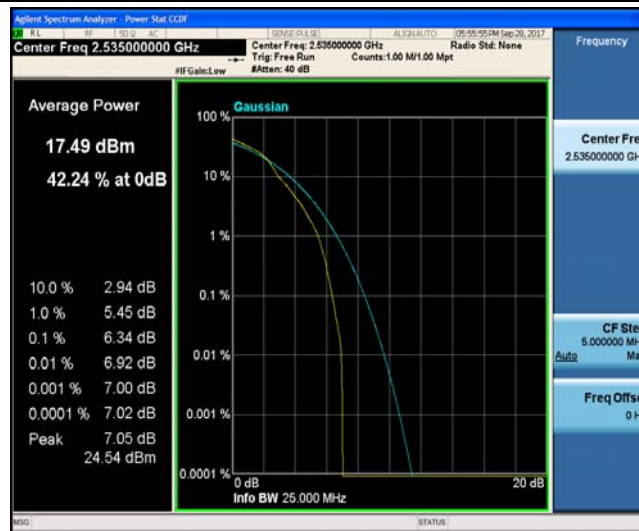
Band7_10MHz_QPSK_21100_50RB#0_6.03_13_PASS
