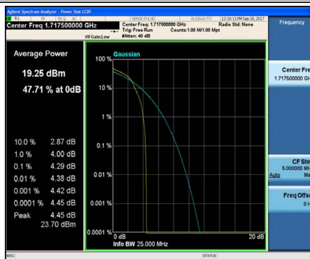
Band4_15MHz_QPSK_20025_75RB#0_5.25_13_PASS
