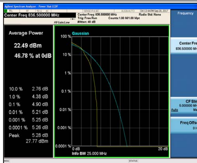
Band5_5MHz_QPSK_20525_25RB#0_4.56_13_PASS
