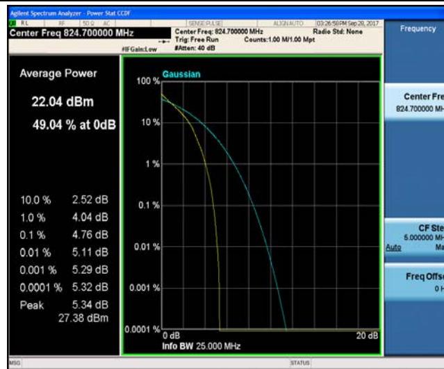
Band5_1.4MHz_16QAM_20407_6RB#0_5.66_13_PASS
