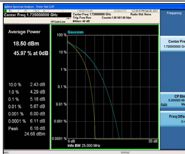
Band4_20MHz_16QAM_20050_100RB#0_6.00_13_PASS
