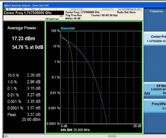
Band4_15MHz_16QAM_20325_1RB#0_4.06_13_PASS
