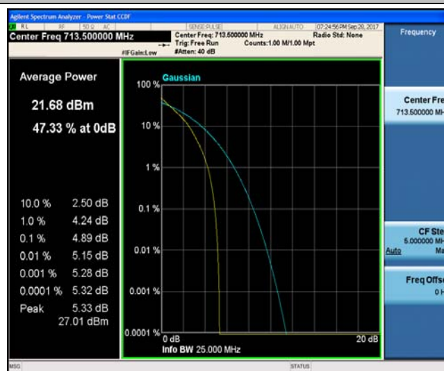
Band17_5MHz_16QAM_23825_25RB#0_5.77_13_PASS
