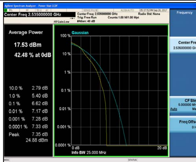
Band7_5MHz_QPSK_21100_25RB#0_6.07_13_PASS
