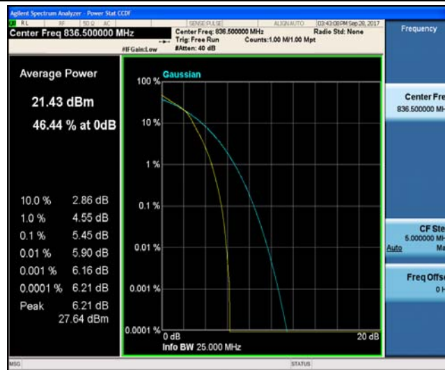
Band5_3MHz_QPSK_20525_1RB#0_3.84_13_PASS
