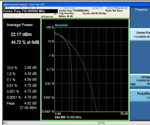
Band17_5MHz_QPSK_23790_25RB#0_4.68_13_PASS
