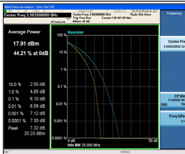
Band7_15MHz_16QAM_21375_75RB#0_6.59_13_PASS
