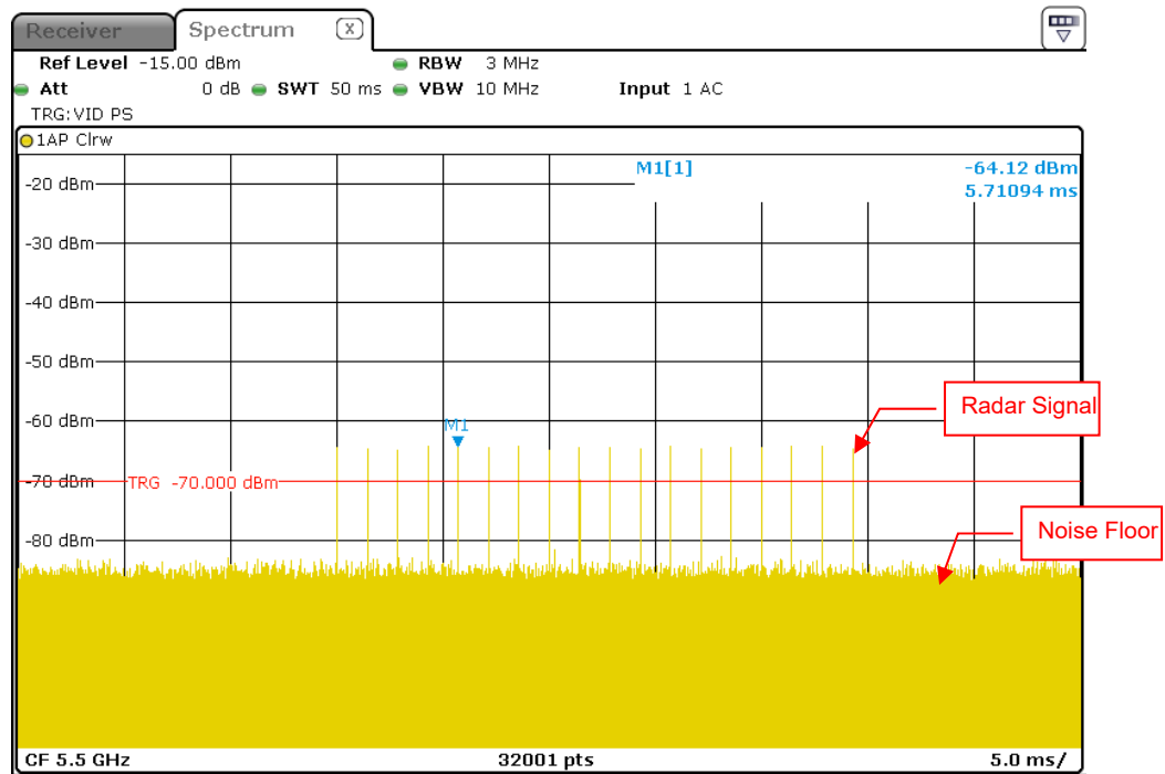
Radar Signal 0
