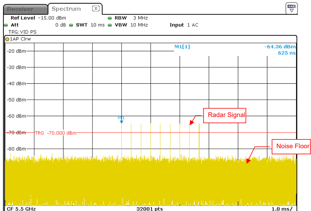
Radar Signal 6
