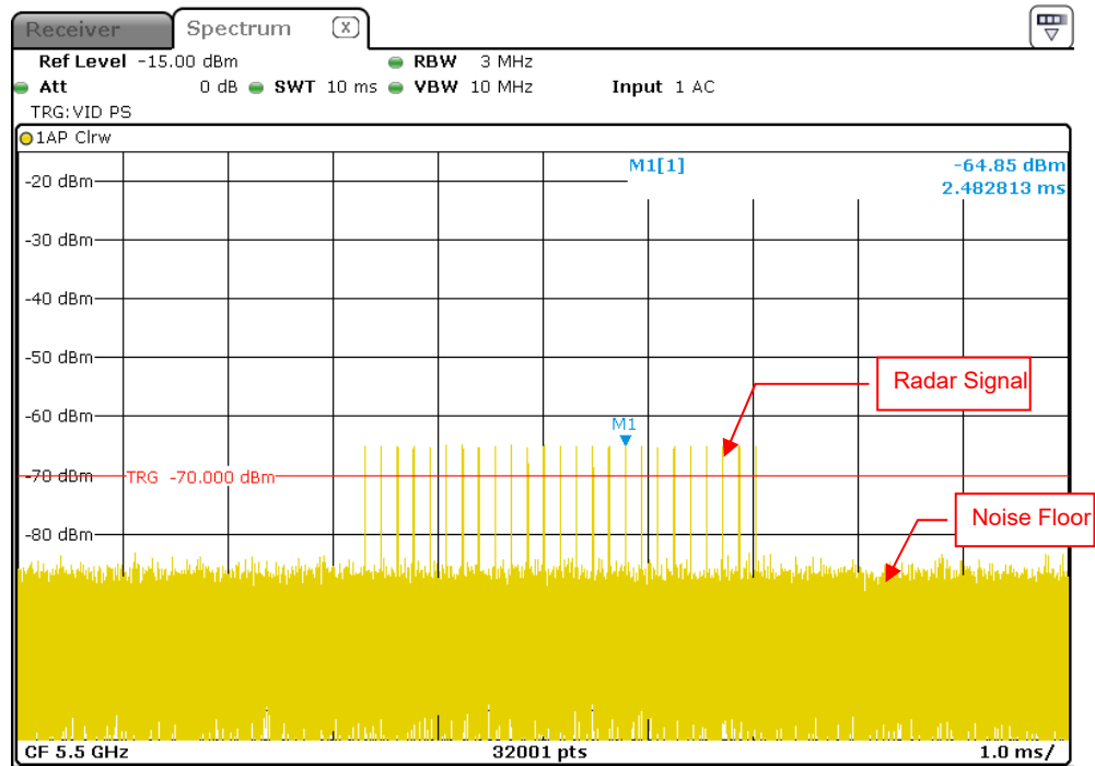
Radar Signal 2
