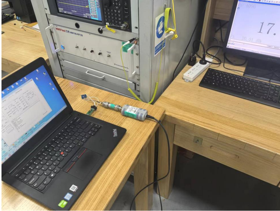
Conducted RF measurement with spectrum analyzer
